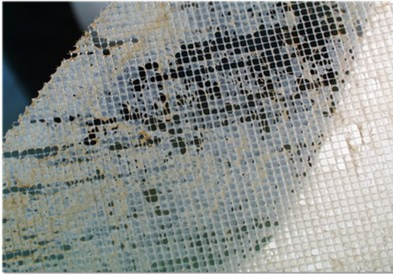
Figure 54. Picture of feed spacer with biofilm
