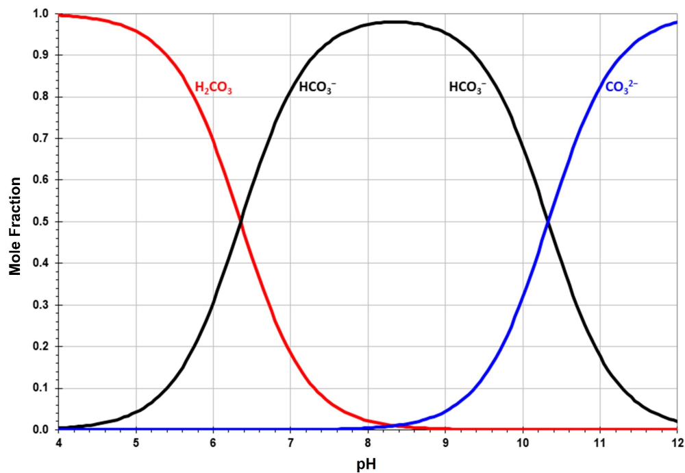
Figure 63. Ionization of carbon dioxide solutions as functions of the pH at 77°F (25°C)
