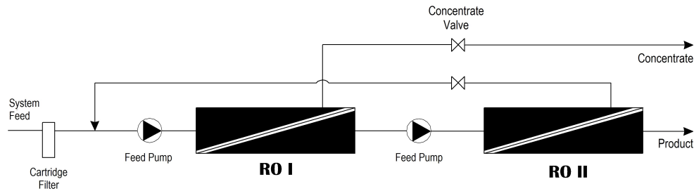
Figure 37. Permeate staged system
