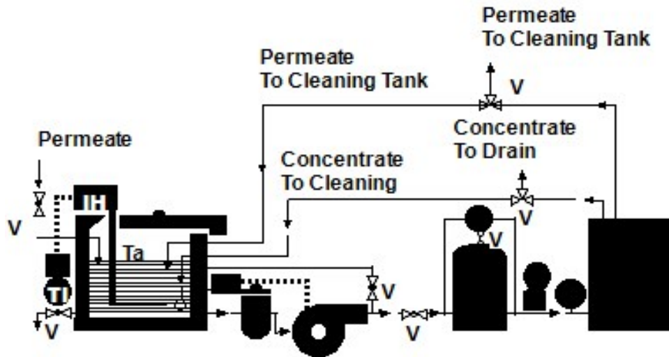
Figure 47. Cleaning system flow diagram
