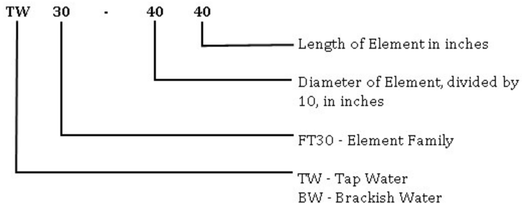
Figure 15. Nomenclature of elements < 8 inches
