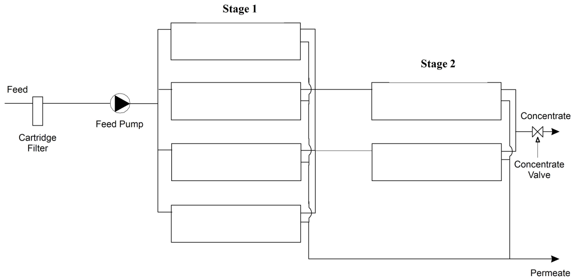
Figure 33. Two-stage system
