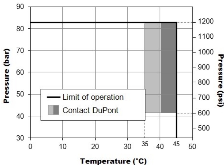
Figure 39. Temperature and Pressure Limits for Elements with iLEC™ Interlocking Endcaps
