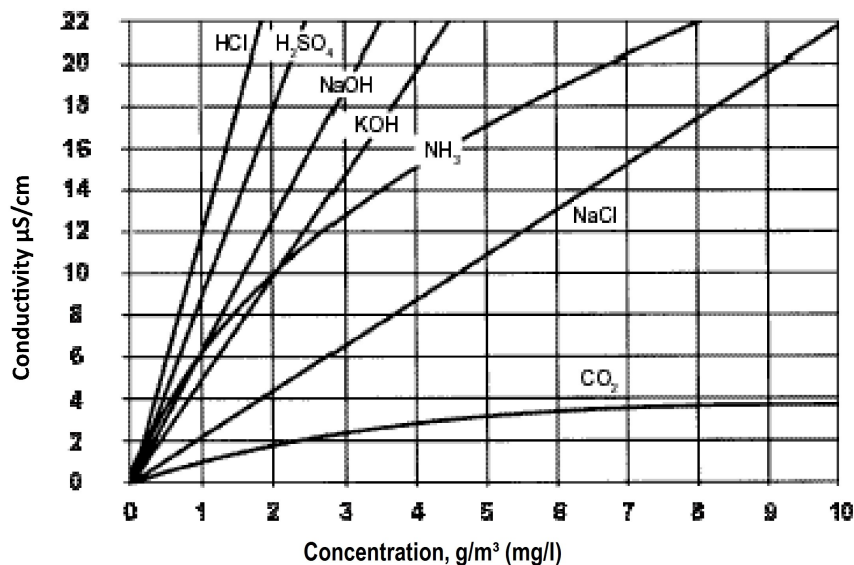
Figure 61. Conductivity of ionic solutions at 77°F (25°C)
