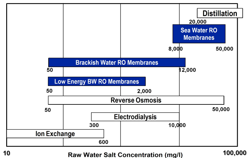
Figure 1. Major desalination processes
