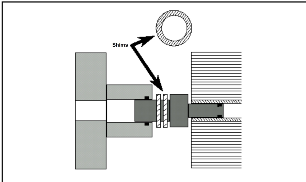
Figure 42. Shim and placement on vessel adapter at feed end of pressure vessel.
