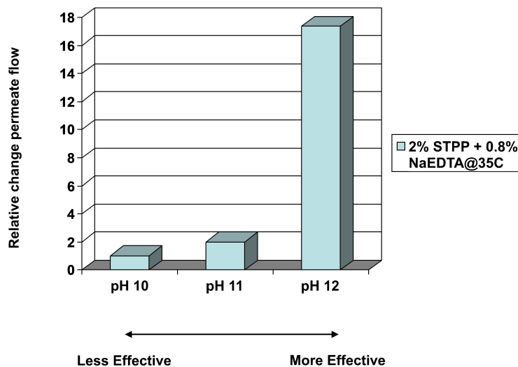
Figure 49. Effect of pH on the removal of biofouling
