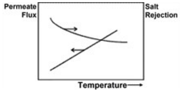
Figure 7. Performance vs. temperature
