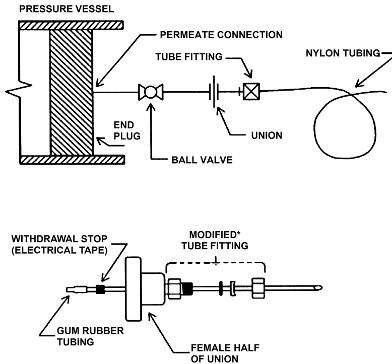
Figure 51. Permeate probing apparatus for spiral-wound membrane
