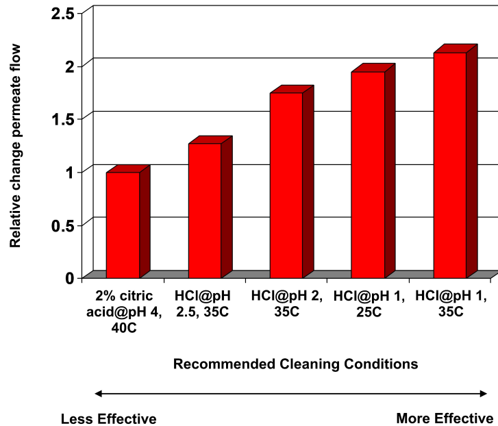
Figure 48. Effect of pH on the removal of calcium carbonate
