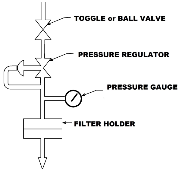
Figure 28. Apparatus for measuring the silt density index
