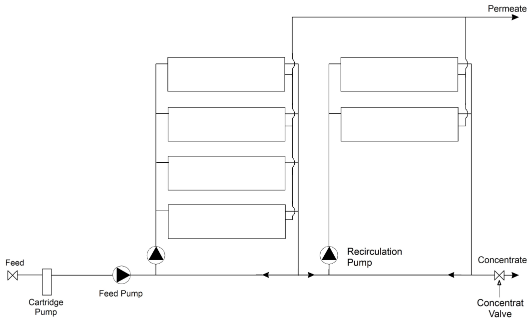
Figure 36. Tapered recirculation system
