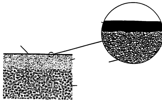
Figure 10. Schematic cross-section of a FilmTec™ thin-film composite membrane
