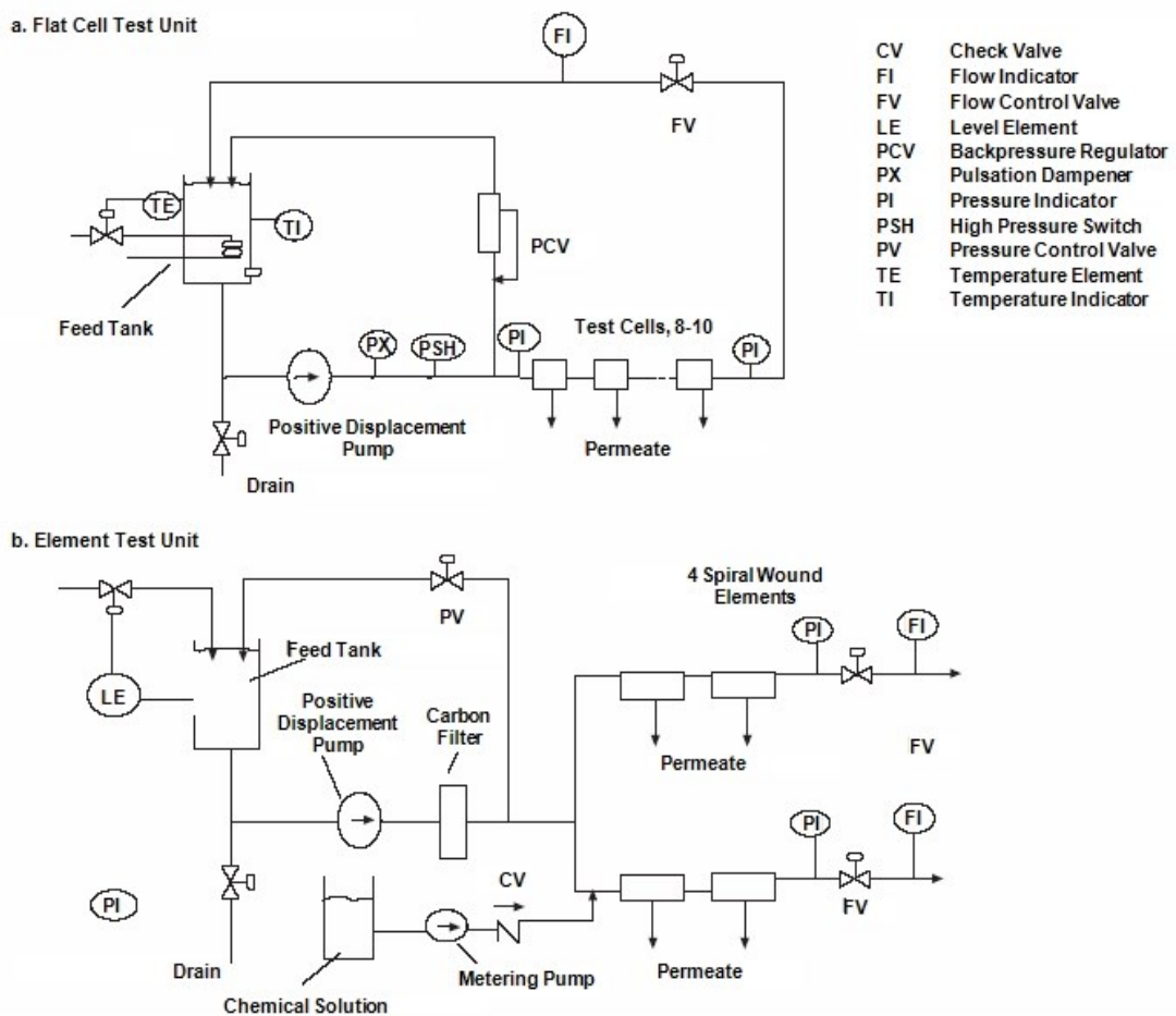
Figure 66. Flow schematic
