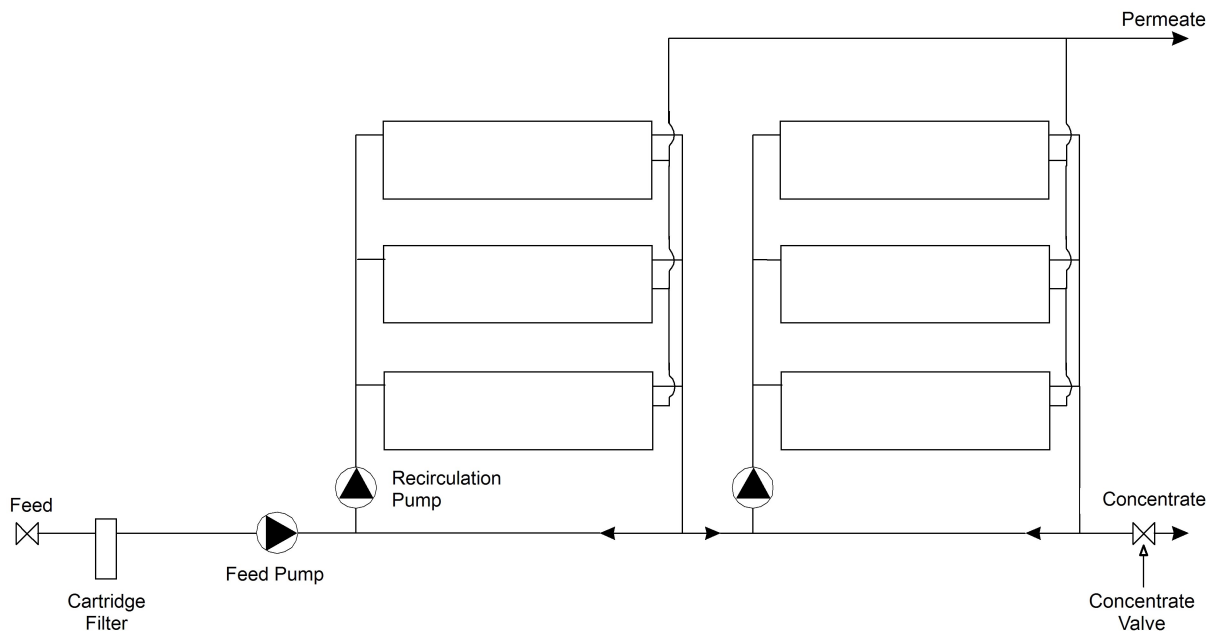
Figure 34. Two-stage system with internal concentrate recirculation
