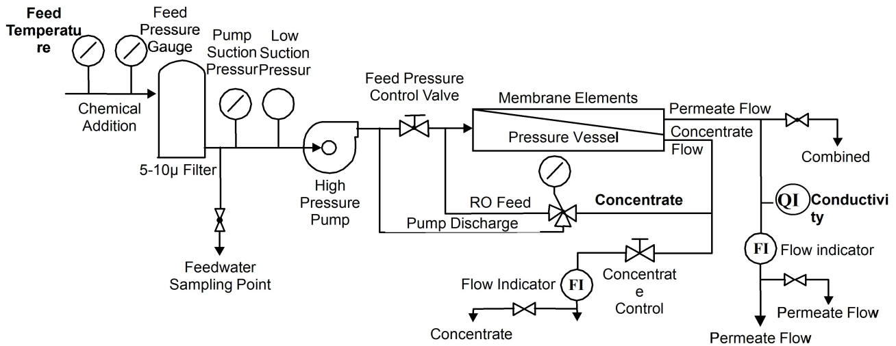
Figure 46. Typical RO/NF system
