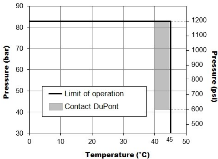
Figure 38. Temperature and Pressure Limits for Elements with Standard Endcaps
