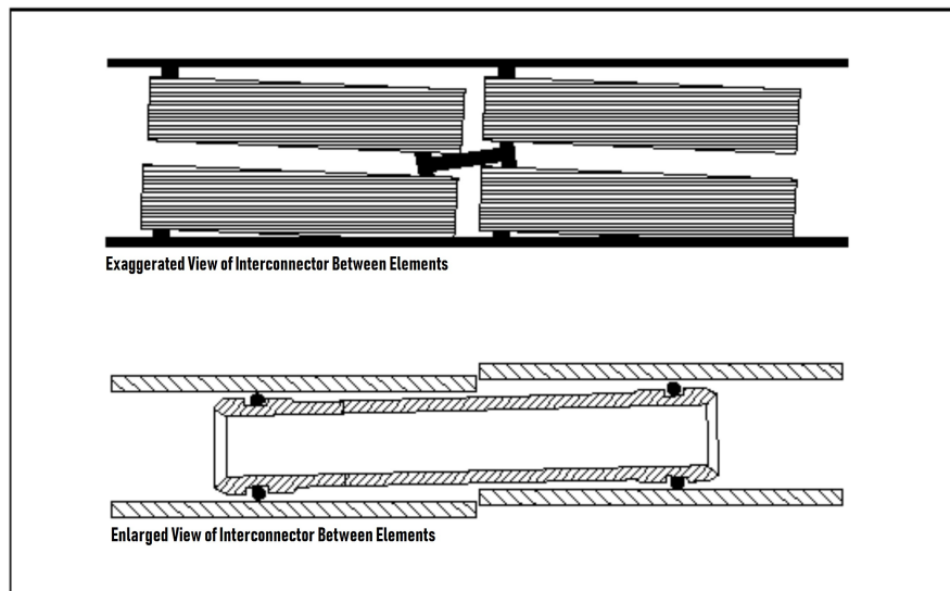
Figure 44. Product water tube misalignment
