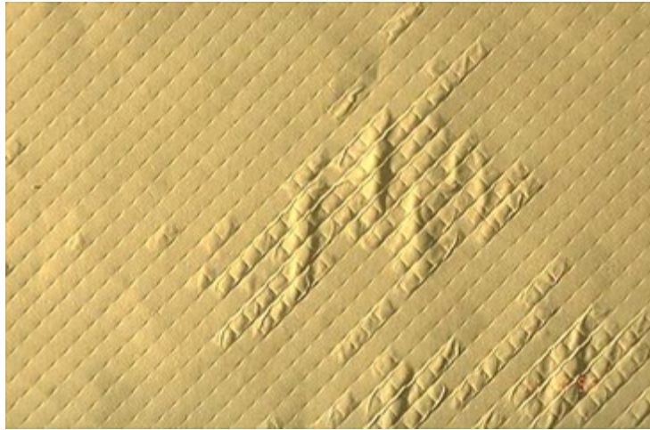
Figure 57. Picture of membrane with permeate backpressure damage
