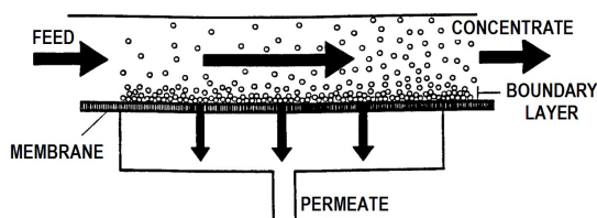
Figure 2. Crossflow membrane filtration
