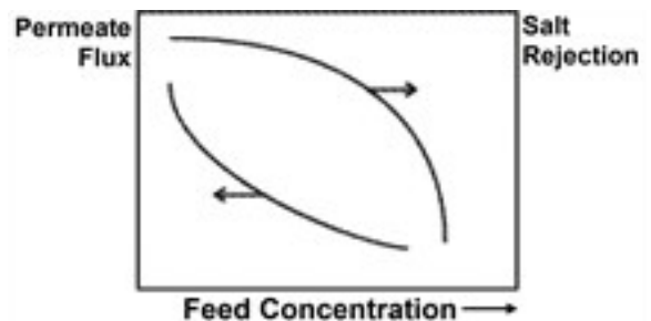
Figure 9. Performance vs. feedwater salt concentration
