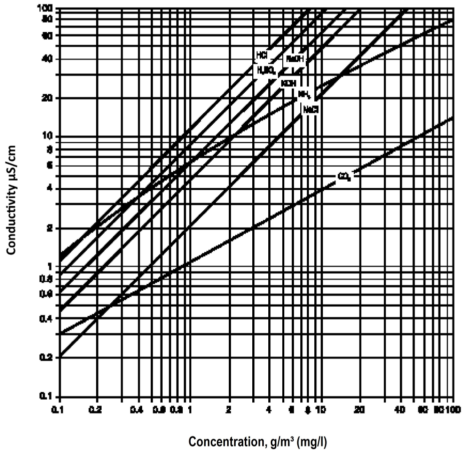
Figure 62. Conductivity of ionic solutions at 77°F (25°C)
