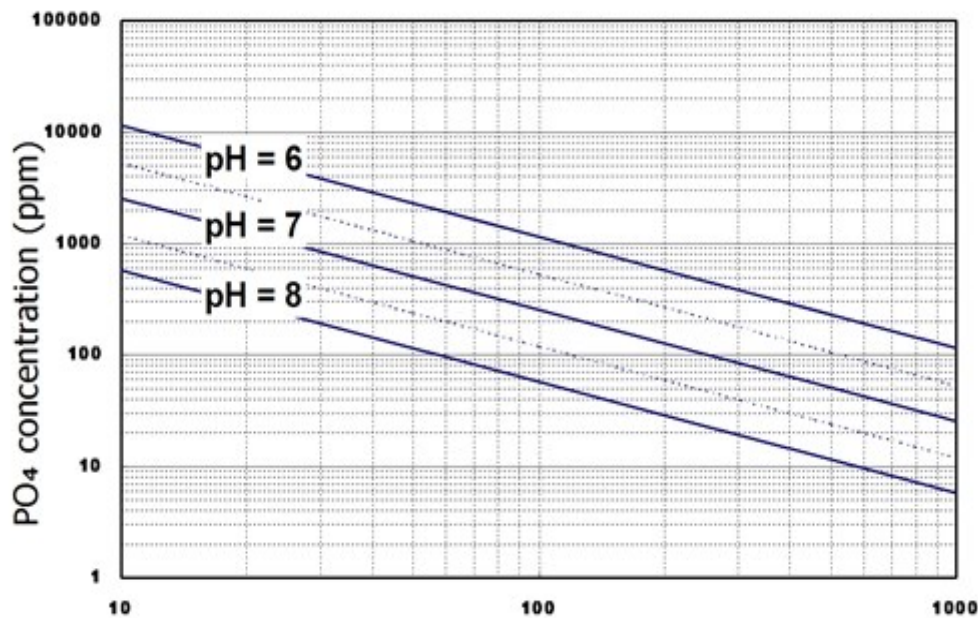
Figure 27. Critical phosphate concentration under various pH at 25°C
