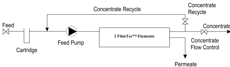
Figure 31. Single-module system
