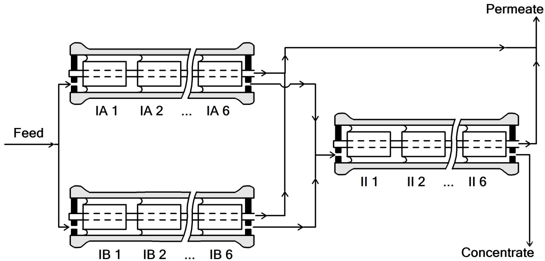
Figure 40. Typical two-stage configuration for spiral-wound RO/NF elements
