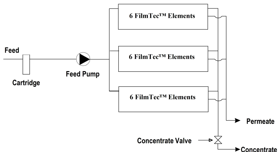
Figure 32. Single-stage system
