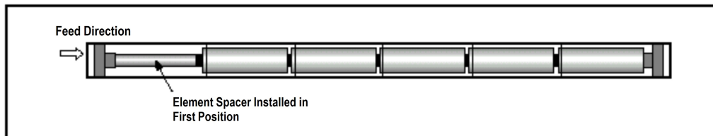
Figure 45. Element spacer properly installed in a pressure vessel
