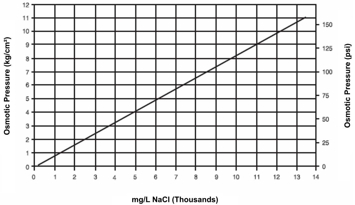
Figure 64. Osmotic pressure of sodium chloride
