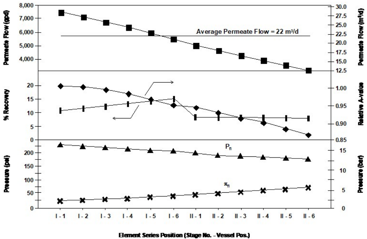
Figure 41. Individual element performance in a system 2:1 array of 8-inch BW30 elements (example)
