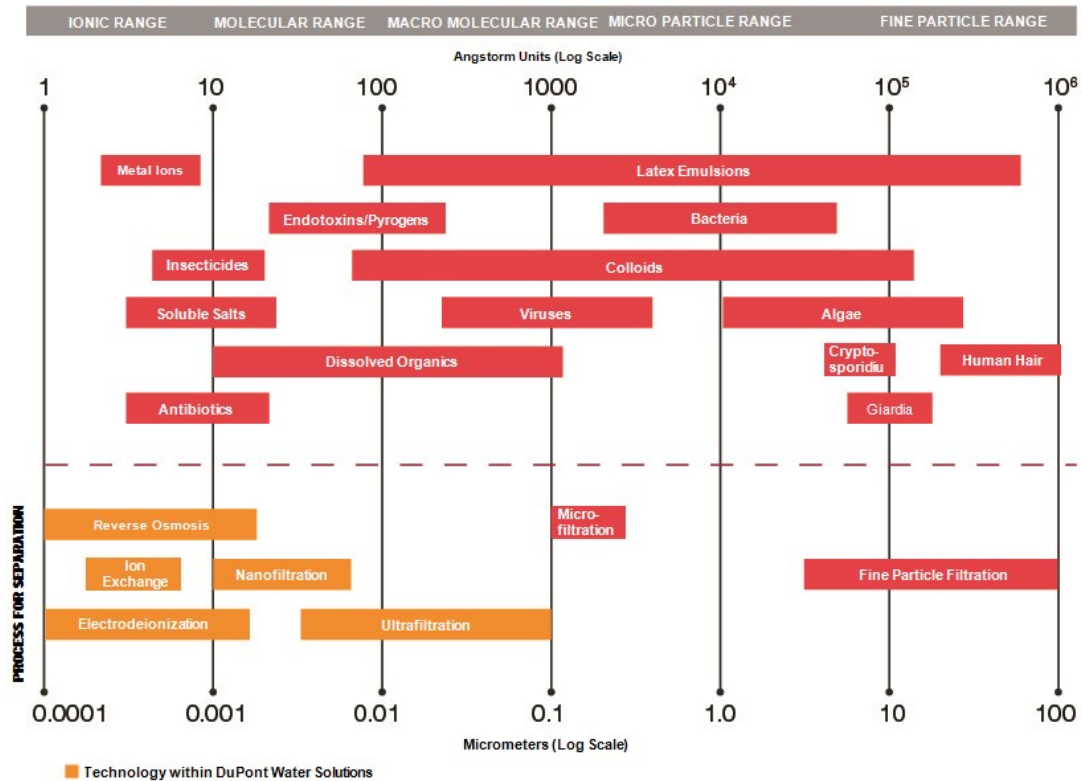
Figure 3. Ranges of filtration processes
