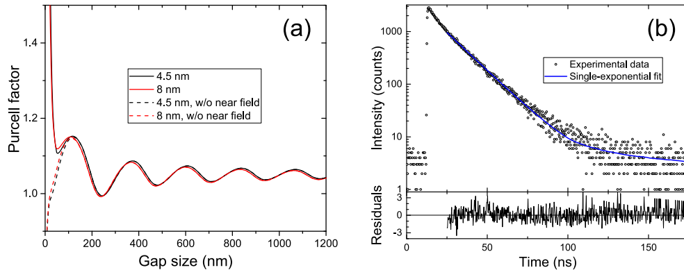
Fig. 4. (a) Purcell factor calculated for an ensemble of 4.5- and 8-nm-deep implanted NV defects in bulk diamond. (b) An example of lifetime histogram with the best fit curve and normalized fitting residuals.
