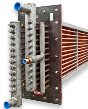
Bare Tubes & Compressed Air Purge Section for Industrial Product Driers
