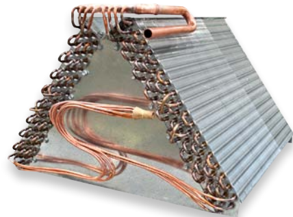
5mm A-Frame Built for Military Comfort HVAC
