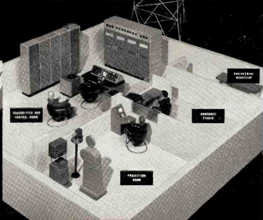
2 kw VHF (ERP range, 2 to 20 kw) Similar to 500-watt plant, but uses an RCA 2-kw transmitter. The ideal set-up for getting up to 20 kw (ERP) for a small investment. "In line" racks at left of control console are: monitoring, audio, and video equipments, sync generator, and power supplies.
