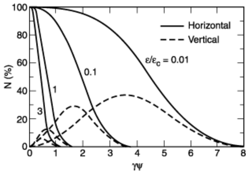
Fig. 2-2. Normalized intensities of horizontal and vertical polarization components, as functions of the vertical observation angle \gamma\Psi , for different photon energies. (Adapted from Ref. 1.)
