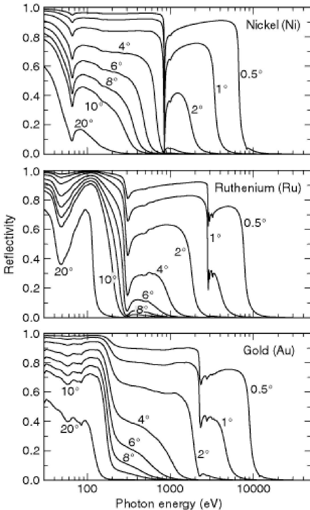
Fig. 4-5. Specular reflectivities of nickel ( \rho = 8.90 \text{ g/cm}^3 ), ruthenium ( \rho = 12.41 \text{ g/cm}^3 ), and gold ( \rho = 19.30 \text{ g/cm}^3 ) as a function of photon energy and grazing angle.
