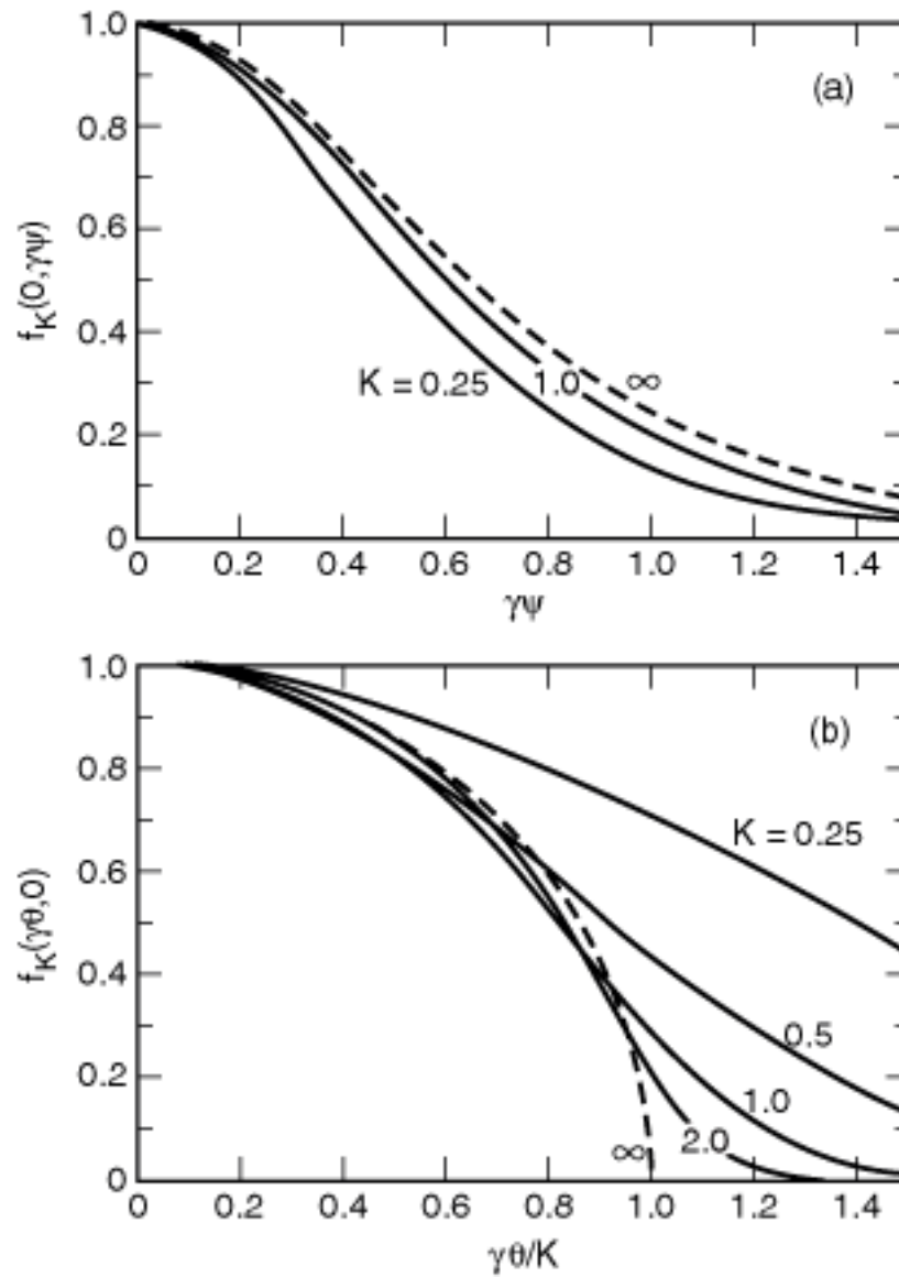
Fig. 2-7. The angular function f_K , for different values of the deflection parameter K , (a) as a function of the vertical observation angle \gamma\psi when the horizontal observation angle \gamma\theta = 0 and (b) as a function of \gamma\theta/K when \gamma\psi = 0 .
