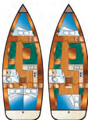
Three Stateroom Version
