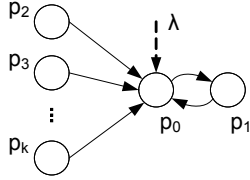
Figure 3: Another optimal structure for a single spam farm with one target page.
