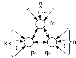
Figure 8: Three spam farms with target pages forming a complete core.
