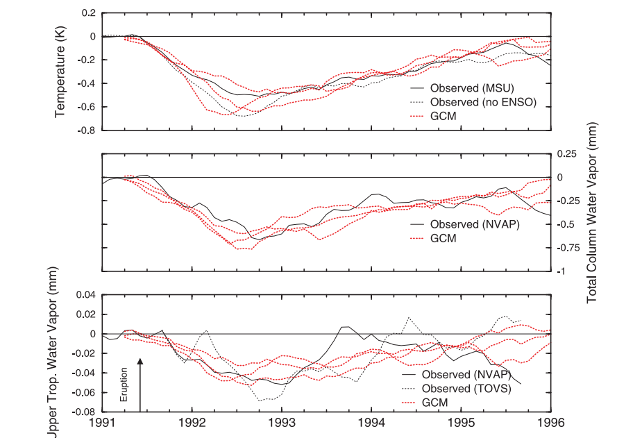
Fig. 2. Comparison of the observed (solid line) and model-predicted (dashed line) global-mean (90°N–90°S) changes in lower tropospheric temperature (top), total column water vapor (middle), and upper tropospheric (300 to 500 hPa) water vapor (bottom) after the eruption of Mount Pinatubo. The observed anomalies are computed using a 1979 to 1990 base climatology and expressed relative to the pre-eruption value, defined here as the mean anomaly for January 1991 to May 1991. The model anomalies are computed for each ensemble pair as the difference between the control and Mount Pinatubo experiments. All time series have been smoothed using a 7-month running mean.
