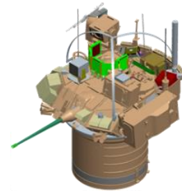
Figure C-3. Manned turret
