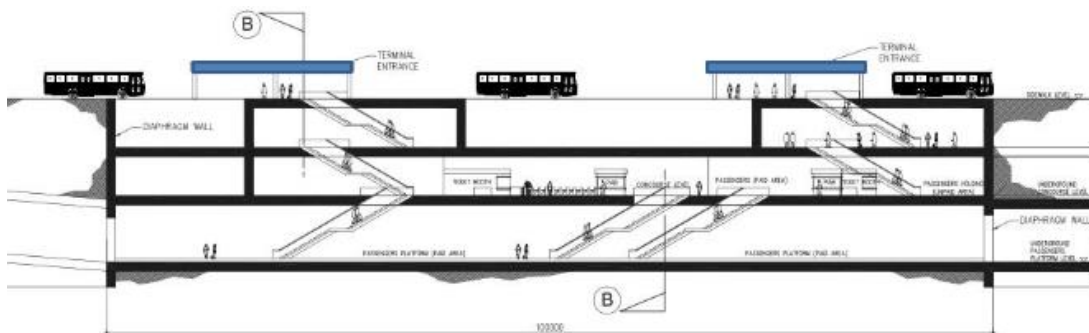
Figure 4.12 Transverse Section of Station (Subway)
