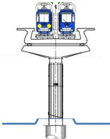
Figure 4.3 Elevated Track System
