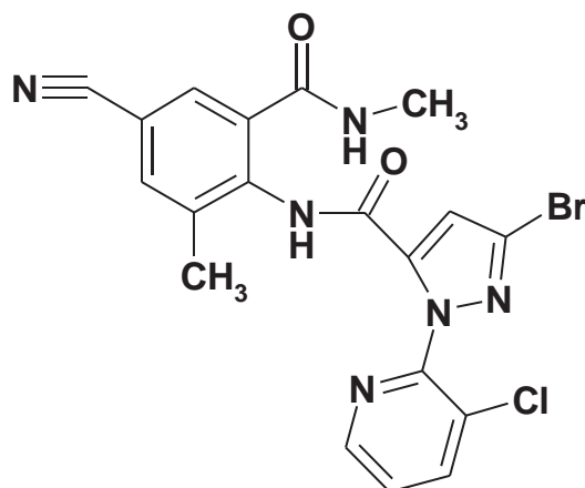
Cyantraniliprole (DPX-HGW86) (MW 473.7)
