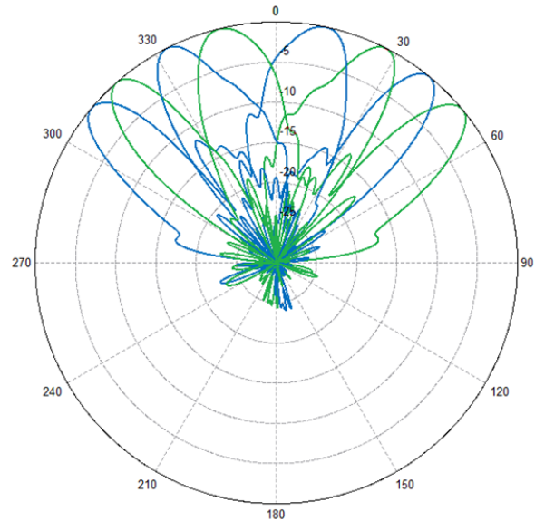
(a) Horizontal Radiation Pattern
