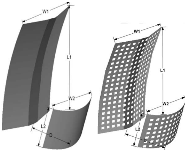
(a) Solid reflectors without punching (b) Punched reflectors
