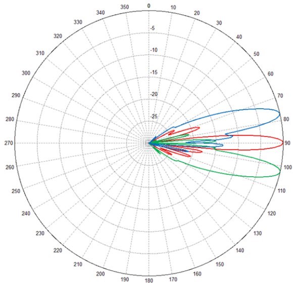
(b) Vertical patterns of three vertical groups of horizontally sectorized beams
