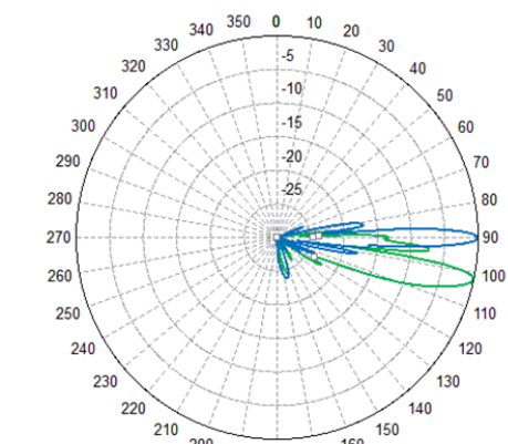
(b) Vertical Radiation Pattern
