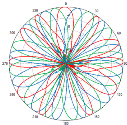
Fig. 11 Horizontal pattern of a configuration for switched beam smart antennas at 1.8 GHz
