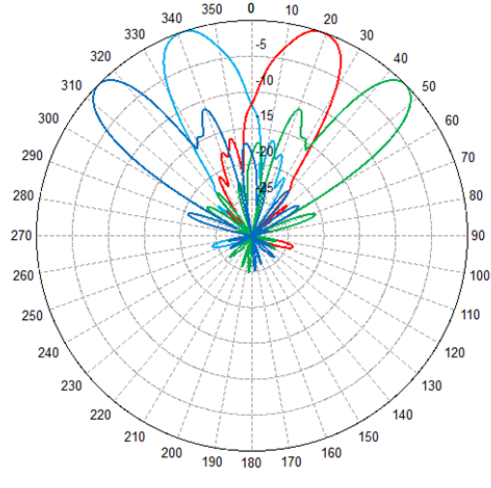
(a) Horizontal Radiation Pattern
