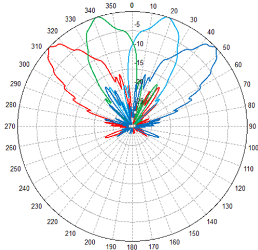
Fig. 6 Radiation patterns of a quad beam antenna with an increased intersection between the beams at 1.8GHz
