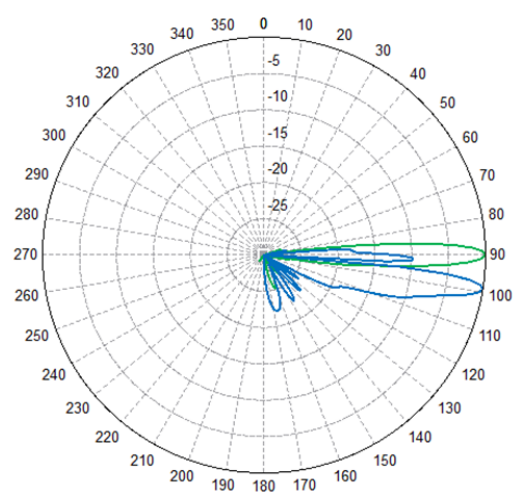
(b) Vertical Radiation Pattern
