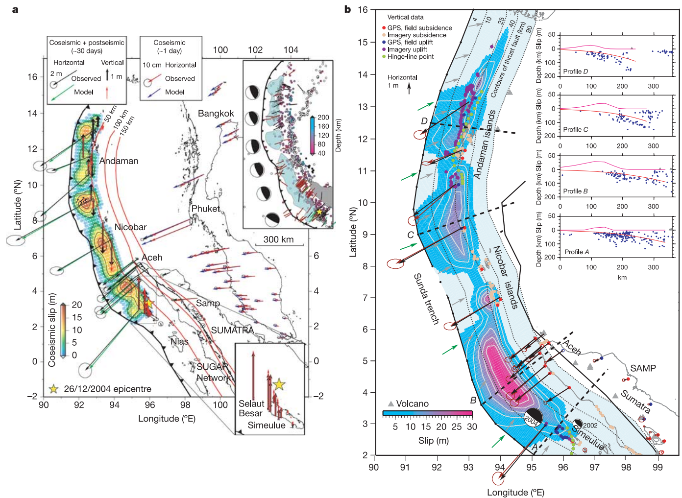
Figure 3 | Fault slip distribution determined from the geodetic data. a , Model A. The distribution of combined coseismic and one-month postseismic slip on the Sunda megathrust estimated from inversion of geodetic data shown in Fig. 2, including 30-day estimates of displacements from the permanent GPS stations at Medan (SAMP) and Phuket (PHKT) 17 . Black contour lines of slip are at 5-m intervals. Displacements computed from this model (green arrows for the horizontal and red arrows for the vertical at the sites used in the inversion, blue arrows at the other sites) are compared with the survey-mode observations and with displacements over the first day estimated at continuous GPS stations in Thailand and Malaysia 17 (red arrows). Displacements are shown with 95% confidence ellipses. The comparison shows that significant postseismic displacements occurred in the first month following the rupture. The lower inset in a is a close-up view of predicted and measured vertical displacements on Simeulue Island. The upper inset in a shows a comparison of ruptured area (where slip exceeds 5 m in the model) with seismicity before the Sumatra–Andaman earthquake (1964–2002) 44 . ‘Beach ball’ symbols show local mechanisms determined
