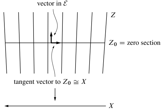
Figure 6.2 The tangent bundle to Z restricted to Z_0 \cong X is \mathcal{T}_X \oplus \mathcal{E} .
