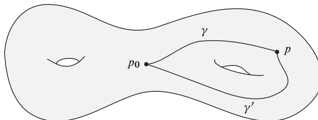
Figure D.4 The integral \int_{p_0}^p \omega may depend on the choice of path.
