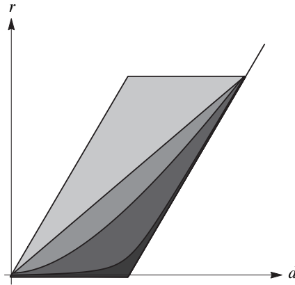
Figure D.5 The shaded regions correspond to points (d, r) such that there exists: ■ a complete linear series whose existence is not contradicted by the Riemann–Roch theorem; ■ a complete linear series that actually exists on some curve of genus 100; ■ a complete linear series on some curve of genus 100, which defines a birational map; and ■ a complete linear series on a general curve of genus 100 (this necessarily defines a birational map when r > 1 ).
