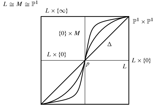
Figure 2.4 [\Delta][L \times \{0\}] = 1 = [\Delta][\{0\} \times M] , so [\Delta] = [\{0\} \times M] + [L \times \{0\}] , as one also sees from the degeneration in the figure.
