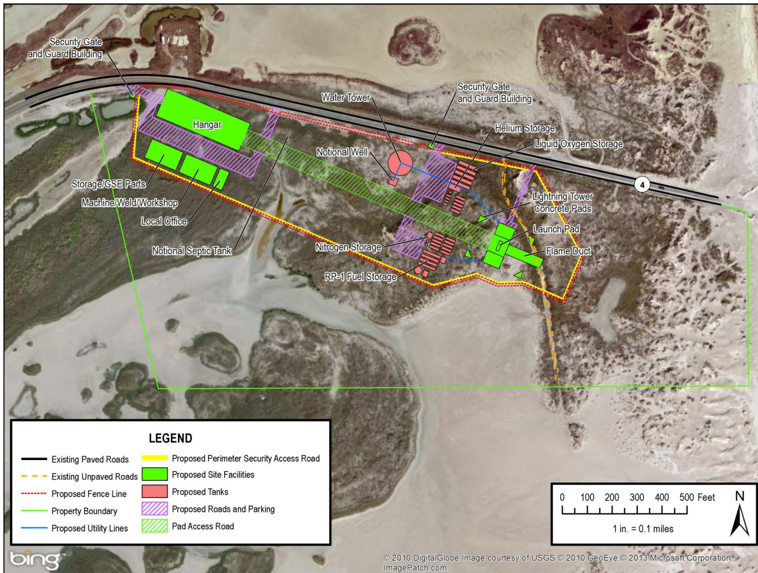
Figure 3. Proposed Vertical Launch Area Site Layout
