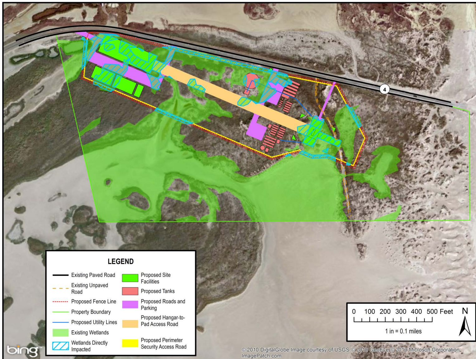
Figure 5. Vertical Launch Area Wetland Impacts
