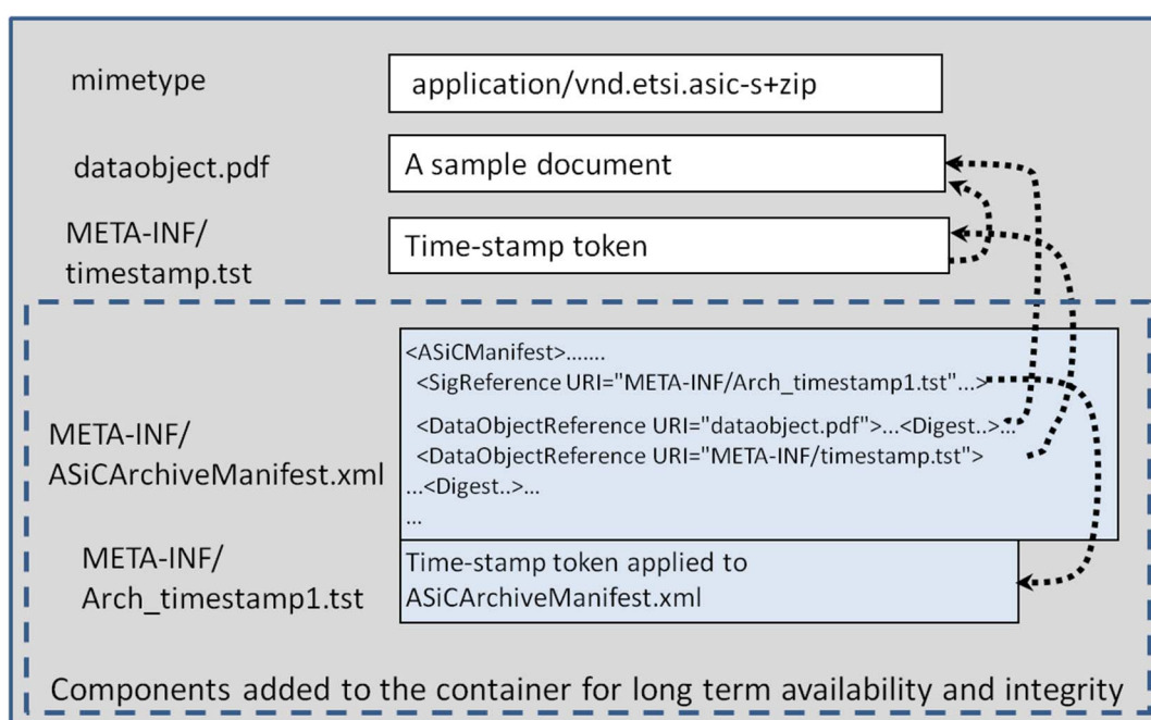
Figure 3: ASiC-S with time-stamp token and long term components (example)
