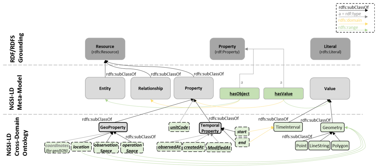
Figure 10: Minimal cross-domain ontology used in NGS-LD API
