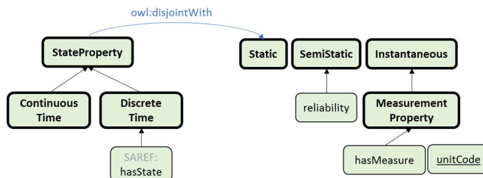
Figure 13: Cross-Domain Properties
