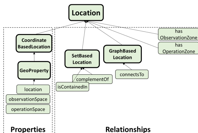
Figure 14: Cross-Domain Location
