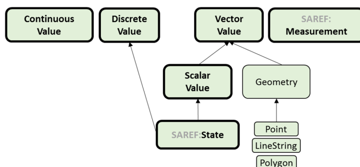
Figure 15: Cross-Domain Values
