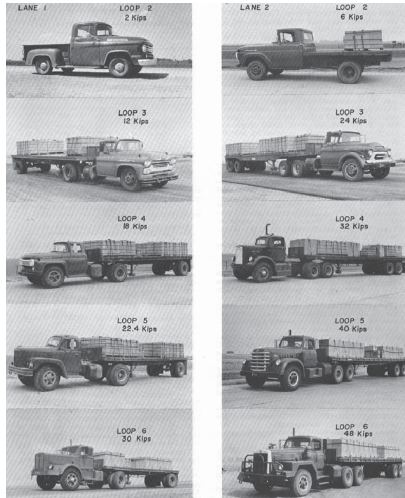
FIGURE 3 AASHO Road Test truck traffic.
