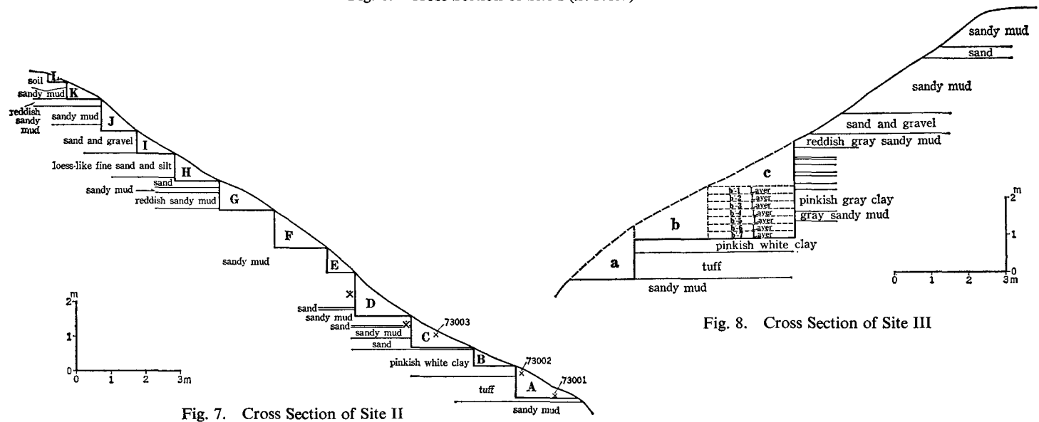
Fig. 7. Cross Section of Site II
