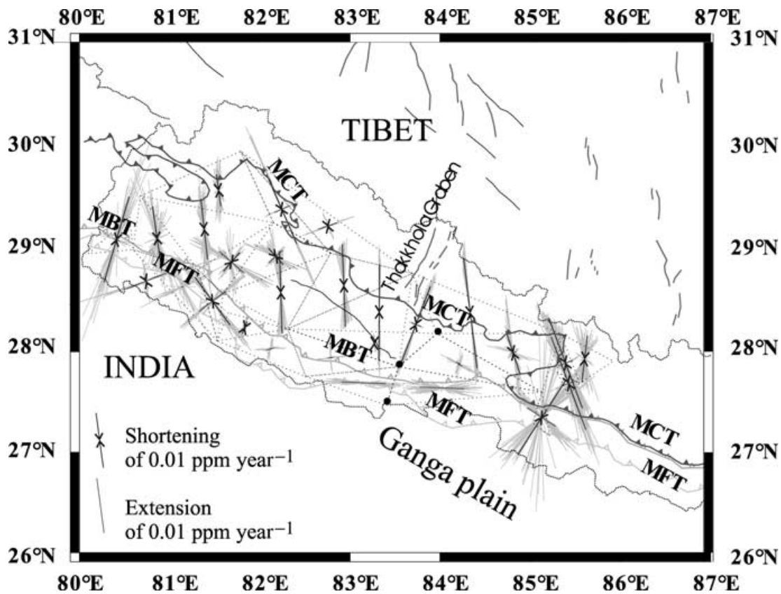
Figure 8. Strain-rate tensors computed from the velocity field. Tensors characterized by their eigenvalues and eigenvectors are drawn at the barycenter of triangles used for their computations. Errors in strain rates for a 95 per cent confidence level have been obtained using a Monte Carlo simulation of errors. Perturbed tensors simulating the errors for a 95 per cent confidence level, are drawn as grey bars around the unperturbed solutions. Strain-rate tensors show an area undergoing most of the current deformation that is surrounded to the north by the Higher Himalayas–southern Tibet area with an E–W extension, and to the south by the outer belt of the Himalayas affected by a nearly negligible present-day deformation. A spatial variation in the orientation of the shortening-axis between western and central Nepal, east of the 83°E meridian, illustrates the segmentation of the present-day deformation of Himalayas probably related to a segmentation of the MHT.
