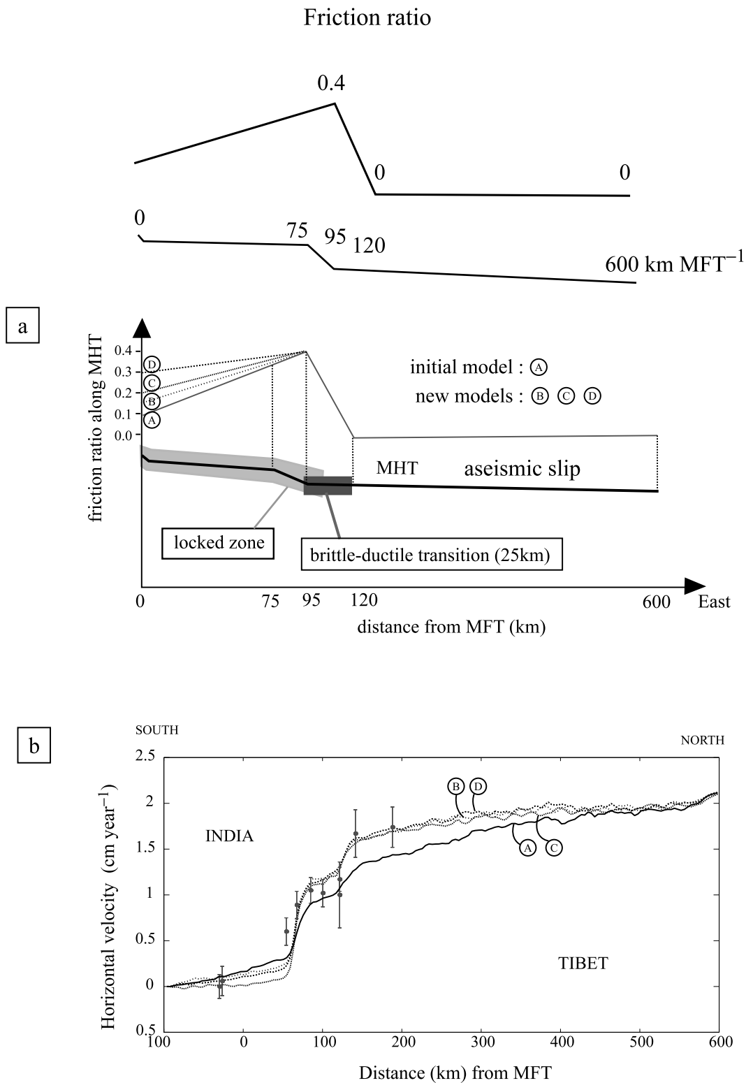
Figure 6. (a) MHT friction ratios for each model accordingly with the distance from the MFT. (b) Calculated (lines) and measured (full circle) interseismic velocities. Measured velocities come from GPS measurements of Wang et al. (2001) expressed in the India fixed reference frame with 95 per cent confidence error bars.
