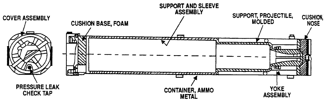
Figure 3-29. Metal Container for Cartridge, 120mm: HEAT-MP-T, M830A1 and HE-OR-T, M908.
