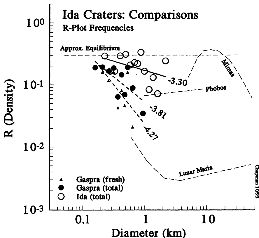
Fig. 2. Crater size-frequency data for Gaspra and Ida, with comparisons. These “R-plot” consists of differential frequency data, normalized by dividing by D^{-3} . Modified from a figure in Chapman et al. (1993).
