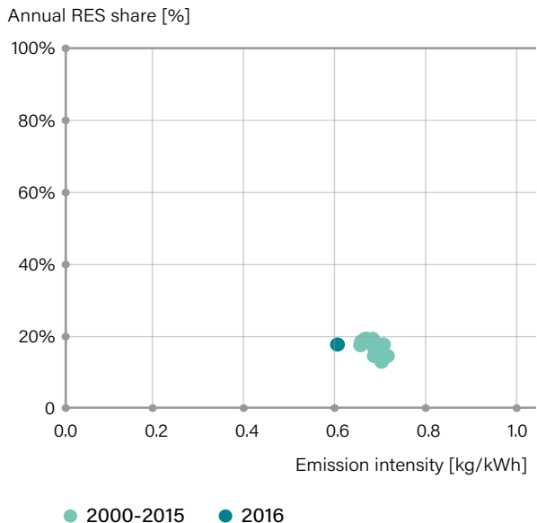
Emission trends in relation to RES shares
