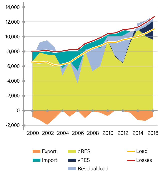
Generation Mix [GWh]
