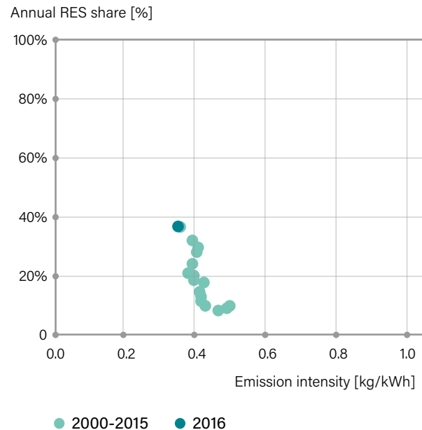
Emission trends in relation to RES shares
