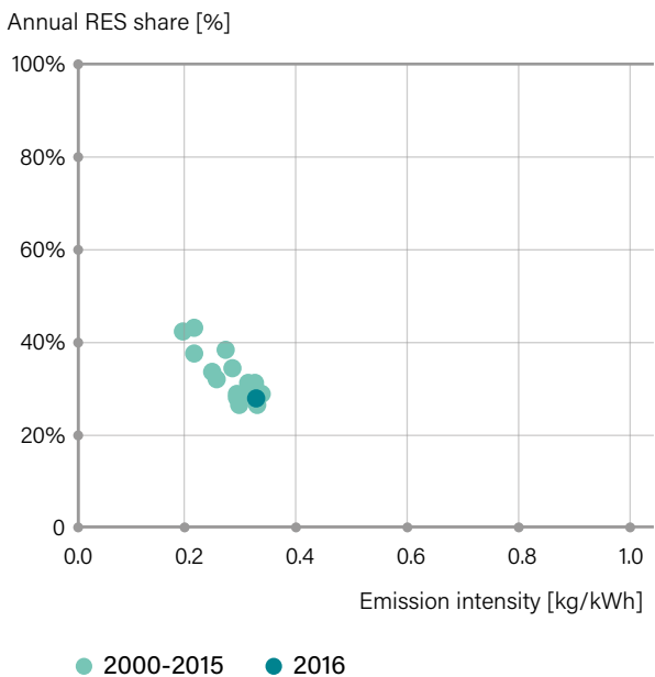
Emission trends in relation to RES shares
