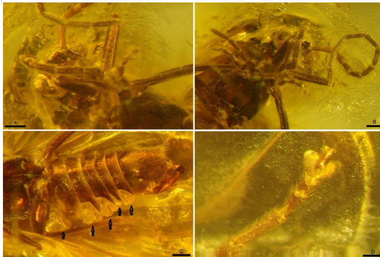
Fig. 16. Mantimalthinus bartholini sp. nov. ALDC0511/ALD.Ba.Can.25 in Baltic amber. A: Holotype, detail of eyes and palpi, bar = 200 µm; B: Holotype, detail of antennae and metasternum, bar = 200 µm; C: Holotype, detail of abdominal segments (arrows show the extruded vesicles), bar = 400 µm; D: Holotype, detail of leg, bar = 100 µm.
