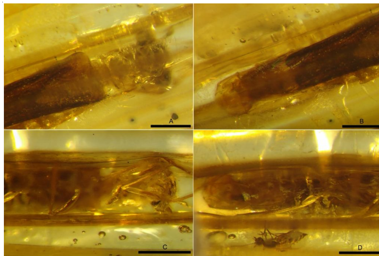
Fig. 14. Sanaungulus troelsikloevedali sp. nov. ALDC0527/ALD.Bu.204 in Burmese amber. A: Holotype, detail of prothorax and elytra, bar = 500 µm; B: Holotype, detail of apex of elytra, bar = 500 µm; C: Holotype, detail of sternum and legs, bar = 1.0 mm; D: Holotype, detail of last ventrites, bar = 500 µm.
