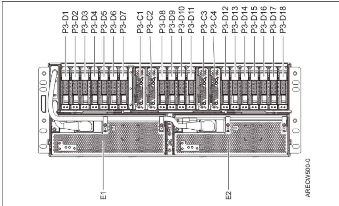
Figure 2-19 5802 I/O drawer front view location codes
