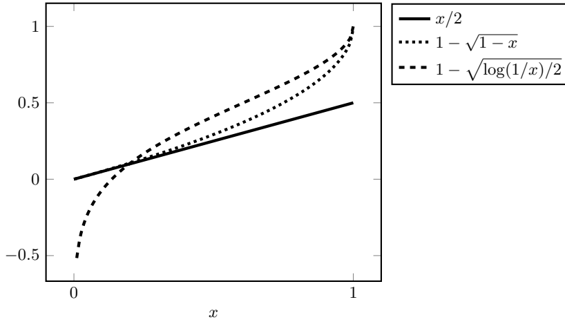
Figure 14.2 Tightening the inequality of Le Cam. Here, x = \exp(-D(P, Q)) . Higher values are better as the figure shows lower bounds on P(A) + Q(A^c) .
