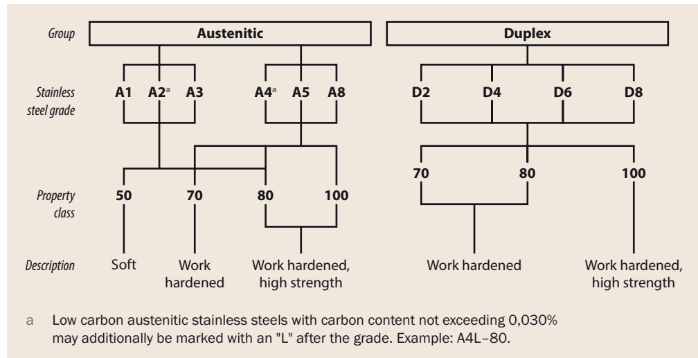
Figure 2.4 Designation system for stainless steel grades and property classes for fasteners
