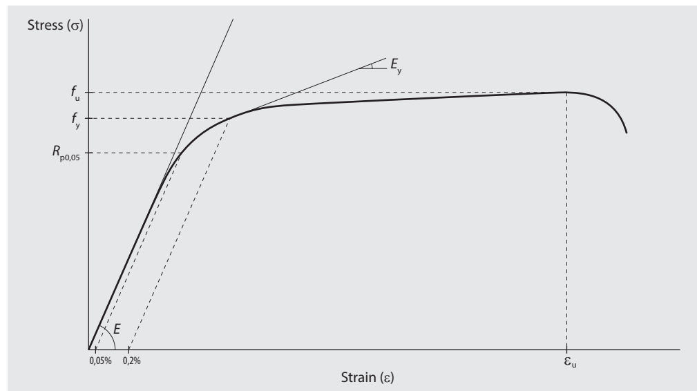
Figure C.1 Key parameters in material model
