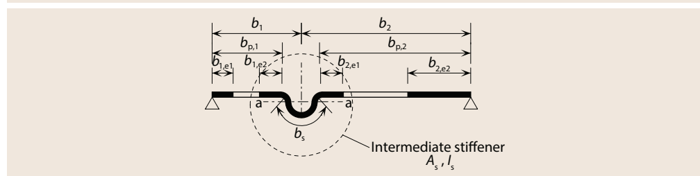
Figure 5.4 Intermediate stiffener
