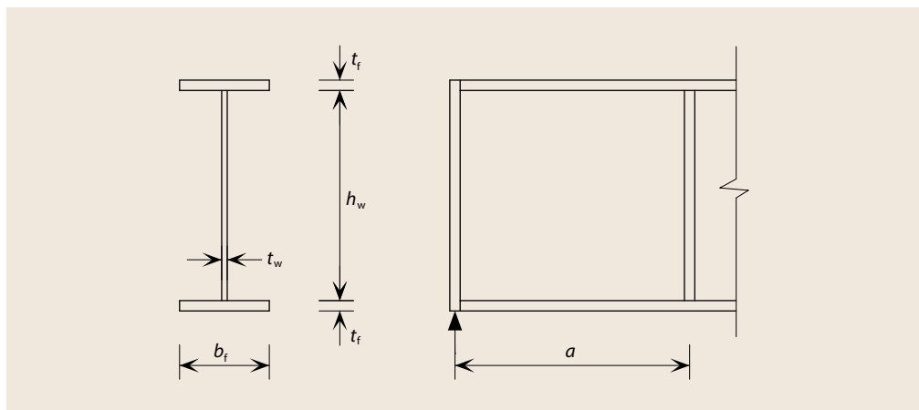
Figure 6.3 Notation for geometrical dimensions
