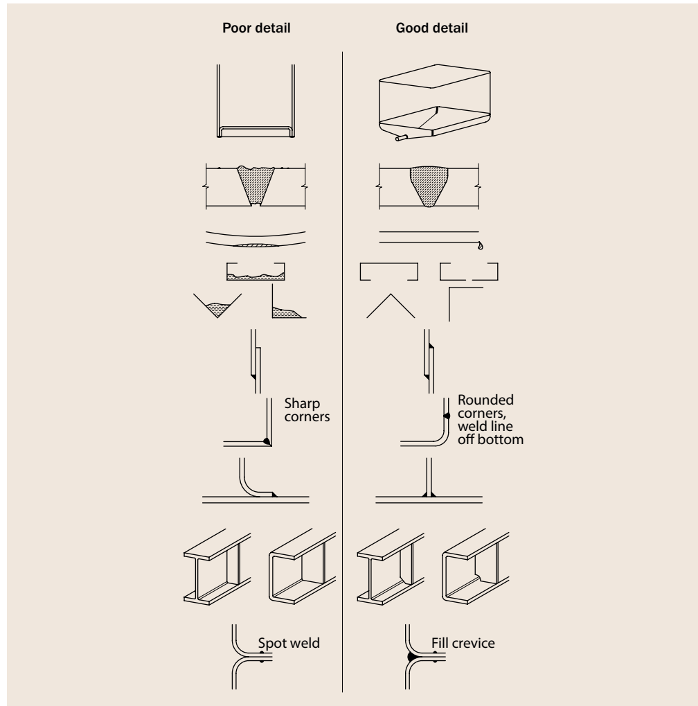
Figure 3.1 Poor and good design features for durability
