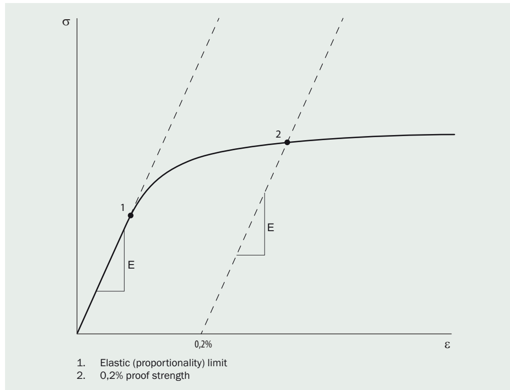
Figure 2.3 Definition of the 0,2% proof strength
