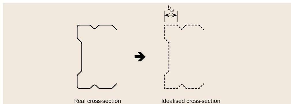
Figure 5.6 Approximate allowance for rounded corners
