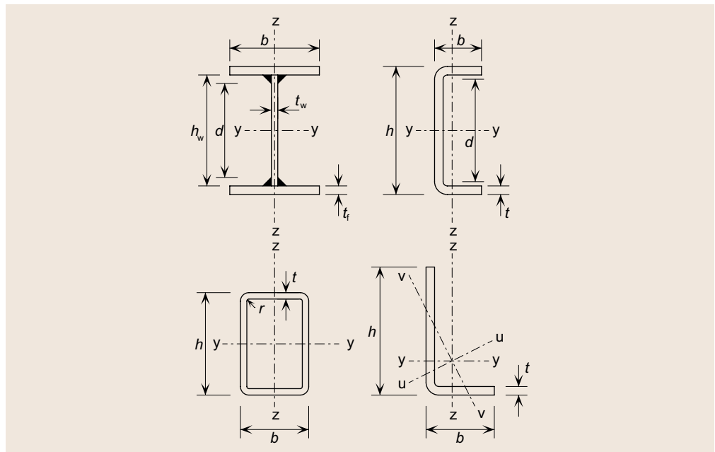
Figure 1.1 Dimensions and axes of sections
