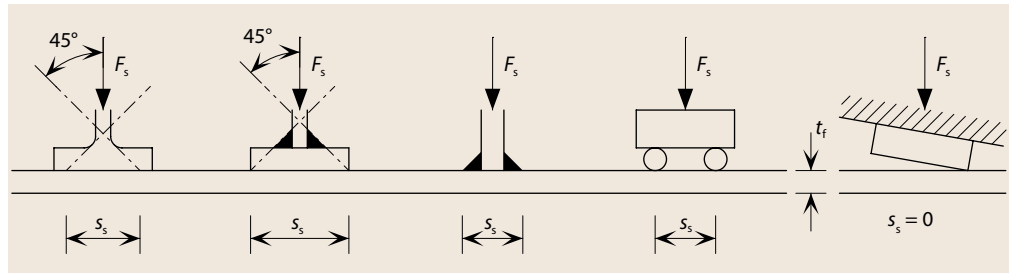
Figure 6.5 Length of stiff bearing
