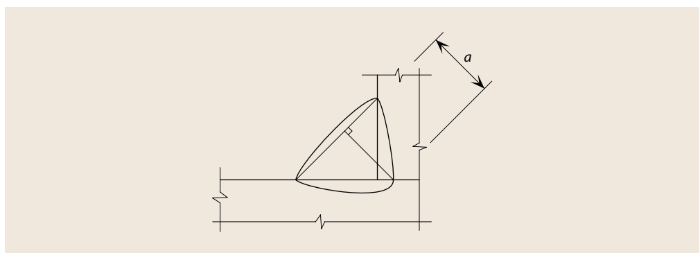
Figure 7.4 Deep penetration fillet weld throat thickness
