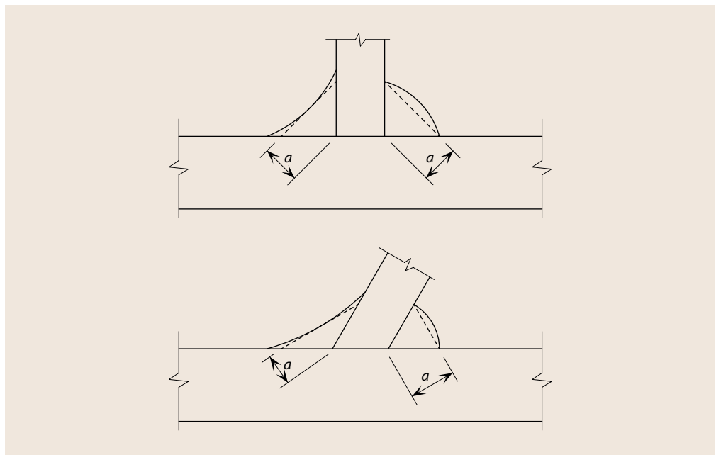
Figure 7.3 Fillet weld throat thickness
