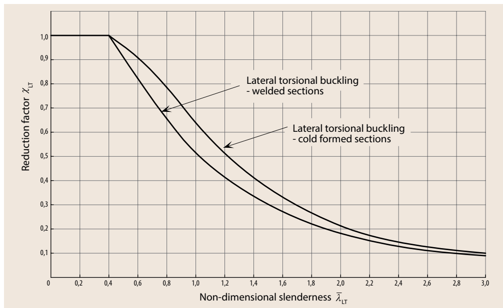
Figure 6.2 Buckling curves for lateral- torsional buckling
