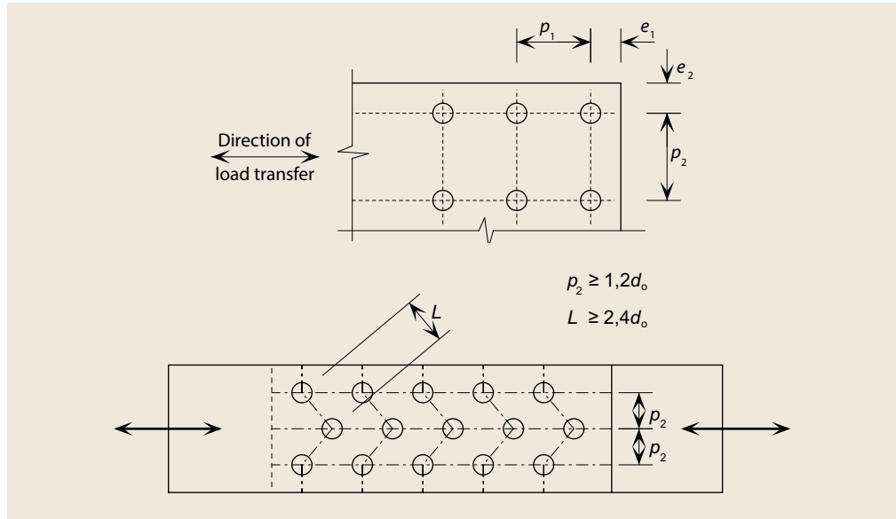
Figure 7.2 Symbols for defining position of holes
