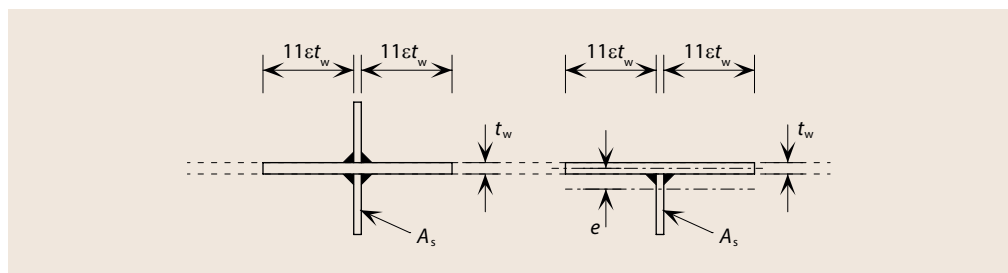
Figure 6.6 Effective cross-section of stiffeners for buckling
