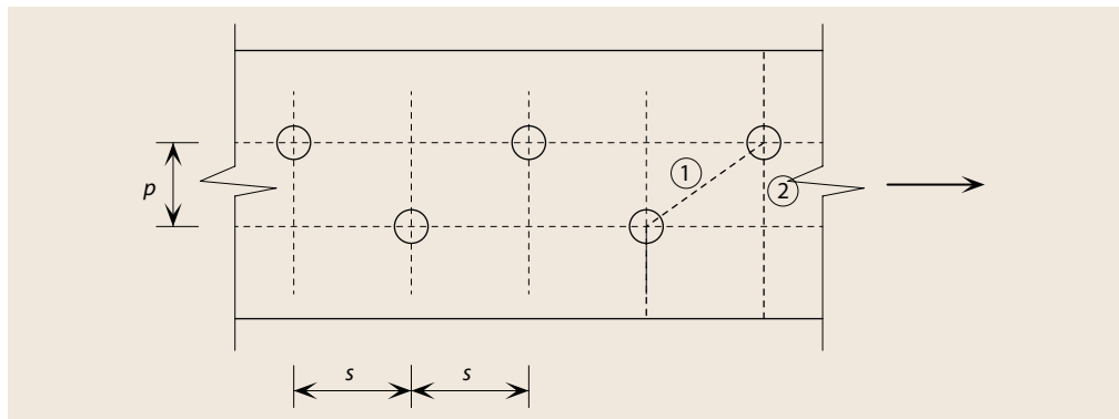
Figure 5.7 Staggered holes and critical fracture lines 1 and 2
