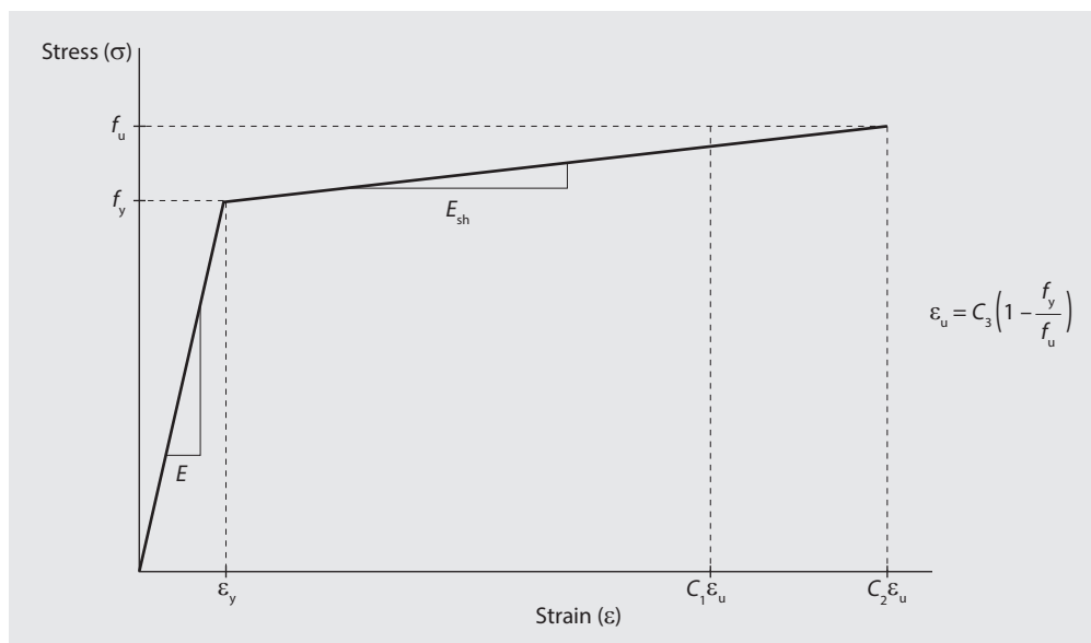
Figure D.1 CSM elastic, linear hardening material model
