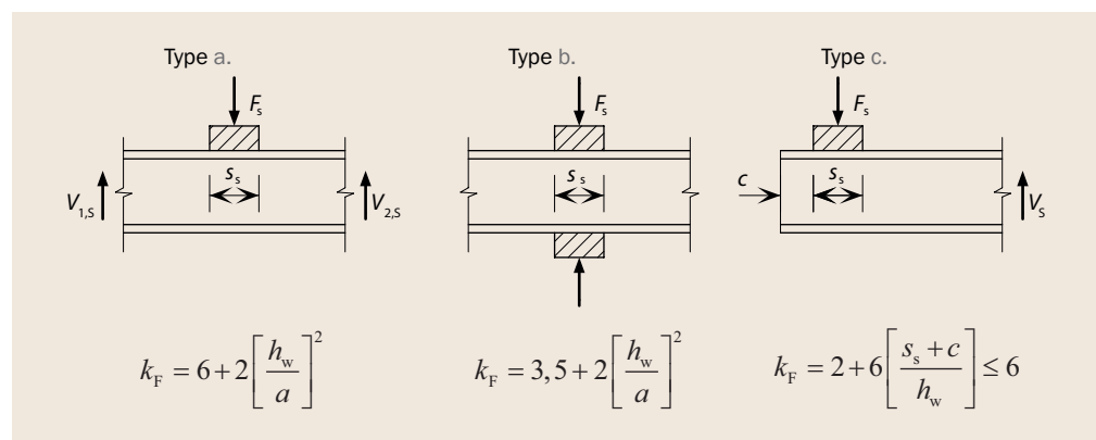
Figure 6.4 Buckling coefficients for different types of load application
