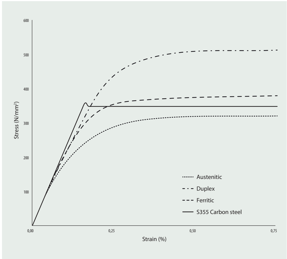
Figure 2.1 Stress-strain curves for stainless steel and carbon steel from 0 to 0,75 % strain
