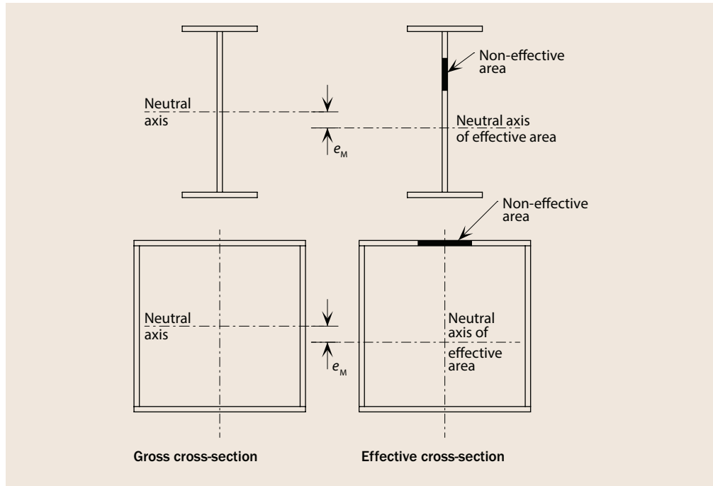
Figure 5.1 Class 4 cross-section subject to bending moment
