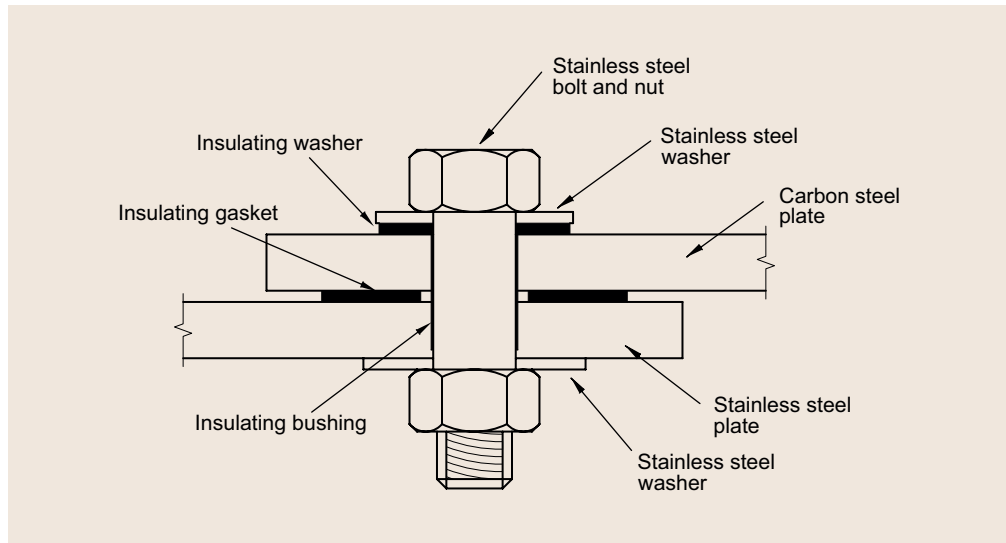
Figure 7.1 Typical detail for connecting dissimilar materials (to avoid bimetallic corrosion)
