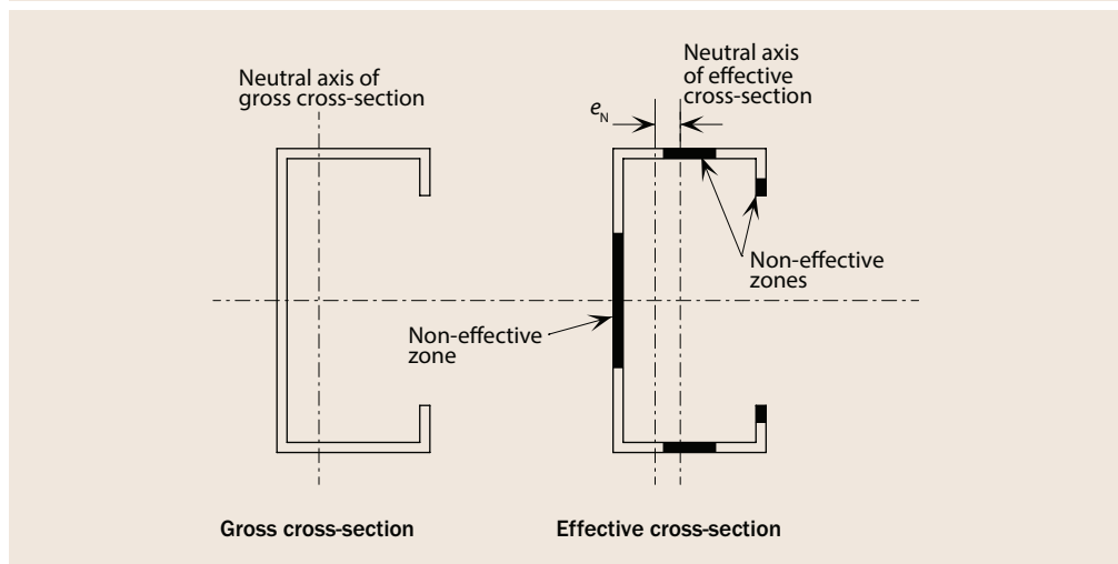
Figure 5.2 Class 4 cross-section subject to compression
