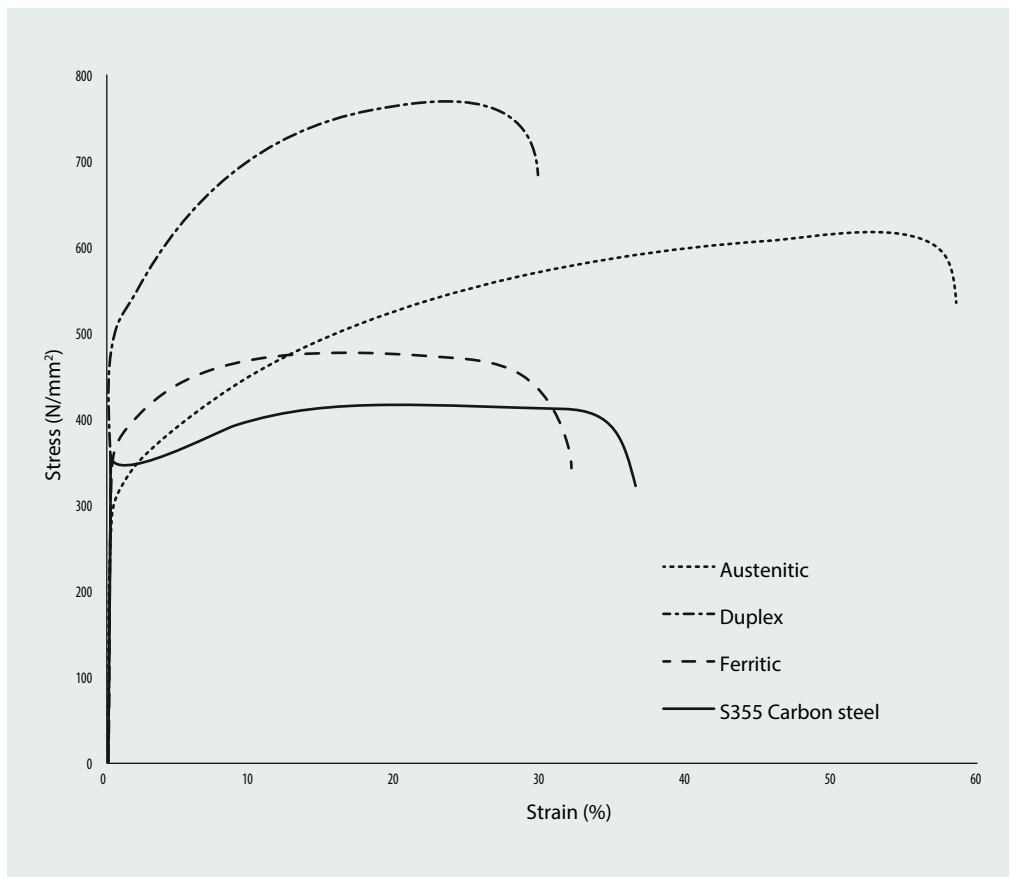
Figure 2.2 Full range stress- strain curves for stainless steel and carbon steel
