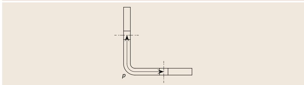
Figure 5.8 Gauge length for angle with holes in both leg
