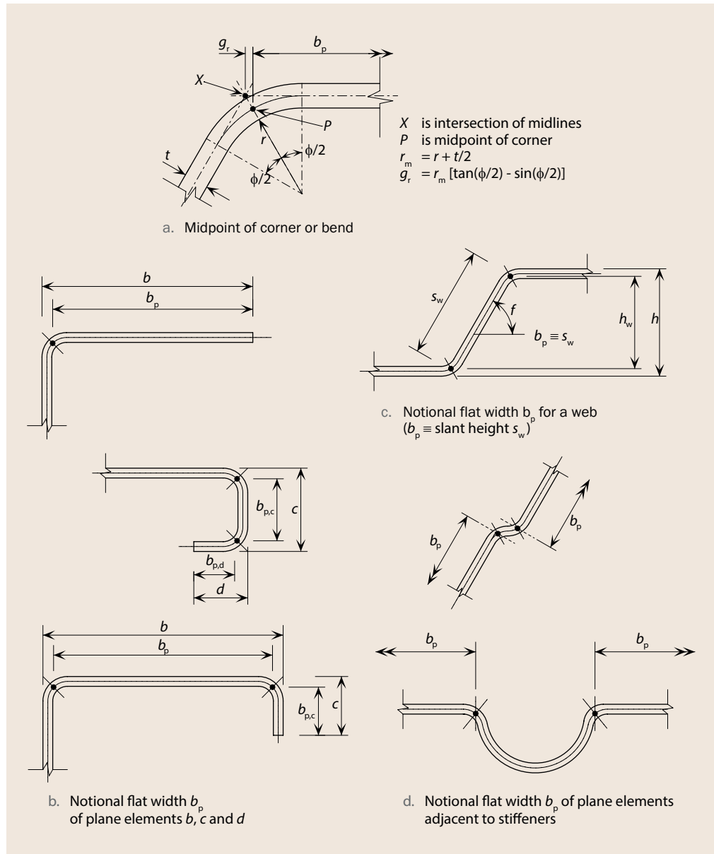
Figure 5.5 Notional widths of plane elements b_p allowing for corner radii
