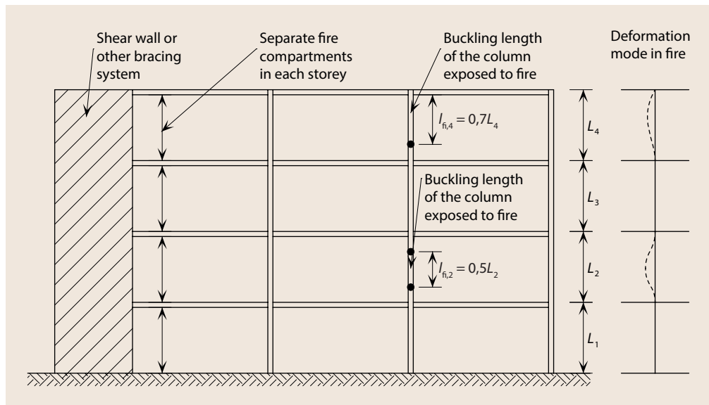
Figure 8.1 Buckling lengths l_{fi} of columns in braced frames
