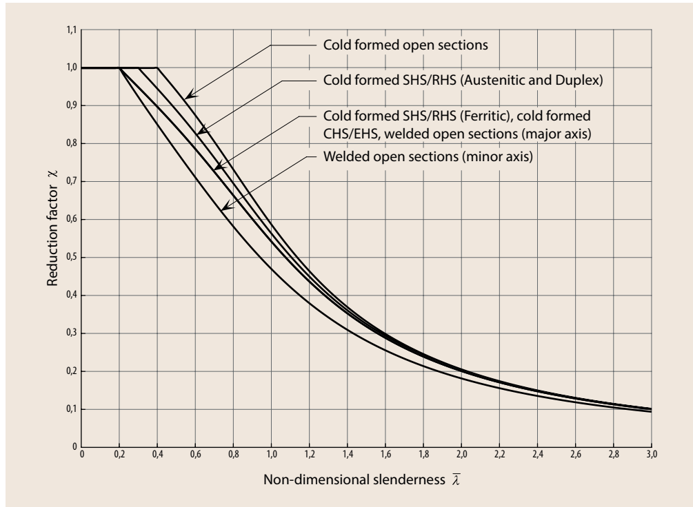
Figure 6.1 Buckling curves for flexural buckling
