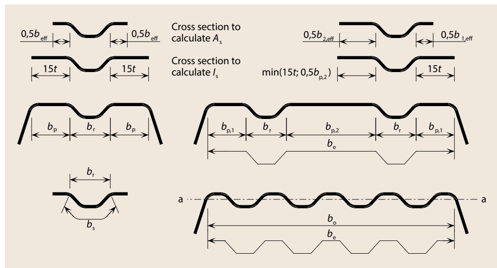
Figure 5.3 Compression flange with one, two or multiple stiffeners
