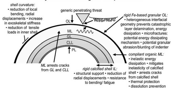
Fig. 5. Schematic of the multilayered design principles of the shell of C. squamiferum . Each material layer serves distinct functional roles leading to many advantages with regards to mechanical protection and penetration resistance.
