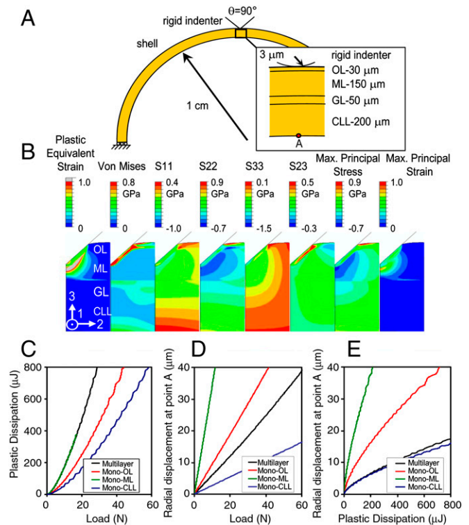
Fig. 3. Computational model of entire multilayered shell of C. squamiferum . (A) Finite element microindentation (indenter radius = 3 \mu\text{m} , included angle = 90°) simulation approximating the shell as hemispherical where the experimentally measured thickness and mechanical properties of the individual layers were taken into account. (B) Predicted stress and strain contours (maximum load, F = 28 N). Prediction of (C) plastic (inelastic) energy dissipation as a function of loading force and (D) radial displacement of point A on inner surface (see A) versus loading force and (E) radial displacement at point A versus plastic (inelastic) dissipation for the multilayered structure compared with three monolayered structures (Mono-OL, Mono-ML, and Mono-CLL).
