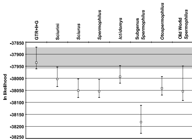
Fig. 6. Comparison between the ln likelihood score for MCMC chains for the unconstrained GTR + G + I model runs and those of alternative runs (with the same model) where particular relationships were constrained. Names of constrained runs represent the groups restricted to monophyly. Likelihood scores are reported as the mean (box) and 95% credibility interval (bars). The shaded area represents the likelihood score range spanned by the 95% credibility interval of the unconstrained MCMC analyses, and represents the region where null hypotheses of constrained relationships would not be rejected.
