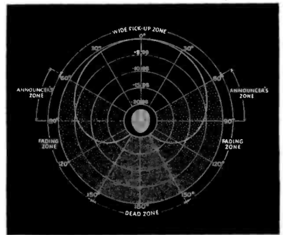
1. Cardioid directional response of 639A.
