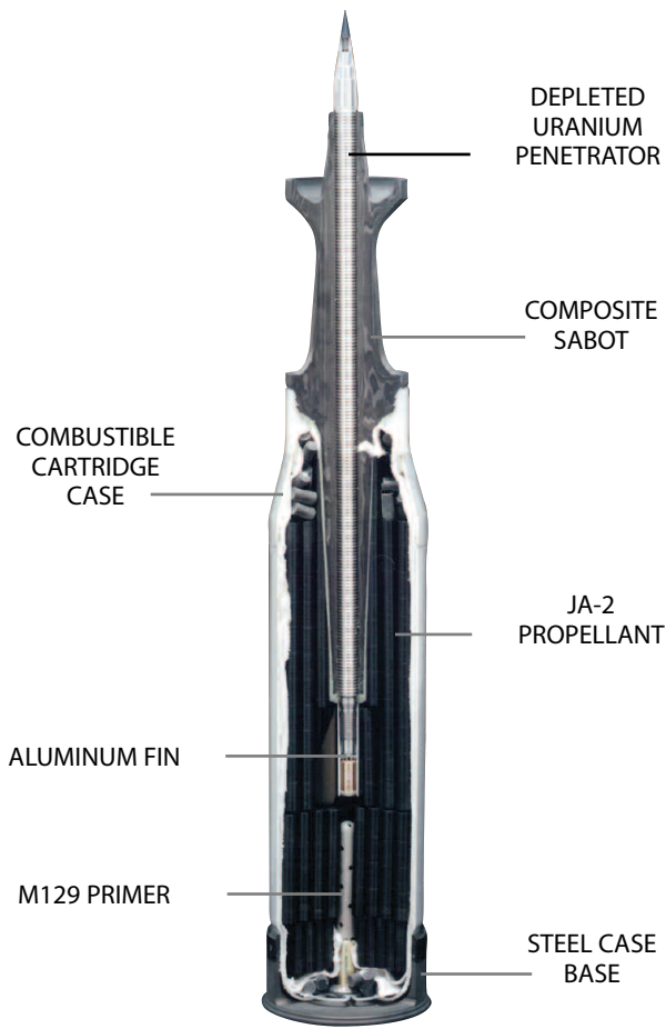
TACTICAL CARTRIDGE M829A2
