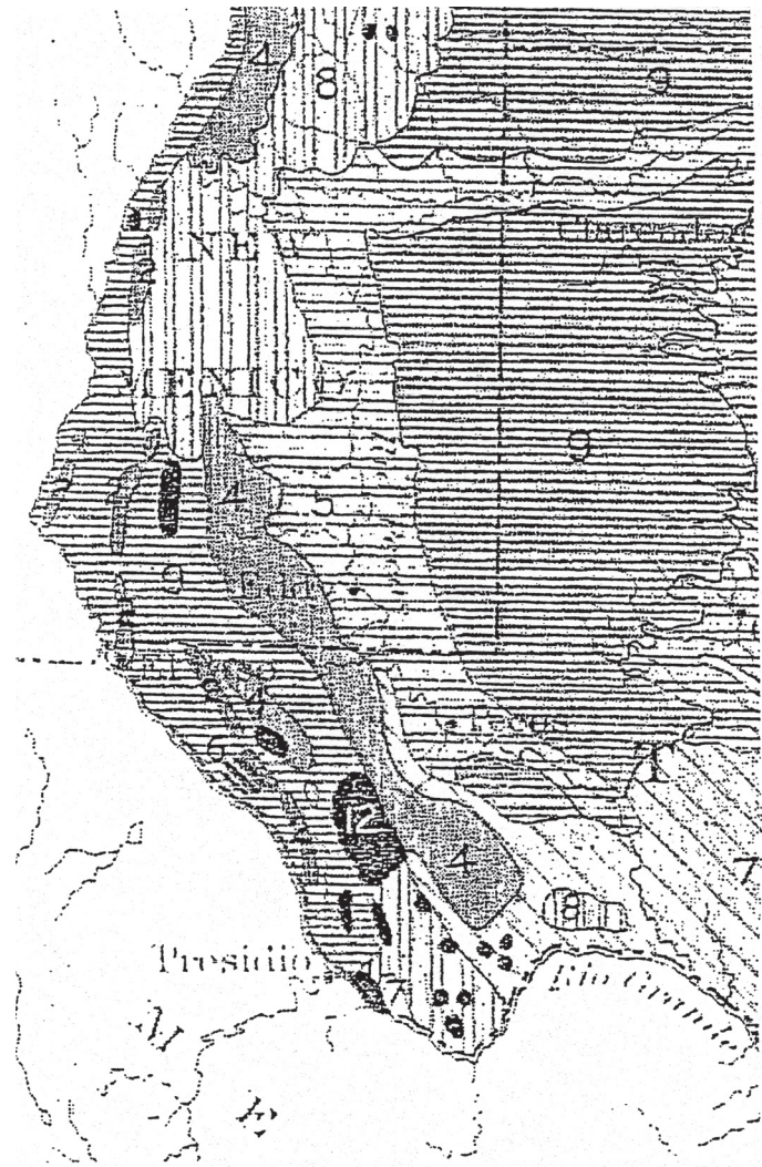
FIGURE 5. Portion of Hill's (1901, pl. 28) geologic map of eastern New Mexico and west Texas. Key: 2, Paleozoic and Mesozoic; 4, Carboniferous; 5, Permian; 7, Lower Cretaceous; 8, Upper Cretaceous; 9, nonmarine Tertiary; 12, later igneous.
