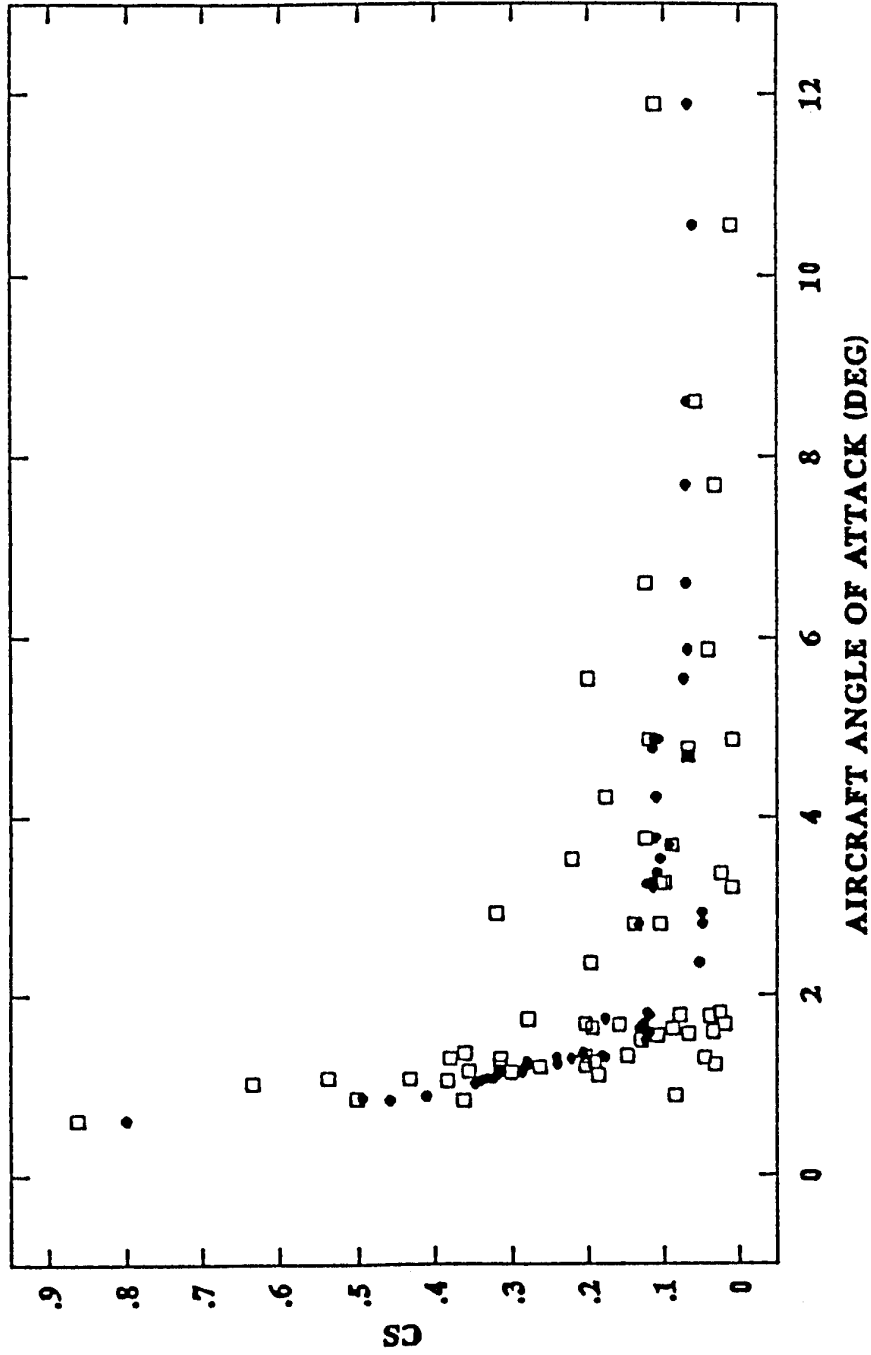
C-6. SEEM Initial Side Force Coefficient Versus Angle of Attack
