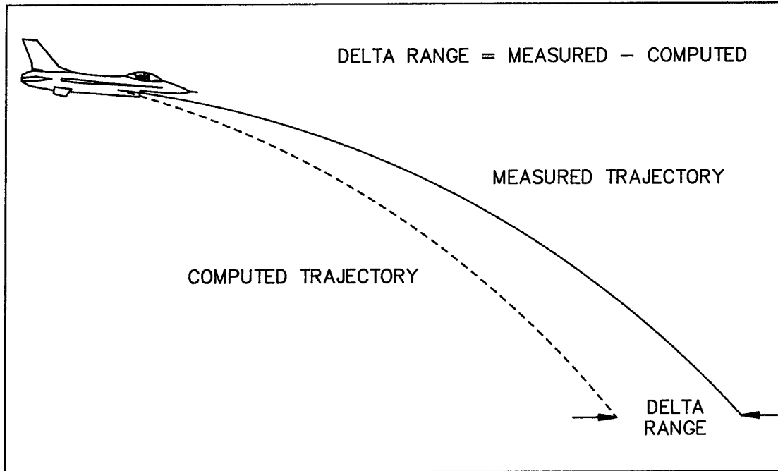
Figure 27. Delta Range
