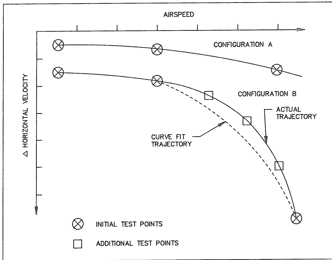
Figure 14. Effect of Airspeed and Configuration on Separation Effects
