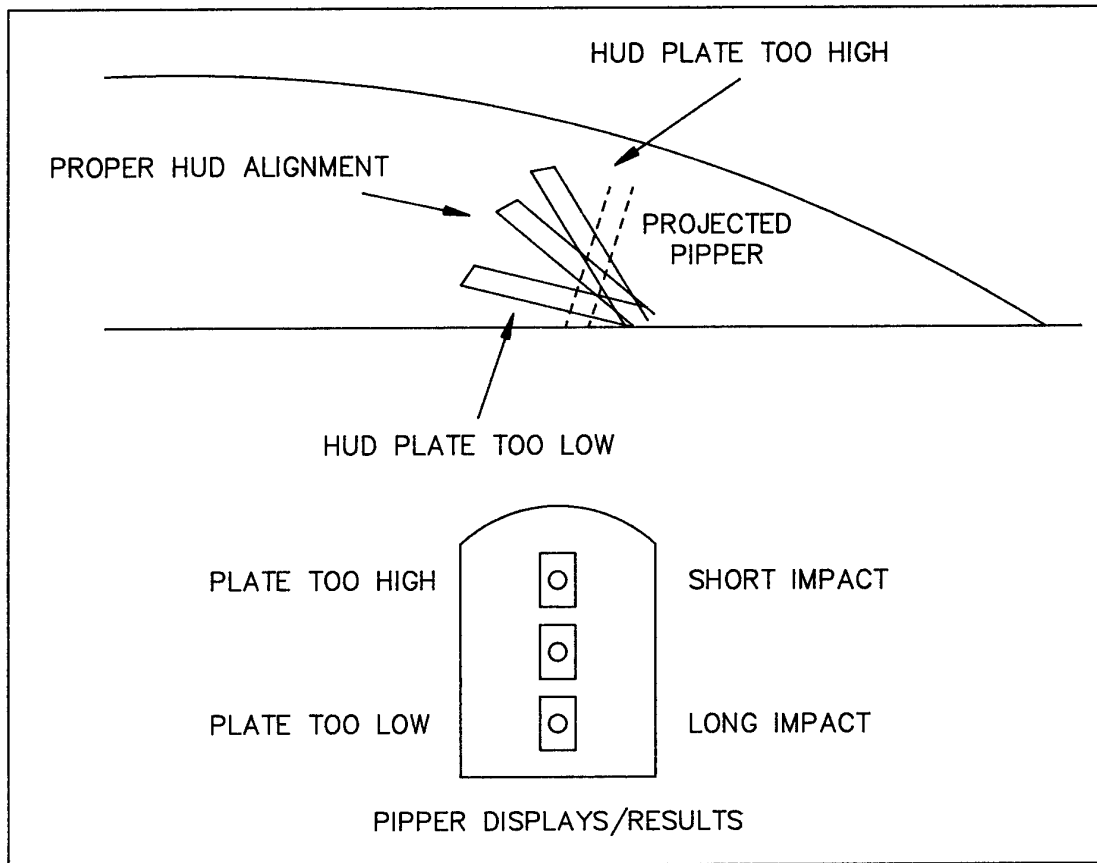
Figure 11. HUD Boresight
