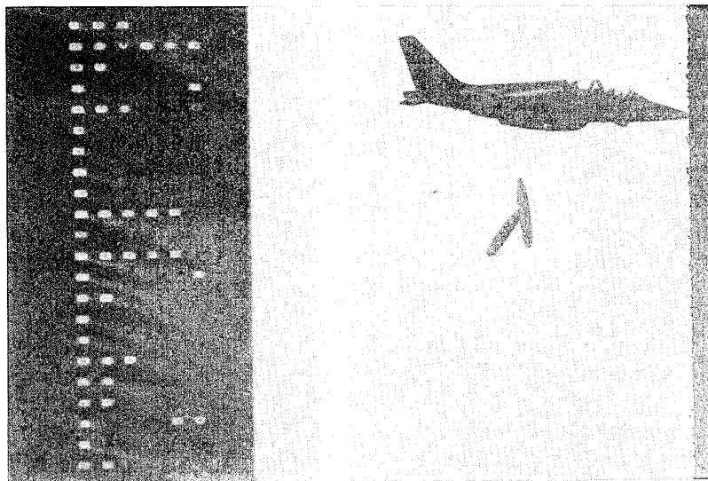
Figure 23(B). Cinetheodolite Photo Coverage of Alpha Jet
