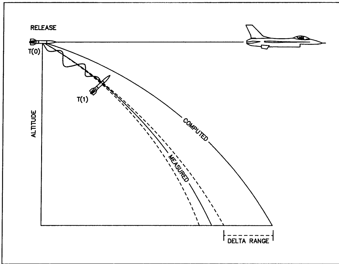
Figure 28. Validation of Freestream Drag
