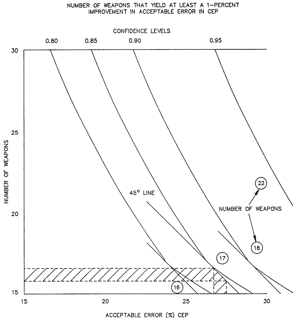
Figure 15. Recommended Number of Weapons
