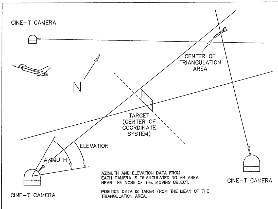
Figure 22. TSPI Raw Data Acquisition
