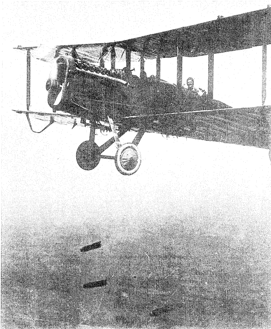
Figure 3. Four 25-Pound Bombs Just After Release from DH-4 Aircraft Using Strap Carriage Racks
