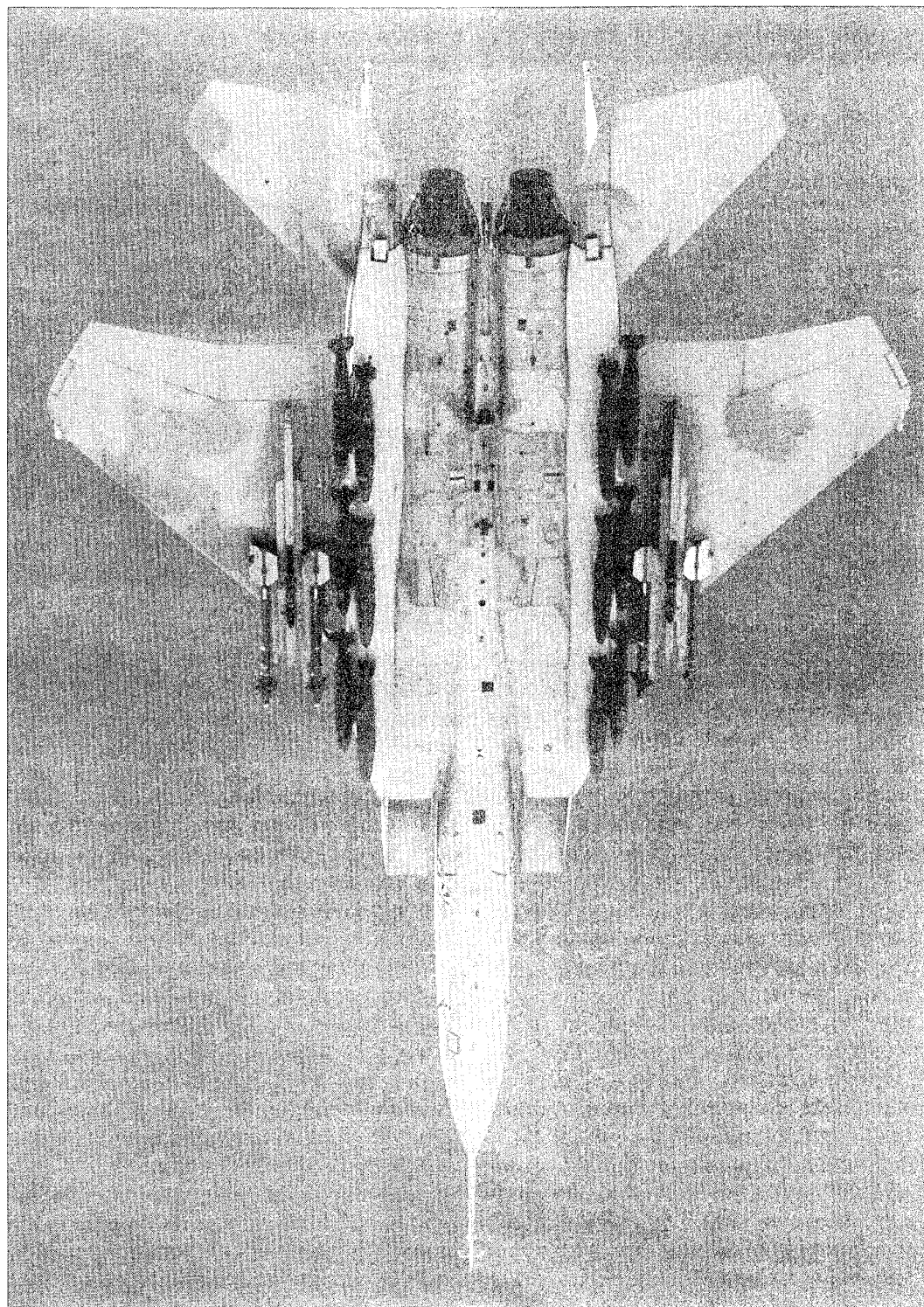
Figure 13. F-15E with Loadout of 12 MK 82 LDGP Bombs
