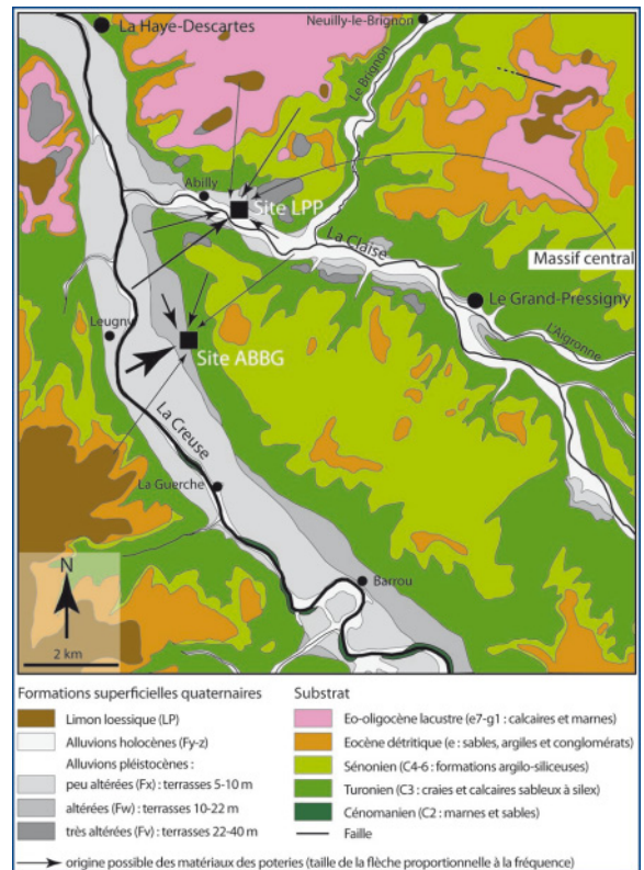
Fig. 2: Geological map of the Grand-Pressigny area (Indre-et-Loire) and possible sources of ceramic raw materials. Based on the 1/50000 map of Preuilly-sur-Claise (Rasplus et al. 1978) and Châtelleraut (Médioni et al. 1974).
