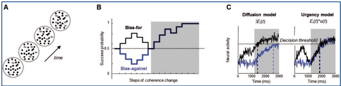
Figure 1: A. Time course of the variable coherence motion discrimination task. Initially, 200 dots move randomly. Then, every 225 ms, a fraction of dots (6, 3 %) begins to move coherently either to the left (black arrows) or to the right (gray arrows). Coherent motion favoring one of the two directions continuously evolves and subjects' task is to guess which net direction will be described by coherently moving dots at the end of the trial. B. Success probability profiles of bias-for (black line) and bias-against (blue line) trials. In both trial types, analyses focus on trials in which decisions are made after the initial bias (shaded gray area). C. Schematic evolution of neural activity of an hypothetical cell that prefers the correct target during "bias-for" (black) and "bias-against" (blue) trials, as predicted by the "diffusion" model (left panel) and the "urgency-gating" model (right panel). For any decision made after the 6 th coherence step (gray area), the integrator model predicts that neural activity will reach the decision threshold (horizontal dotted line) faster in "bias-for" than in "bias-against" trials, resulting in shorter decision times in the former (vertical dotted black line) than in the latter (vertical dotted blue line). The urgency-gating model predicts no difference in behavior for the two trial types when decisions are made after the 6 th coherence step.
