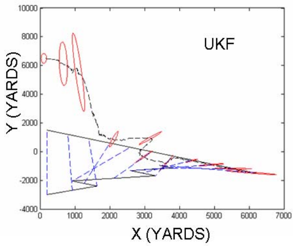
Figure 13: A Comparison of Three Nonlinear Kalman Tracking Filters
