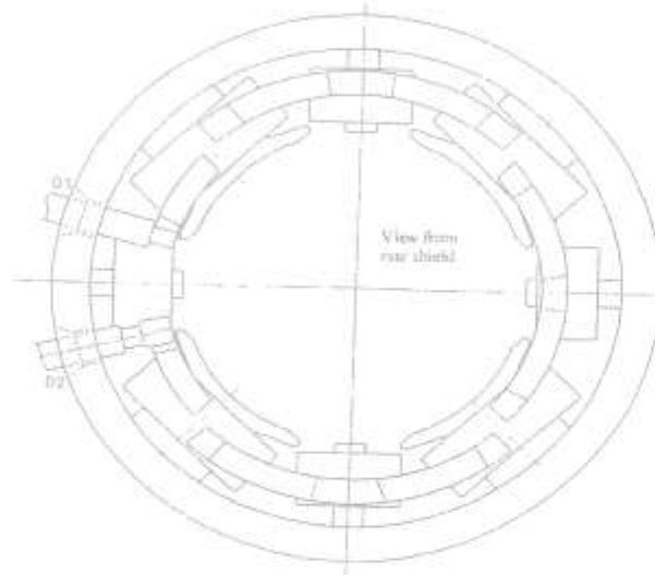
Wiring diagram View from rear shield
