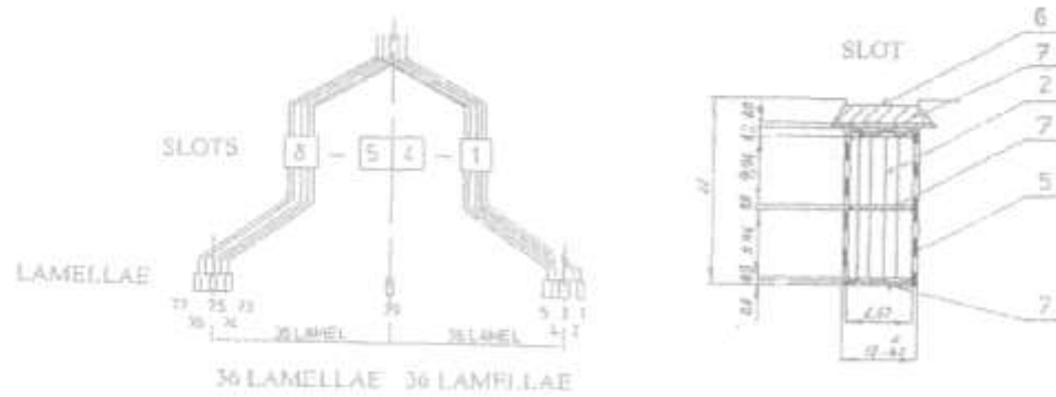
MOUNTING DIAGRAM
