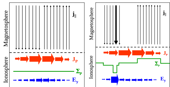
Figure 9. Current circuit cartoon of conditions giving the E_\perp - j_\parallel observed by Cluster and reproduced in our model. (left) A large scale current system in which broad upward and downward field aligned currents close in the ionosphere as Pedersen current. (right) Adding an intense downward field aligned current locally depletes the ionosphere and makes it more electrically insulating. In the cavity, a strong electric field is required to drive the Pedersen current associated with the large scale background current system.
