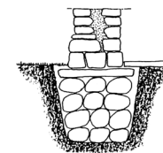
Heas korras vundament. (Joonised: I. Holmström, C. Sandström "Maintenance of old buildings. Preservation from the technical and antiquarian standpoint.")
