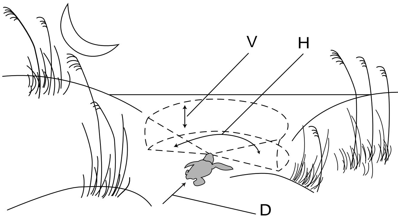
Figure 8. A hypothetical cone of acceptance that describes how a sea turtle hatchling measures the brightest direction. The vertical component of the cone ( V ) is approximately 10^{\circ} – 30^{\circ} from the horizon, and the horizontal component of the cone ( H ) is approximately 180^{\circ} . Light within this cone of acceptance is integrated into an assessment of brightness for the direction D . This description is based on data from studies of green turtles, olive ridleys, and loggerheads (Verheijen and Wildschut, 1973; Witherington, 1992b). Figure adapted from Witherington (1997); used with permission.
