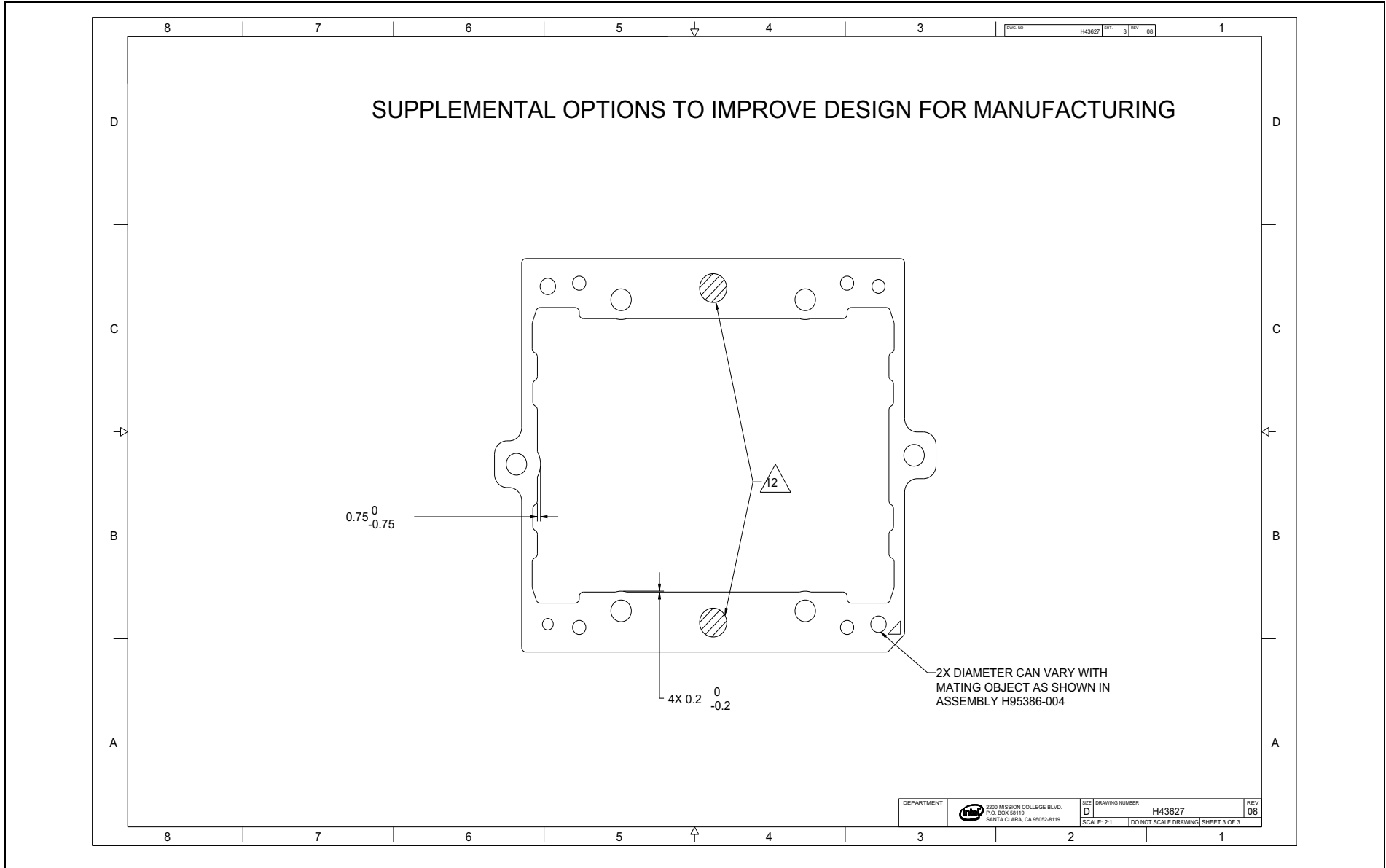
Figure D-12. Square Bolster Plate (Sheet 3 of 3)
