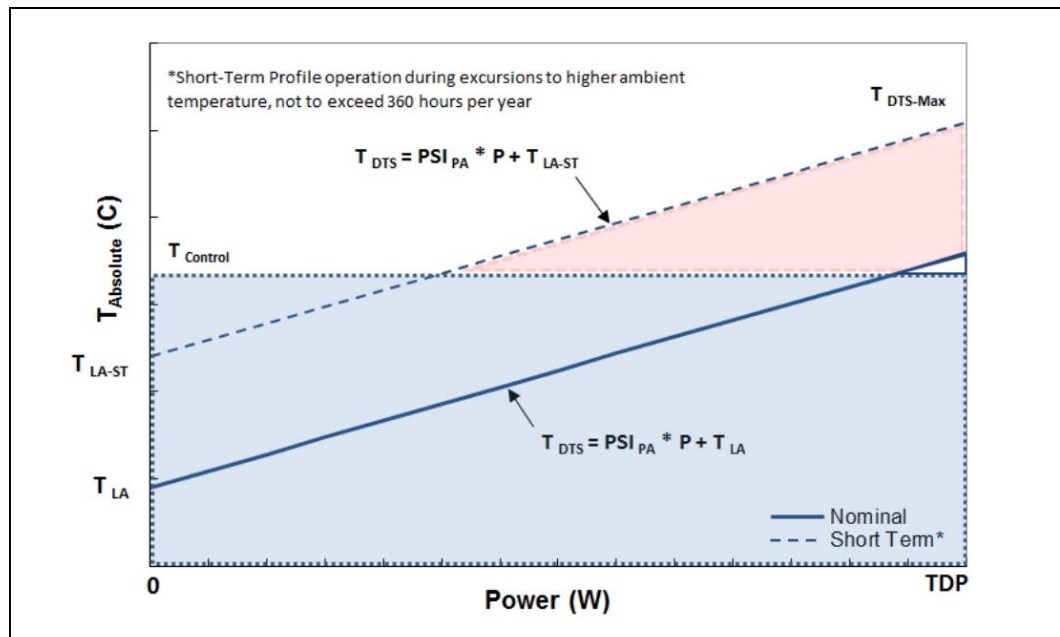
Figure 5-4. NEBS DTS Thermal Profile
