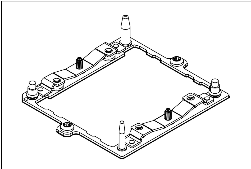
Figure 8-6. Square Bolster Plate Assembly (ISO View)
