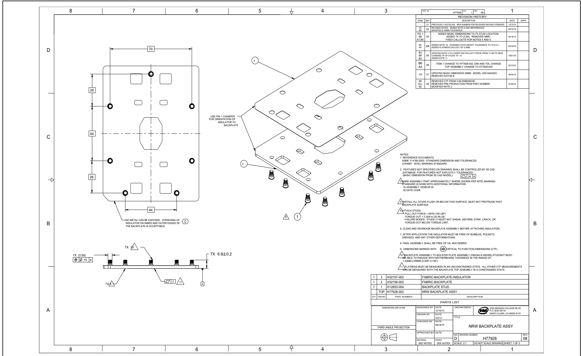
Figure D-19. Narrow Backplate Assembly (Sheet 1 of 2)
