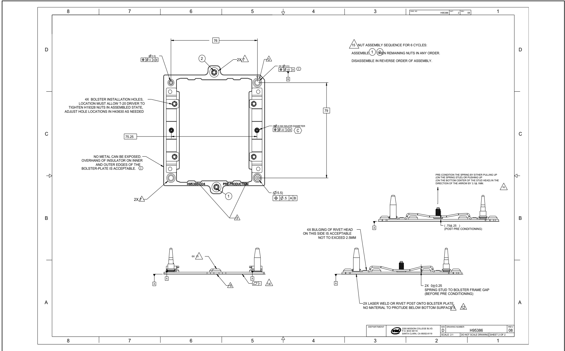
Figure D-30. Square Bolster Plate Assembly (Sheet 2 of 2)
