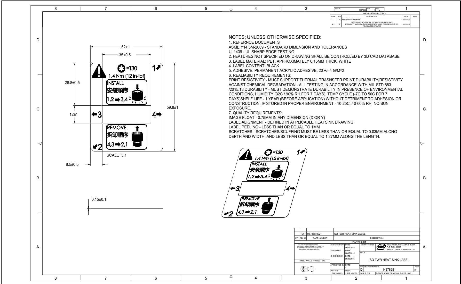
Figure E-22. Square Tower Heatsink Label
