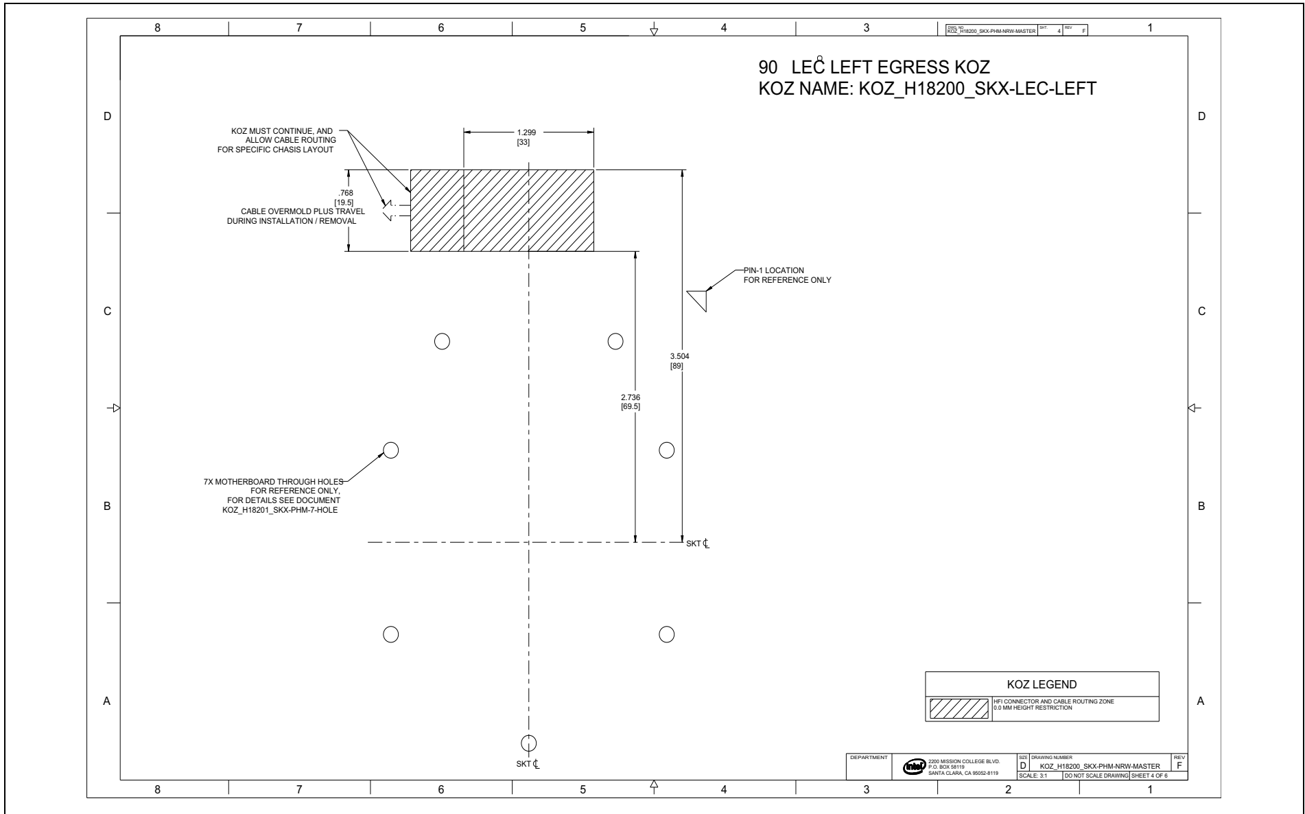
Figure F-3. KOZ: PHM Narrow Master (Sheet 4 of 6)
