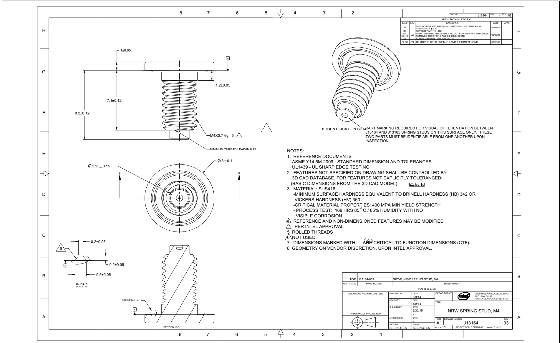
Figure D-32. Narrow Spring Stud
