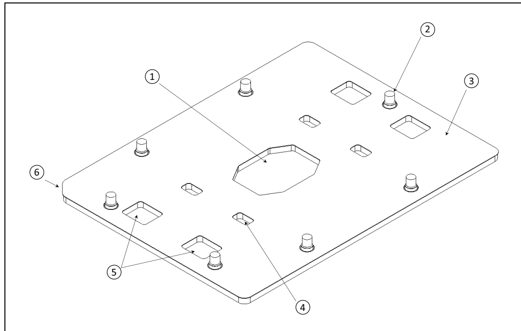
Figure 8-9. Narrow Back Plate Part Feature
