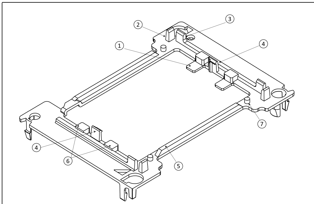
Figure 8-15. Narrow Non-Fabric Package Carrier Mechanical Features (Bottom View)
