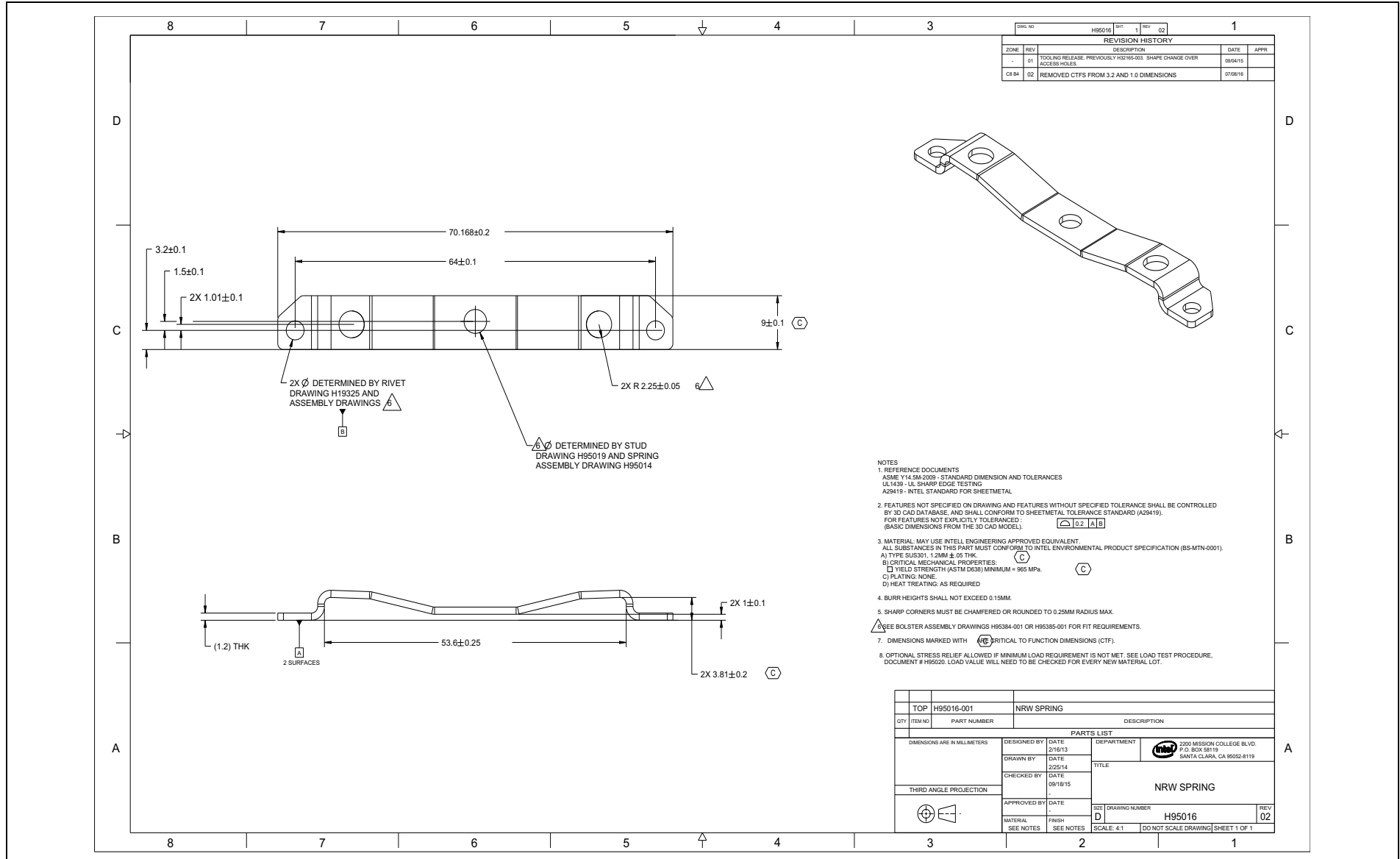
Figure D-25. Narrow Spring
