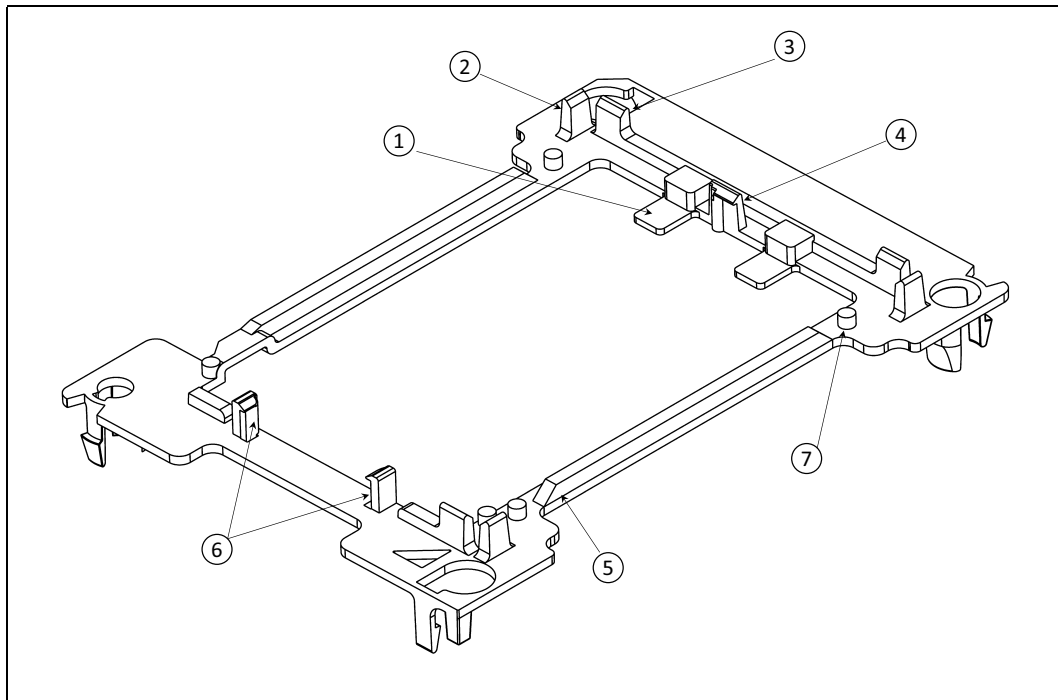
Figure 8-13. Narrow Fabric Package Carrier Mechanical Features (Bottom View)
