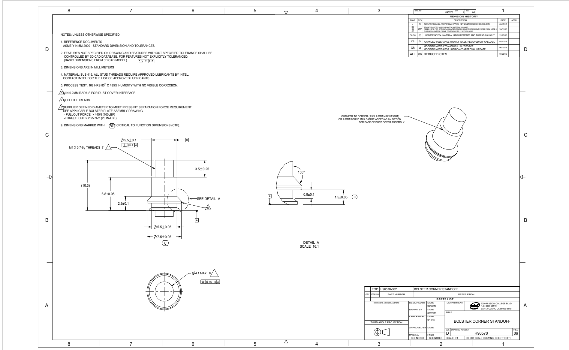
Figure D-31. Bolster Corner Standoff
