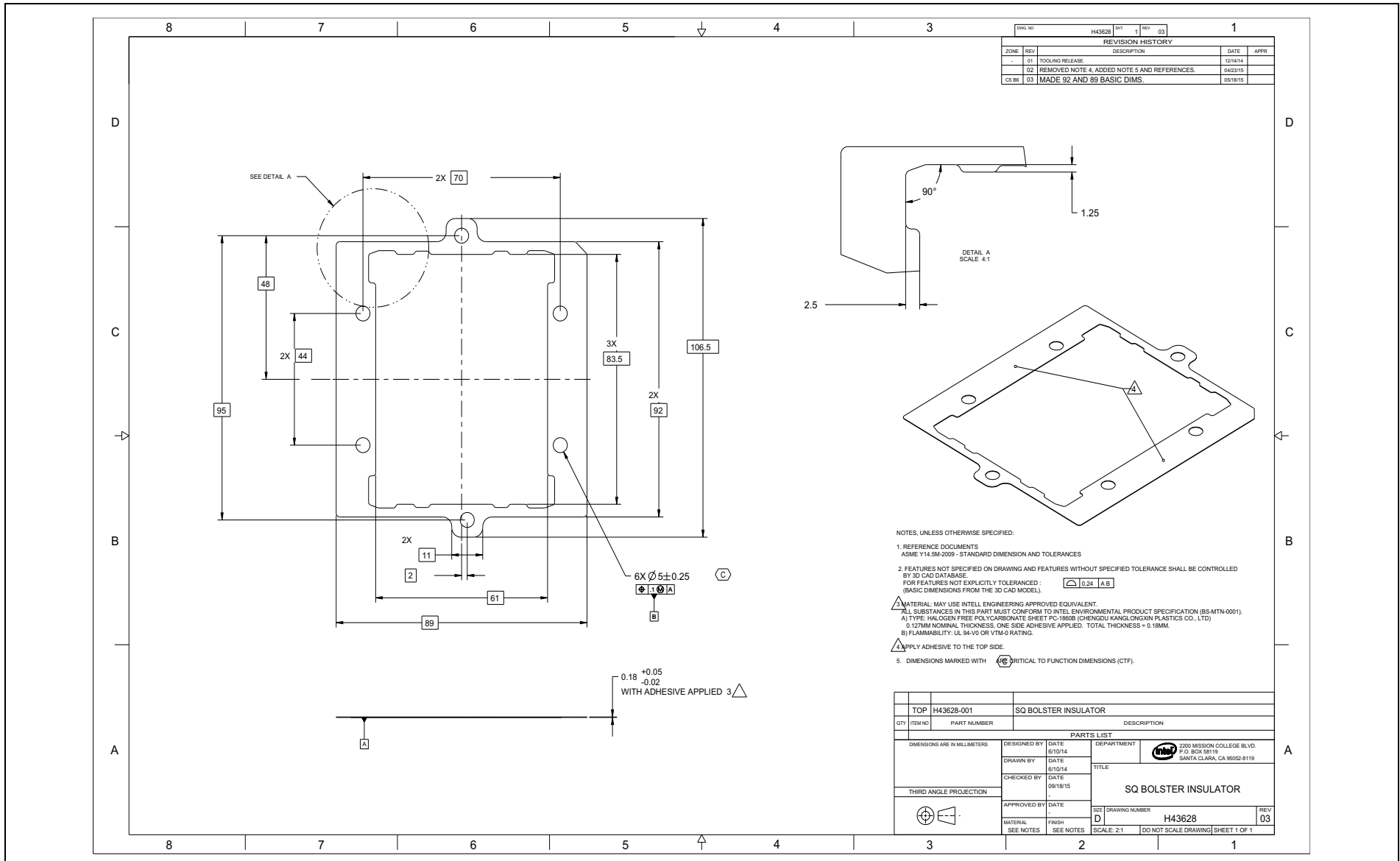
Figure D-13. Square Bolster Insulator
