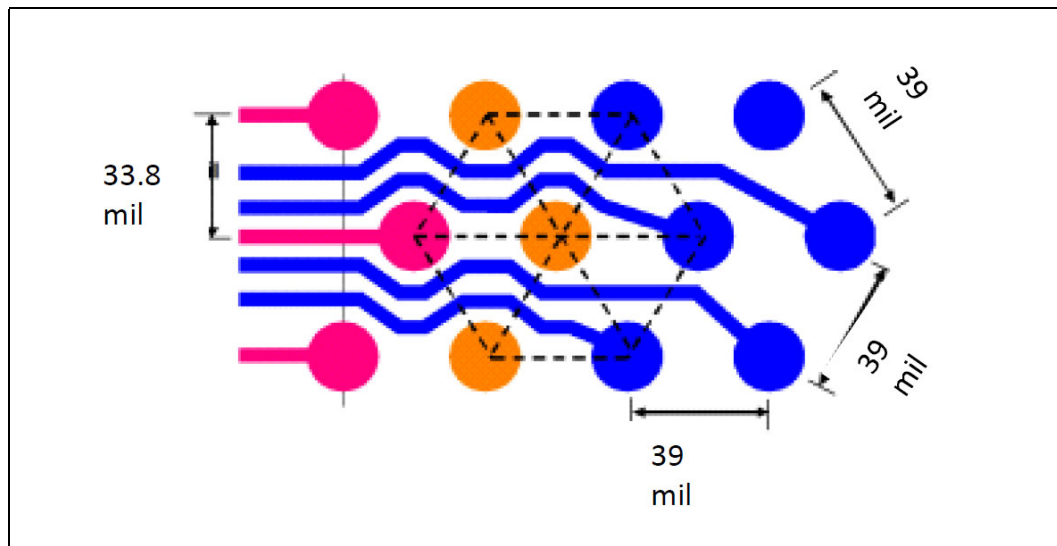
Figure 3-12. LGA3647-0 Socket PCB Land Pattern
