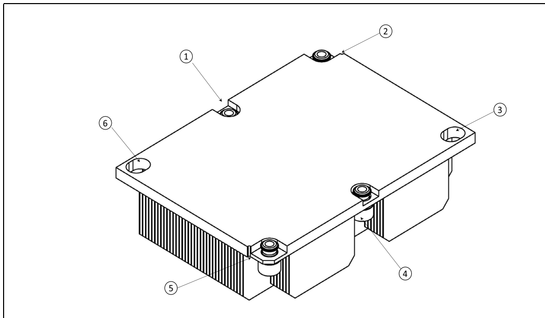
Figure 8-19. Heatsink Base Mechanical Features
