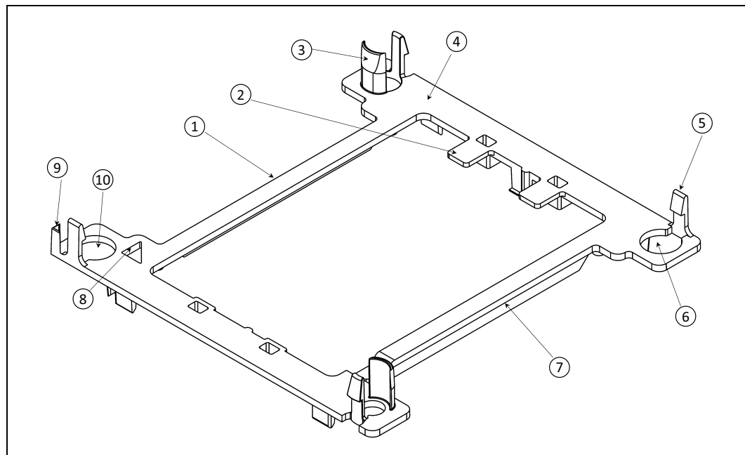
Square Package Carrier Mechanical Features (Top View)
