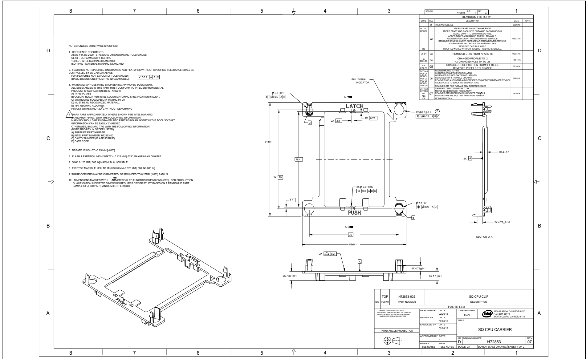
Figure D-18. Square CPU Carrier (Sheet 1 of 2)
