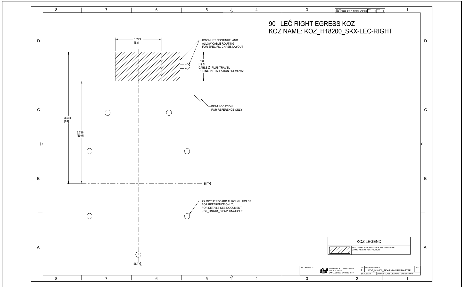
Figure F-3. KOZ: PHM Narrow Master (Sheet 6 of 6)
