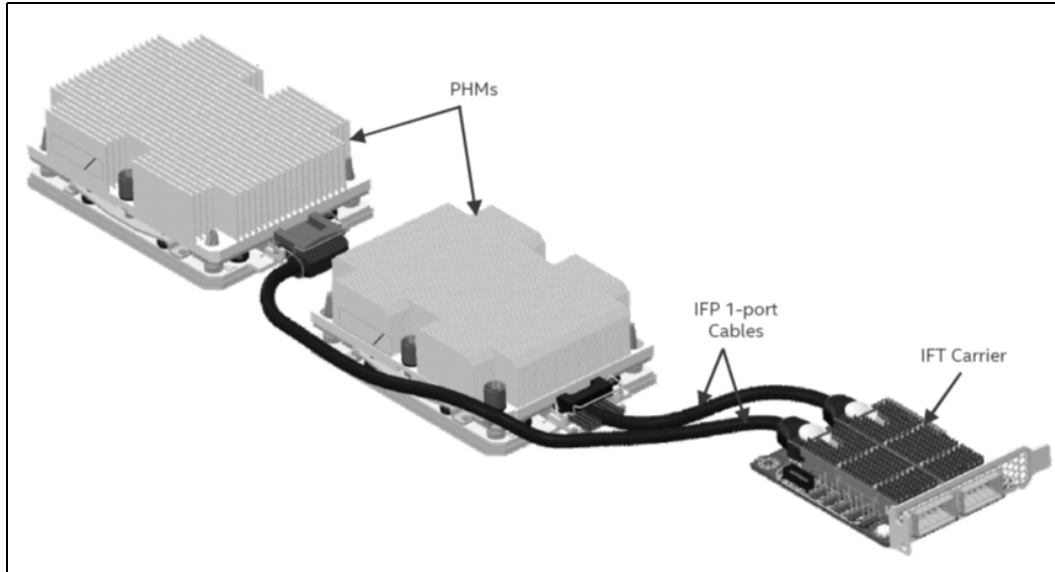
Figure 1-3. PHM Assembly with IFP Internal Cable in Shadowing Configuration and IFT Connector Carrier Card
