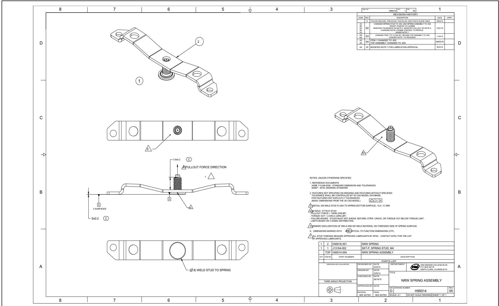
Figure D-24. Narrow Spring Assembly
