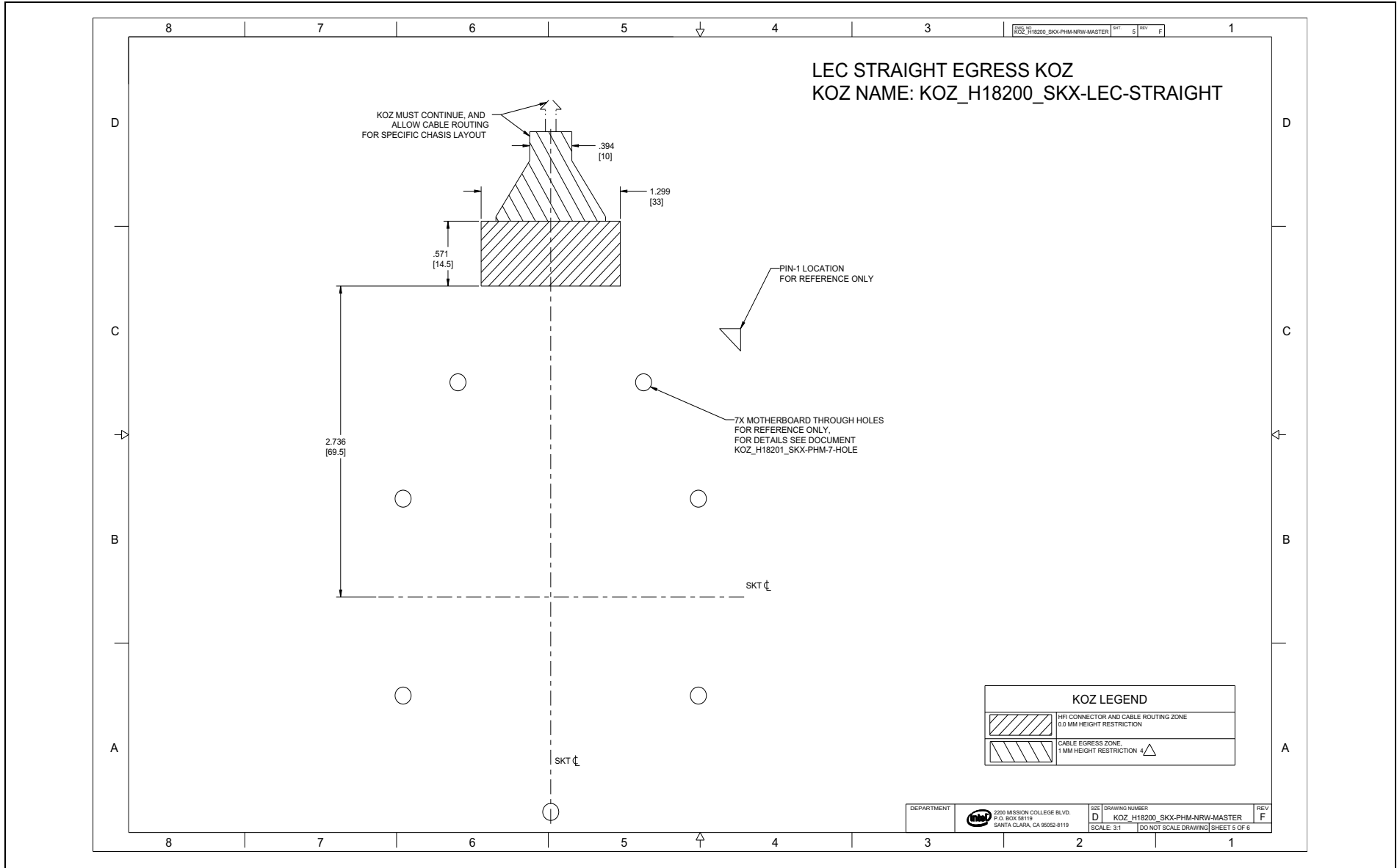
Figure F-3. KOZ: PHM Narrow Master (Sheet 5 of 6)
