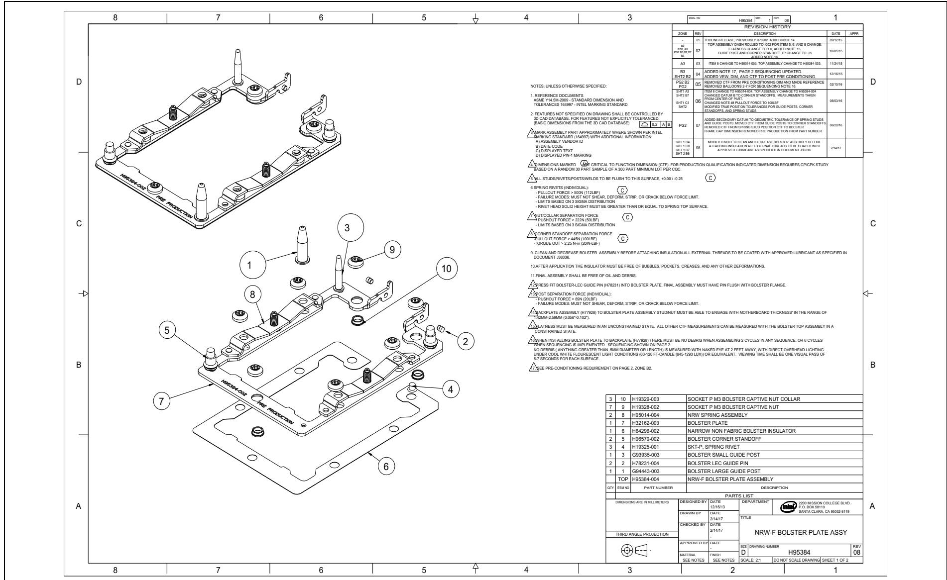
Figure D-28. Narrow - Fabric Bolster Plate Assembly (Sheet 1 of 2)
