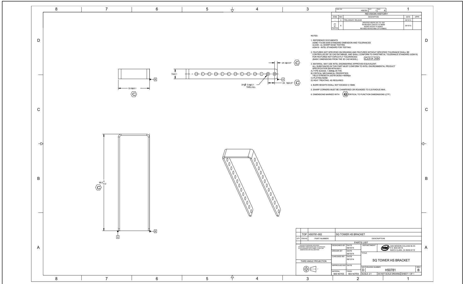
Figure E-20. Square Tower Heatsink Bracket
