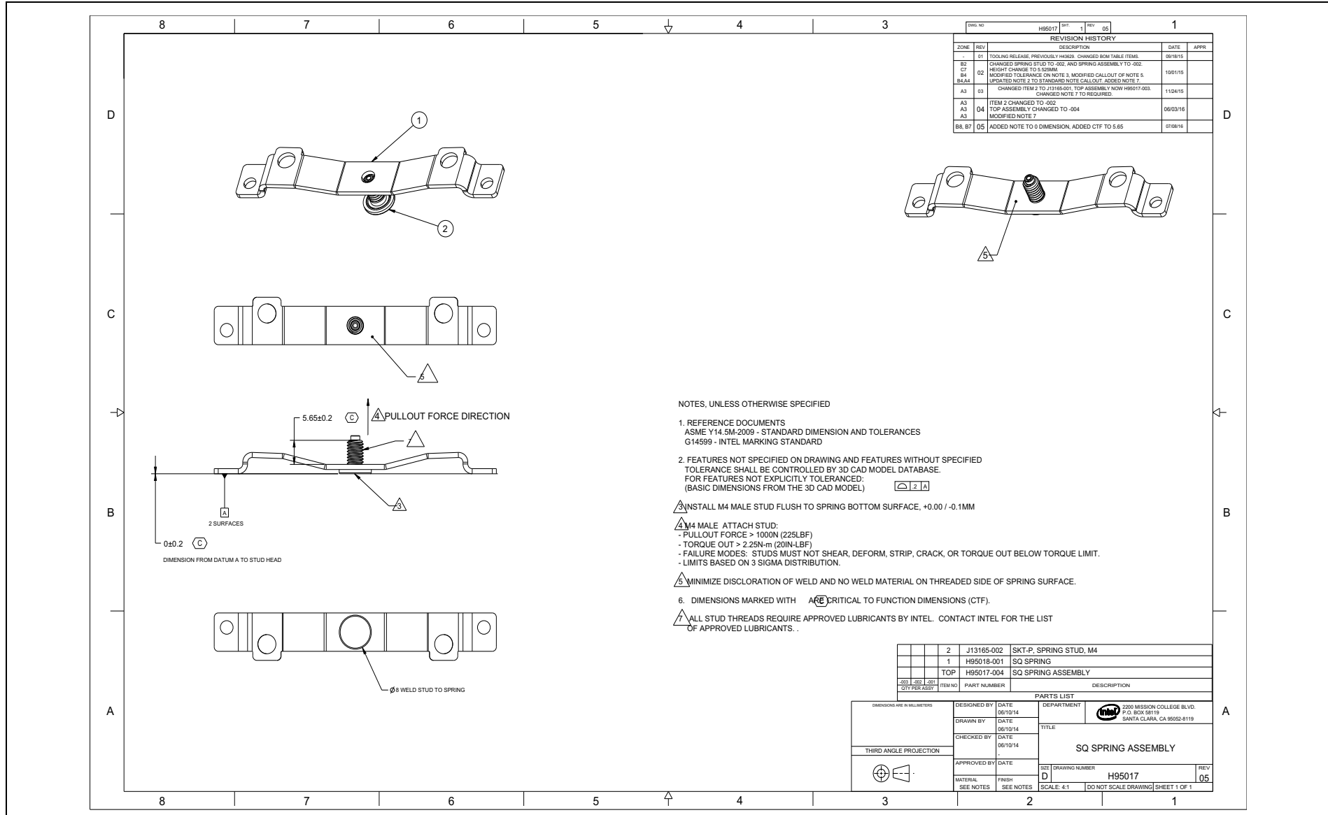
Figure D-26. Square Spring Assembly
