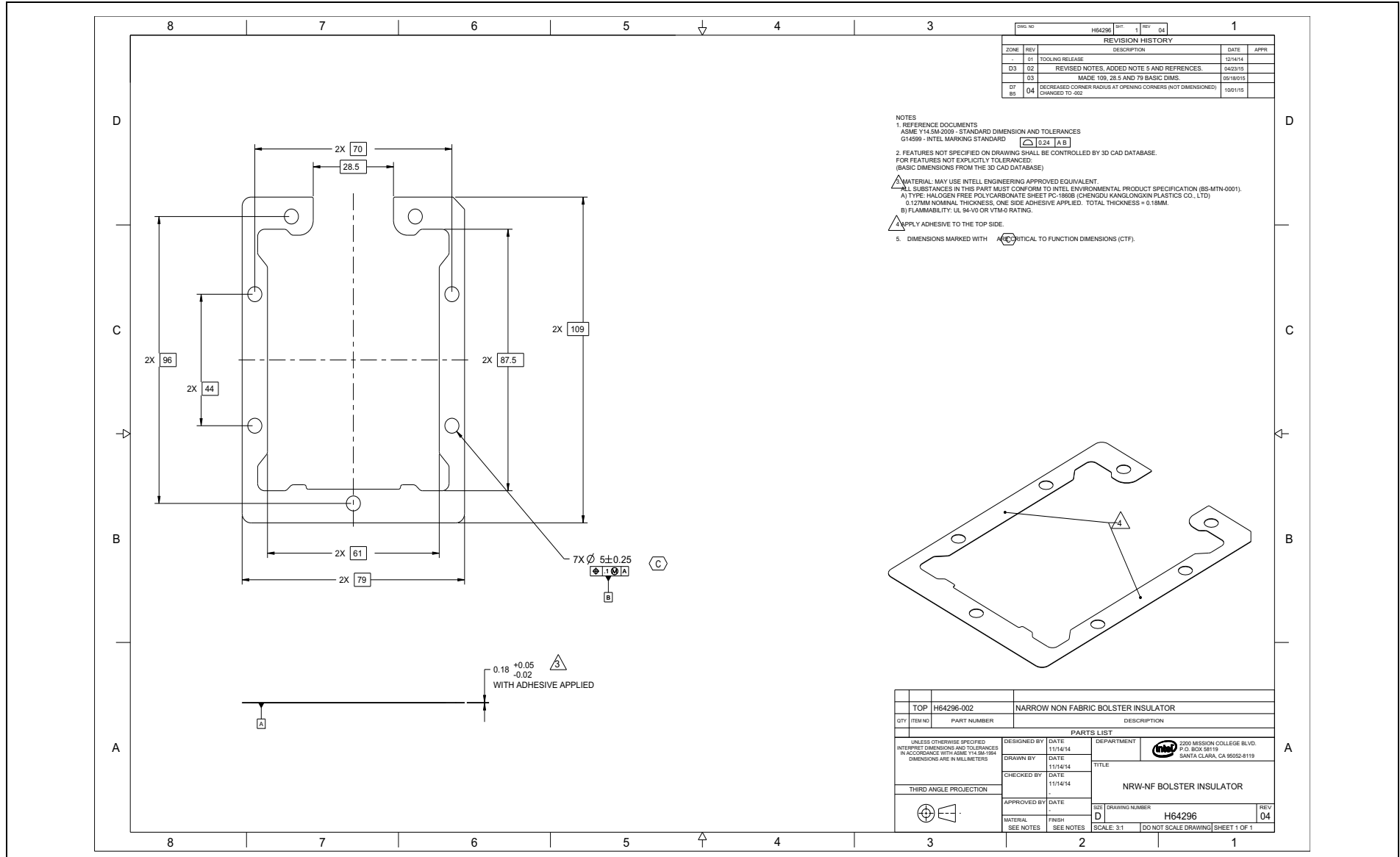
Figure D-15. Narrow Bolster Insulator
