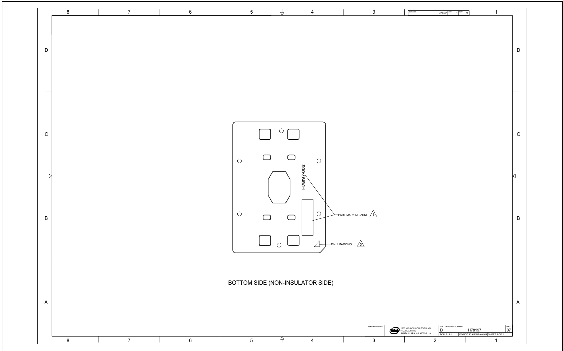
Figure D-21. Square Backplate Assembly (Sheet 2 of 2)
