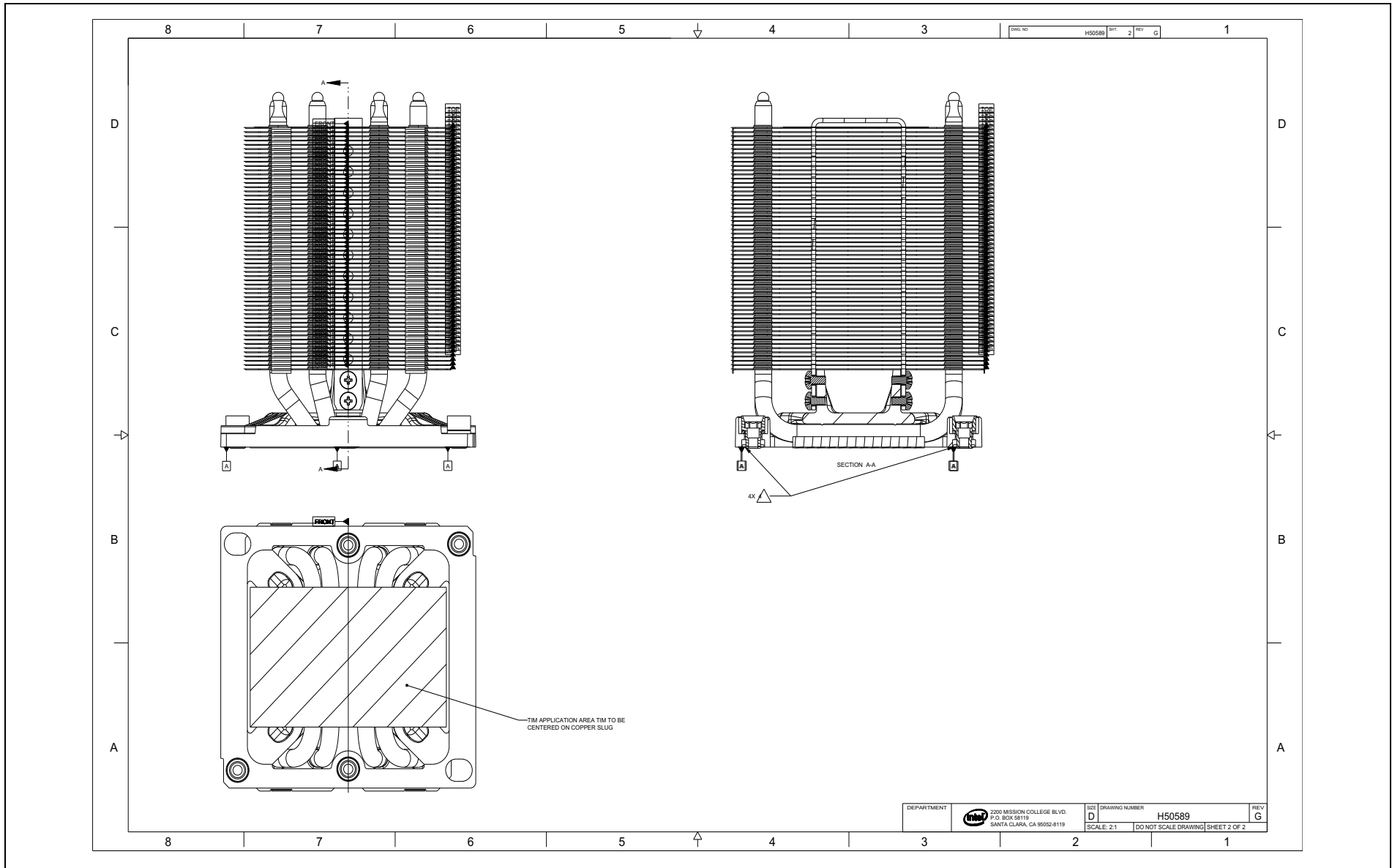
Figure E-14. Square Tower Heatsink Assembly (Sheet 2 of 2)
