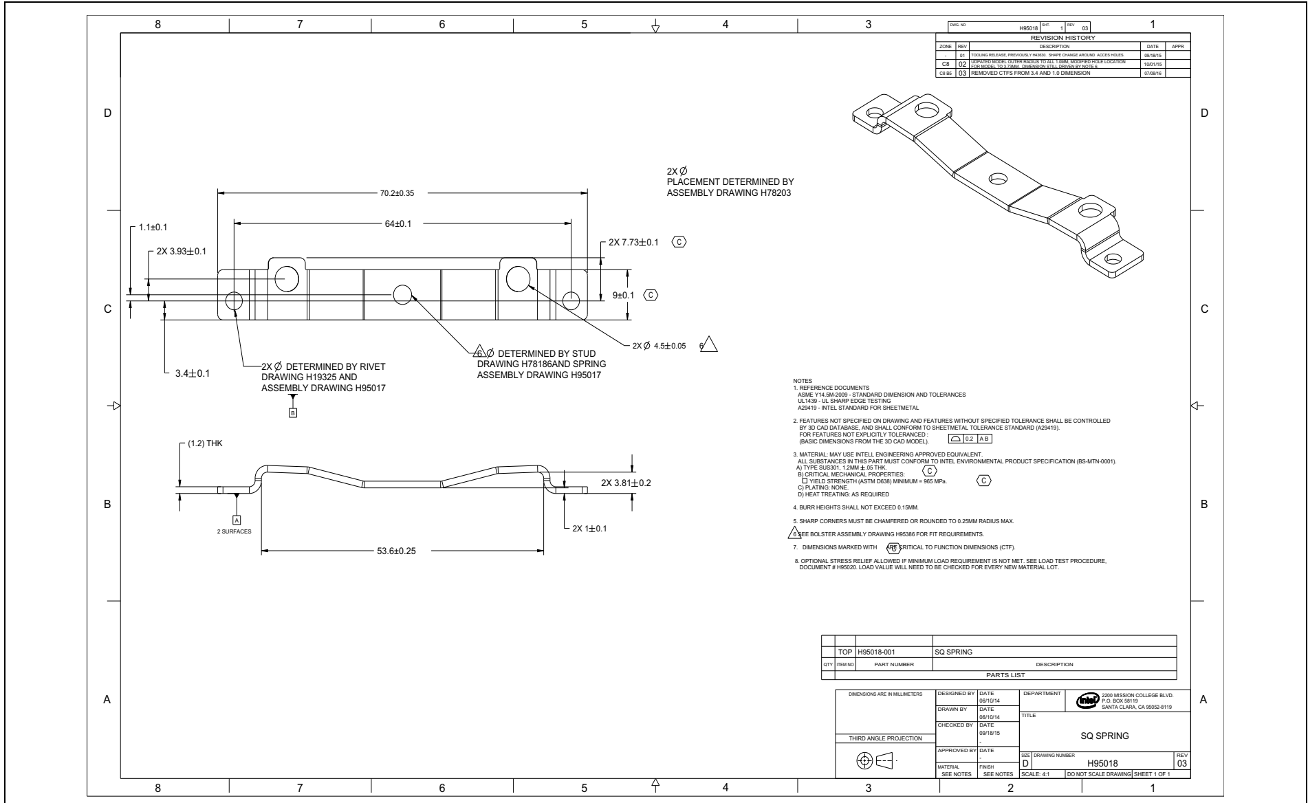
Figure D-27. Square Spring
