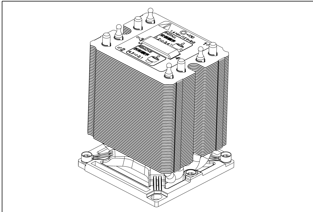
Figure 10-4. Workstation Passive Square Heat Pipe Heatsink
