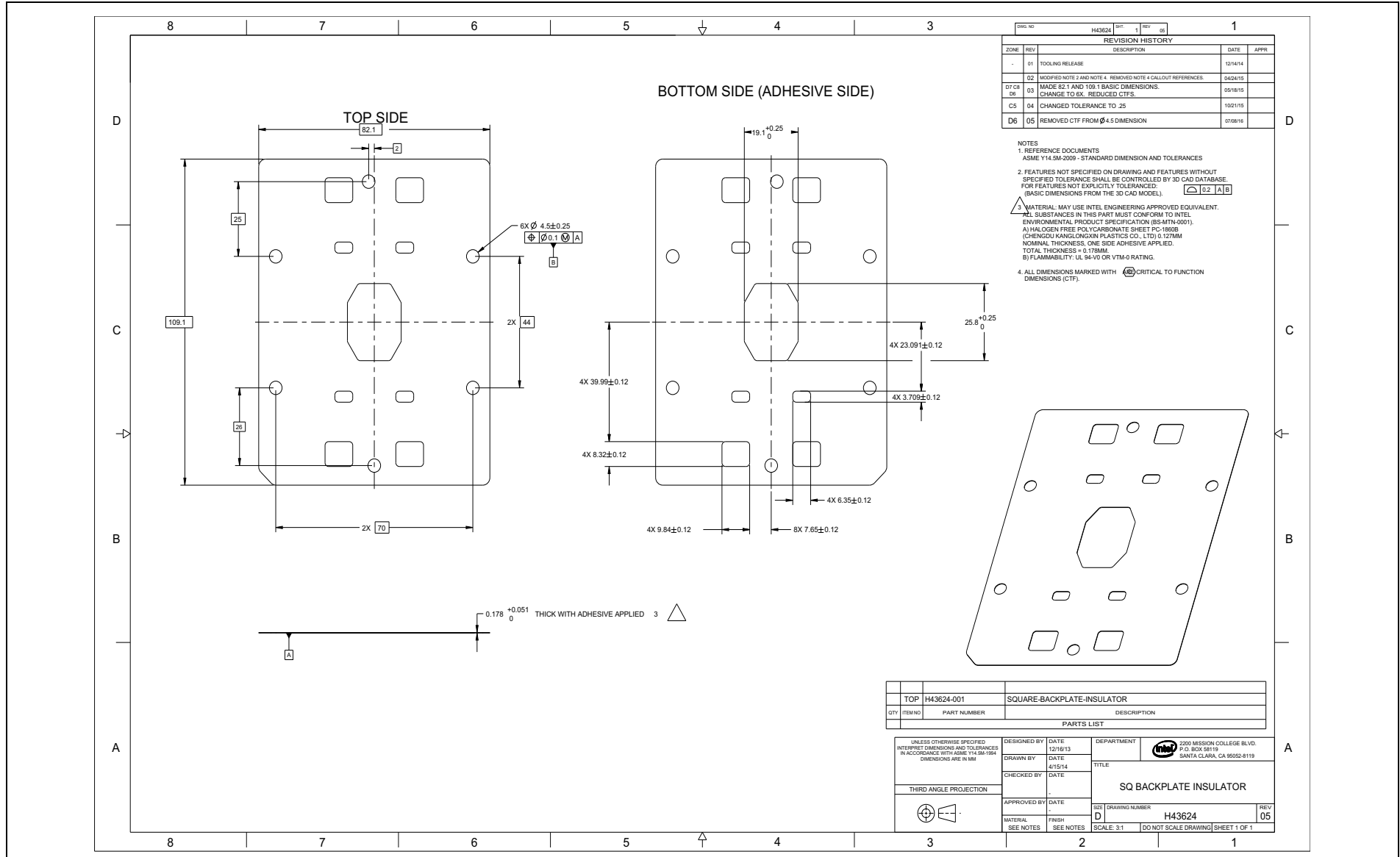
Figure D-11. Square Backplate Insulator
