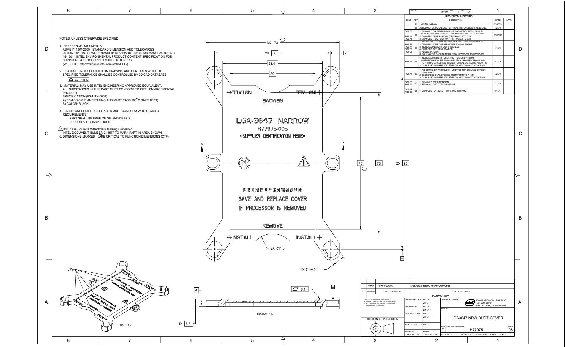
Figure D-20. Narrow Dust Cover (Sheet 1 of 2)
