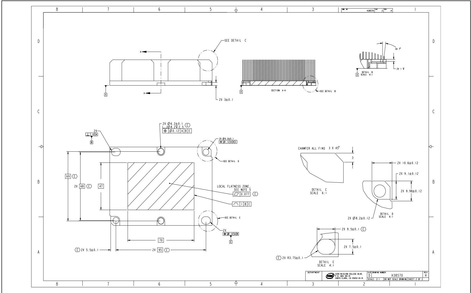
Figure E-10. 1U Heatsink (Sheet 2 of 2)
