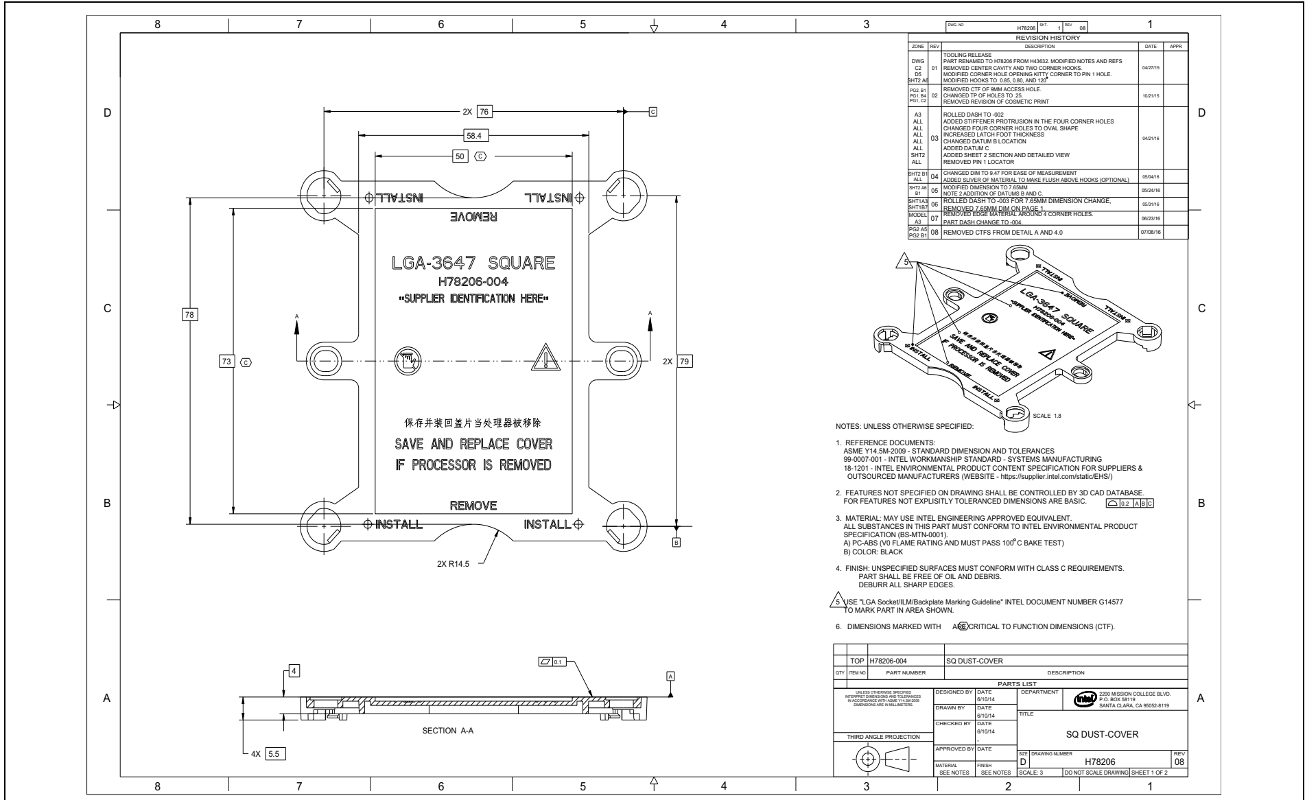
Figure D-22. Square Dust Cover (Sheet 1 of 2)
