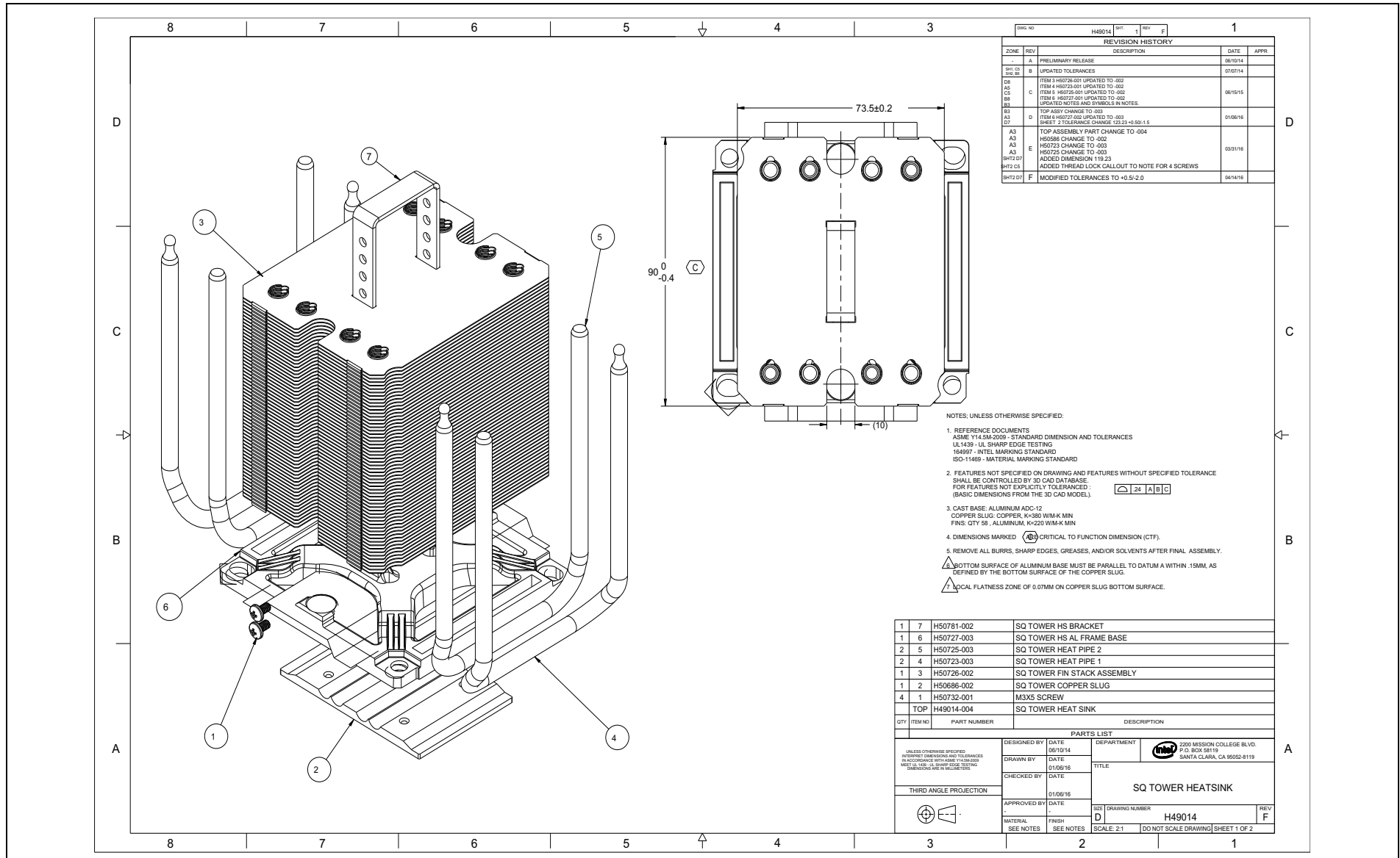
Figure E-13. Square Tower Heatsink (Sheet 1 of 2)
