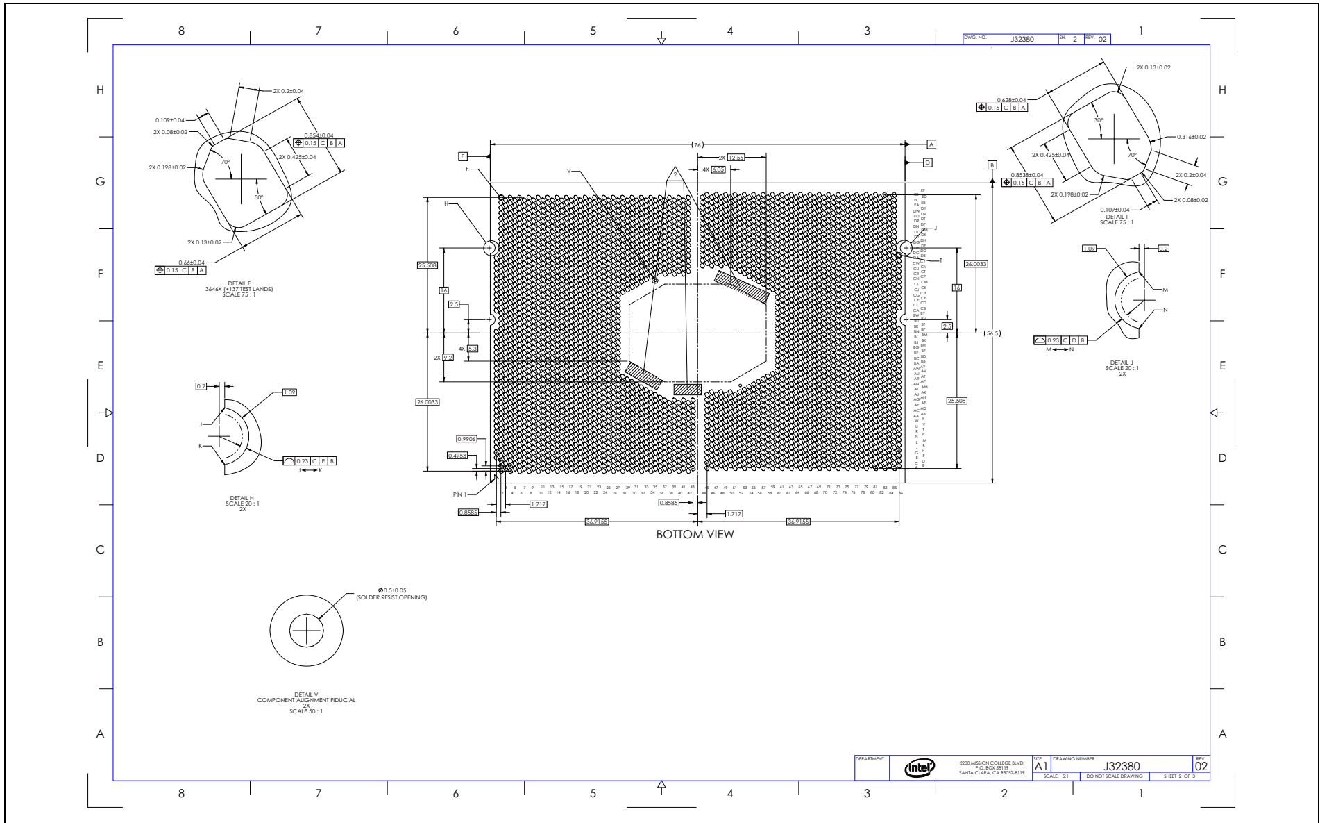
Figure B-4. PMD LCC Form Factor (Sheet 2 of 3)
