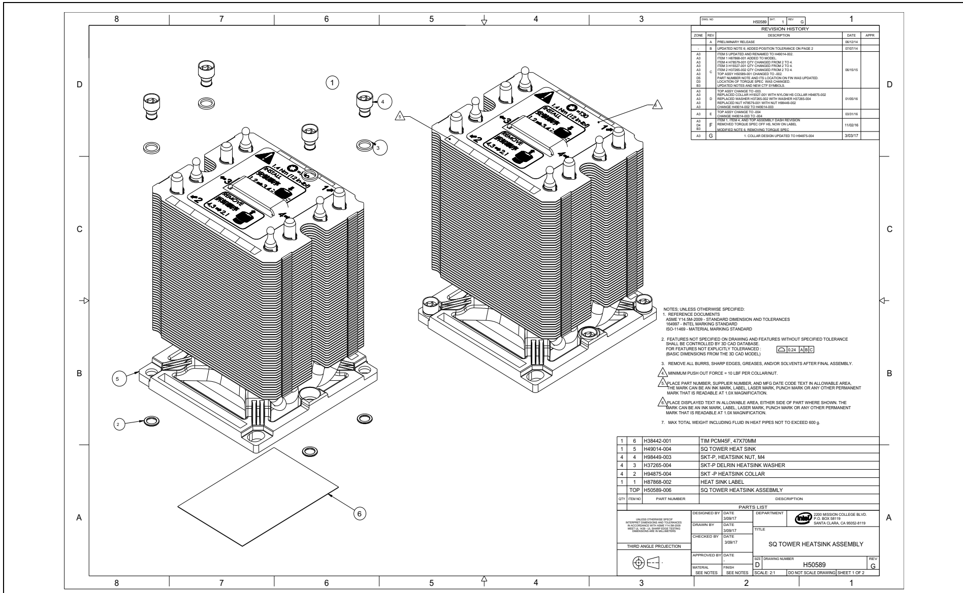
Figure E-14. Square Tower Heatsink Assembly (Sheet 1 of 2)
