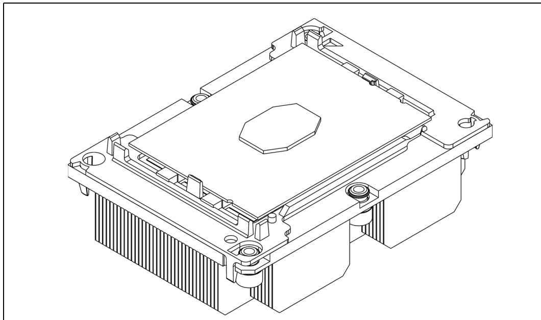
Figure 8-18. PHM Assembly (Bottom View)
