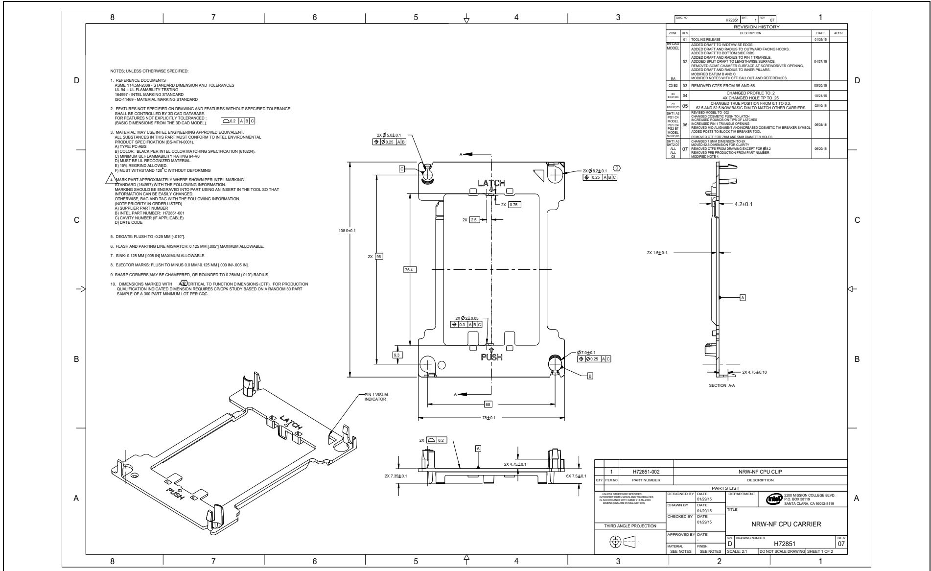
Figure D-17. Narrow CPU Carrier (Sheet 1 of 2)
