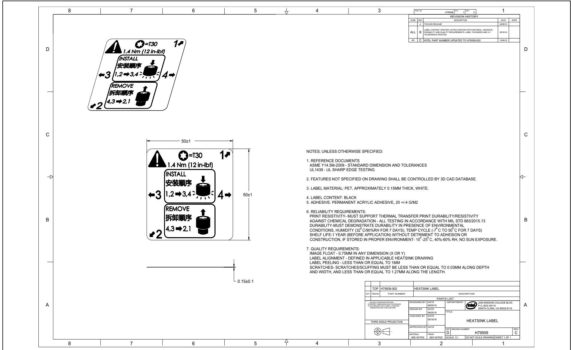
Figure E-21. Heatsink Label
