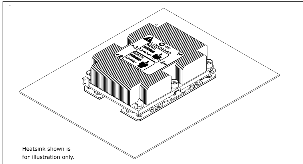
Figure 1-2. PHM Assembly without the IFP Internal Cable
