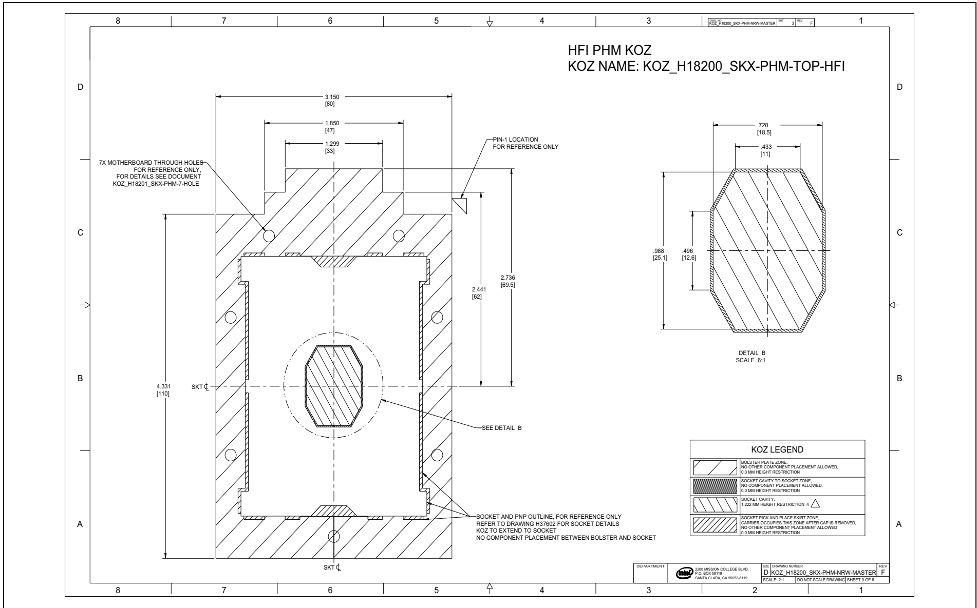
Figure F-3. KOZ: PHM Narrow Master (Sheet 3 of 6)
