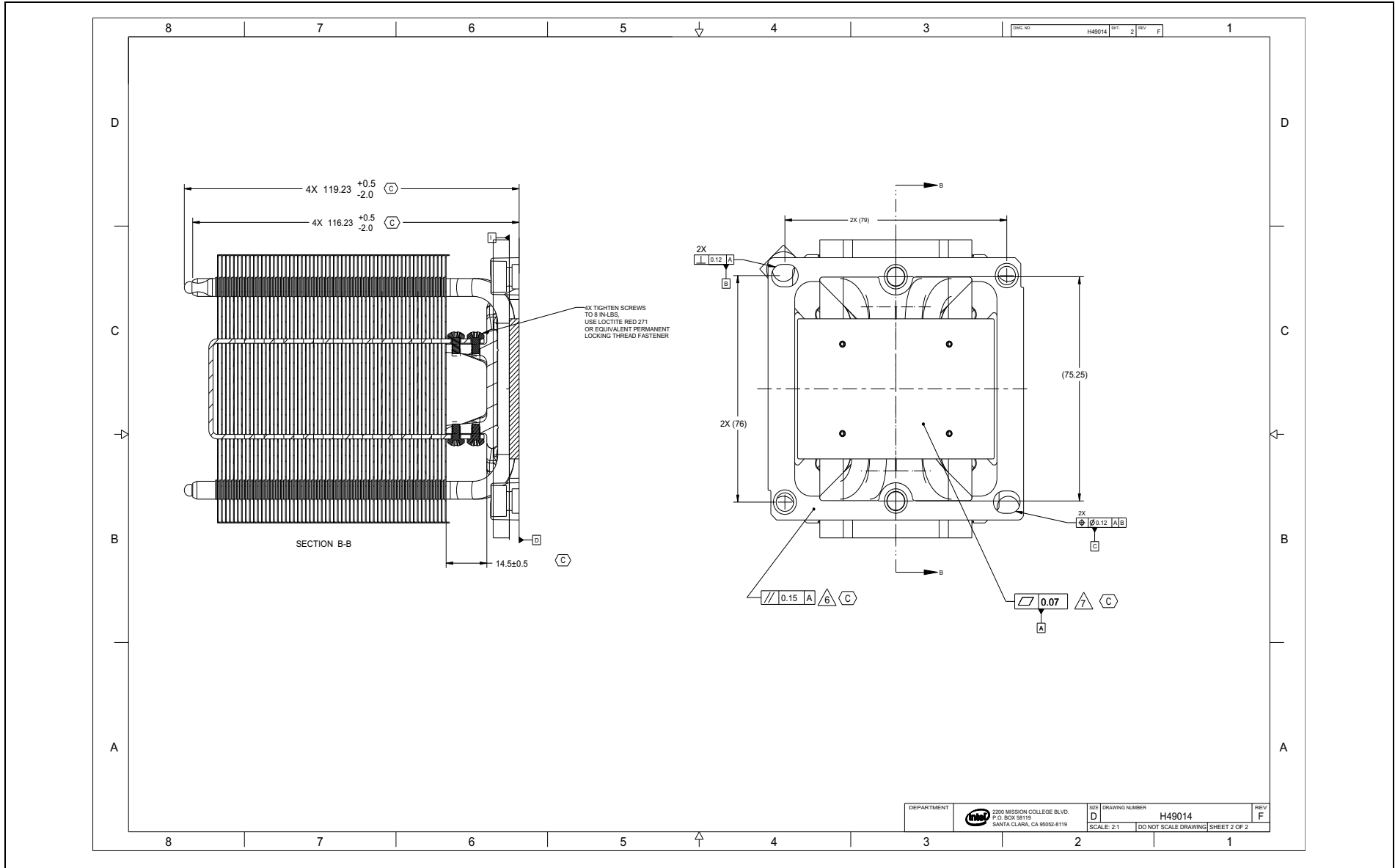
Figure E-13. Square Tower Heatsink (Sheet 2 of 2)
