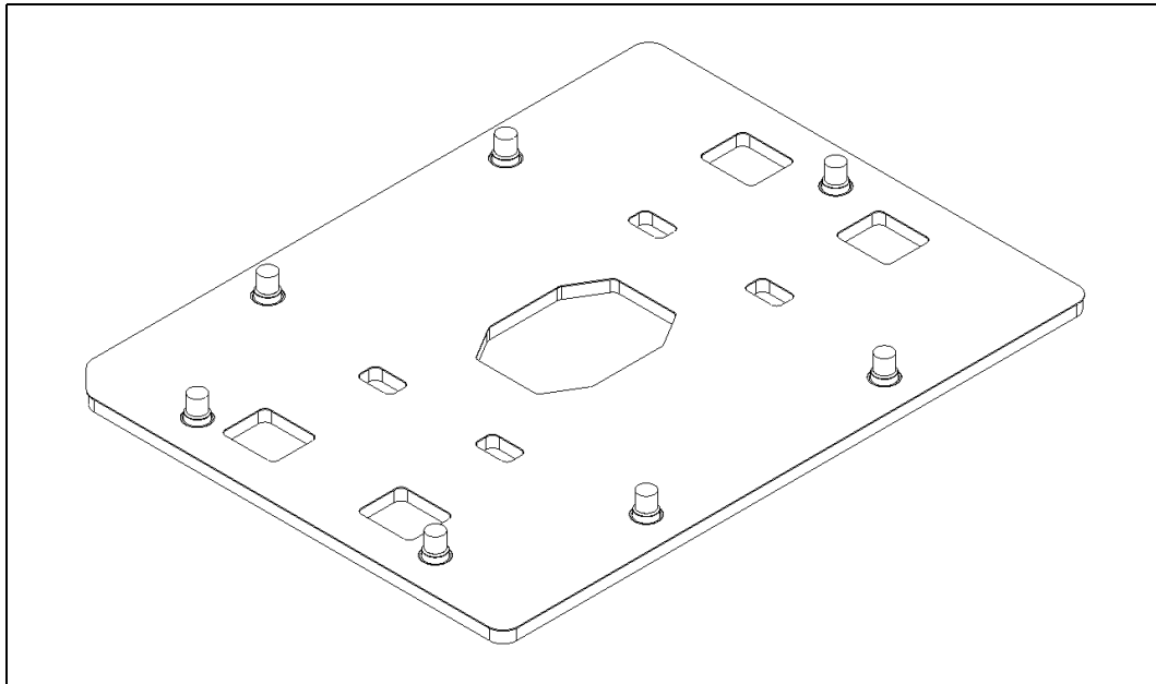
Figure 8-6. Square Bolster Plate Assembly (ISO View)
