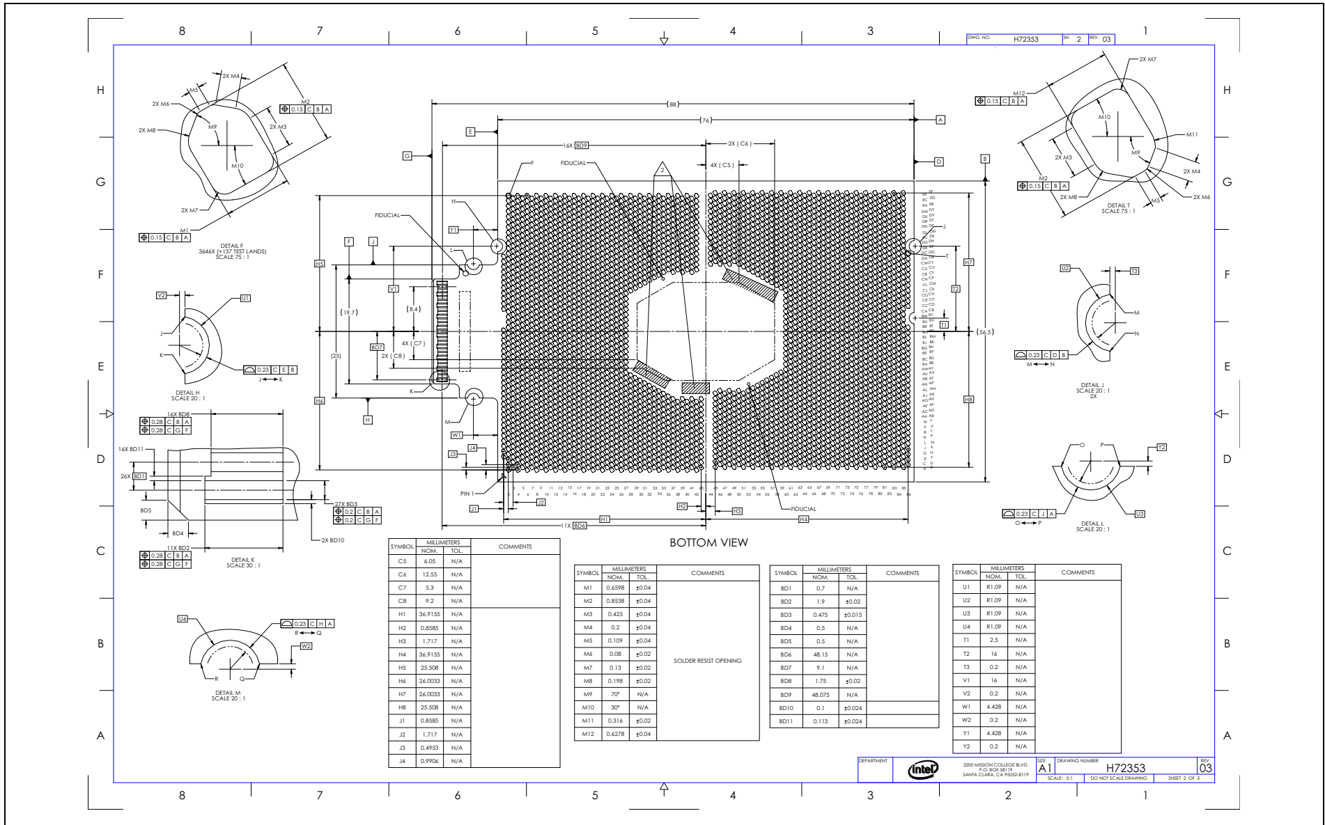
Figure B-2. PMD XCC: Fabric Form Factor (Sheet 2 of 3)
