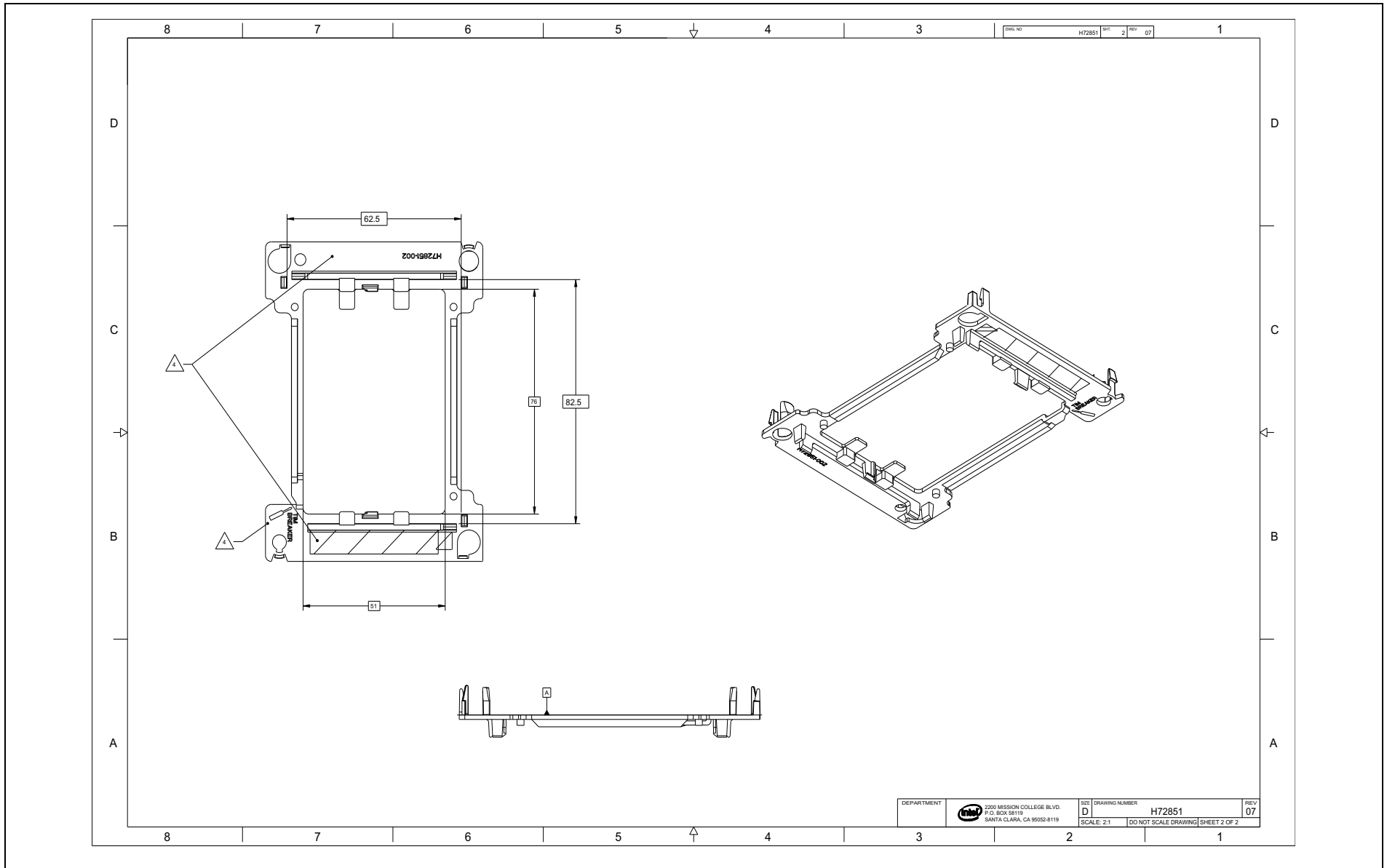
Figure D-17. Narrow CPU Carrier (Sheet 2 of 2)
