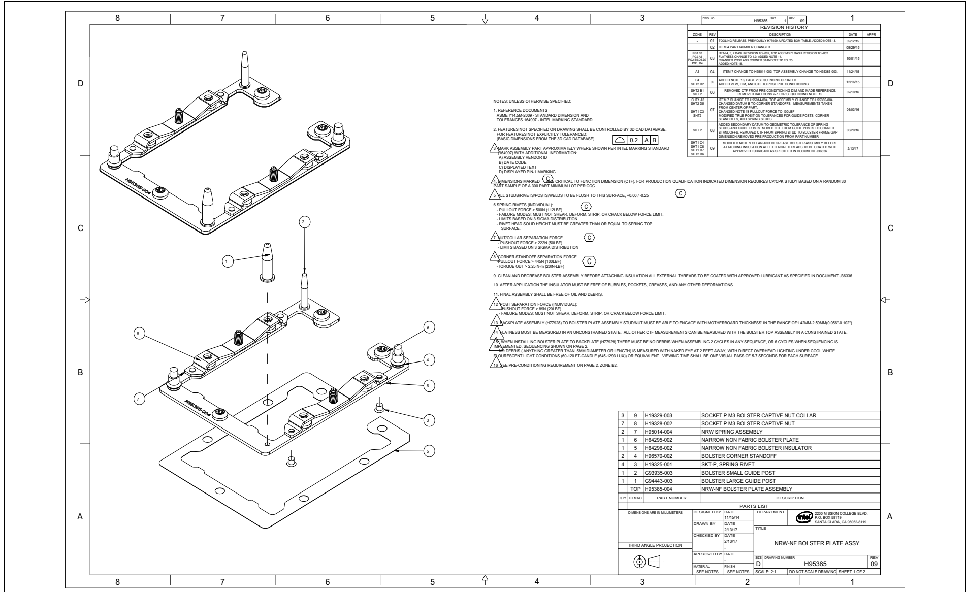
Figure D-29. Narrow Bolster Plate Assembly (Sheet 1 of 2)
