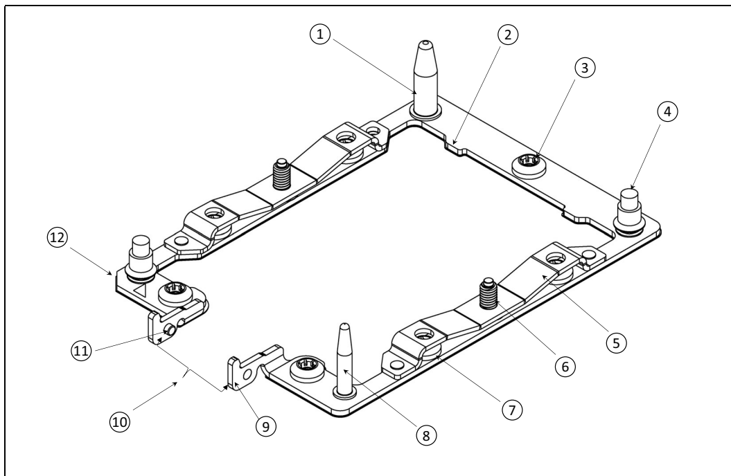
Figure 8-8. Narrow Bolster Plate Part Feature
