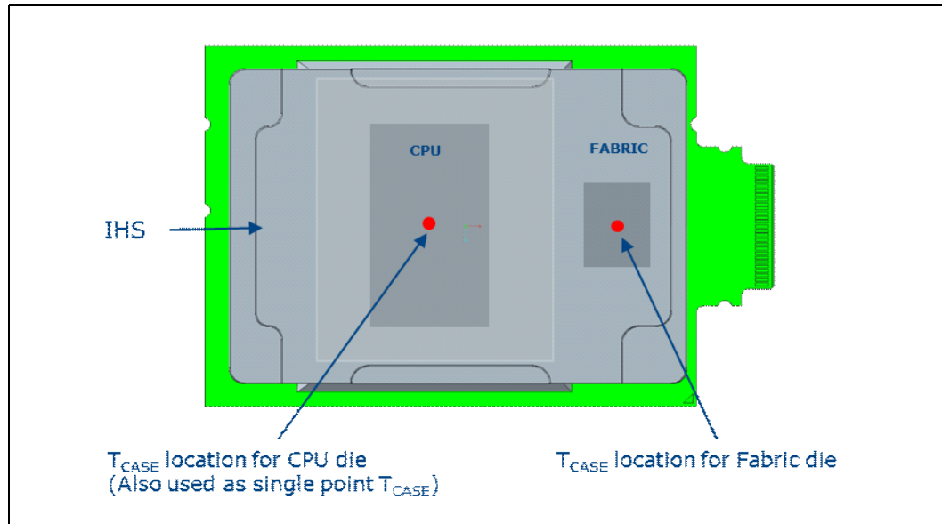
Figure 5-2. T Case Locations for an MCP
