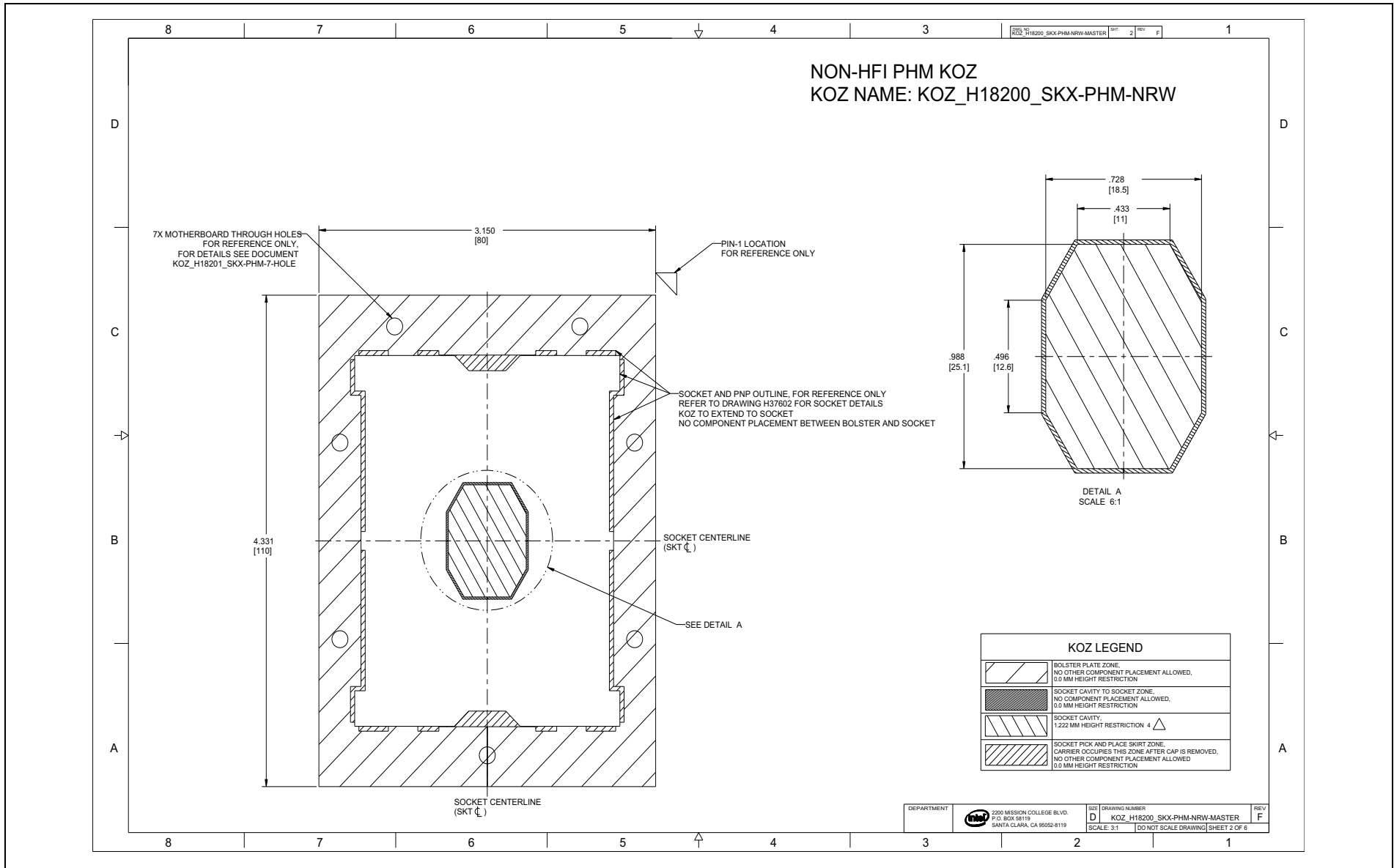
Figure F-3. KOZ: PHM Narrow Master (Sheet 2 of 6)
