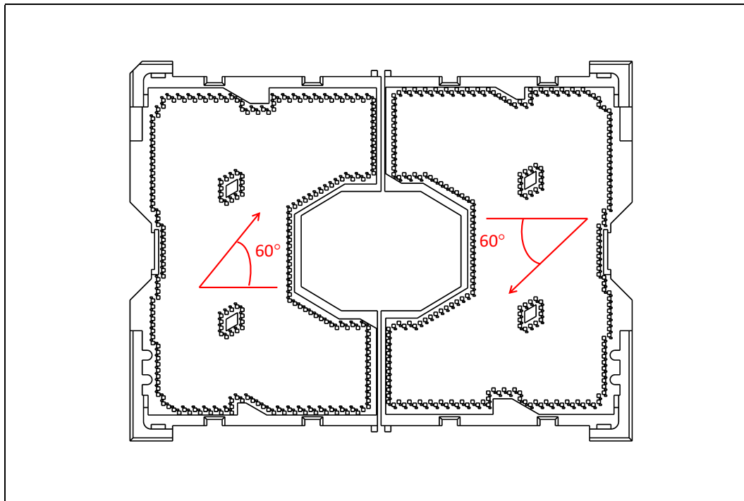
Figure 3-6. Contact Orientation
