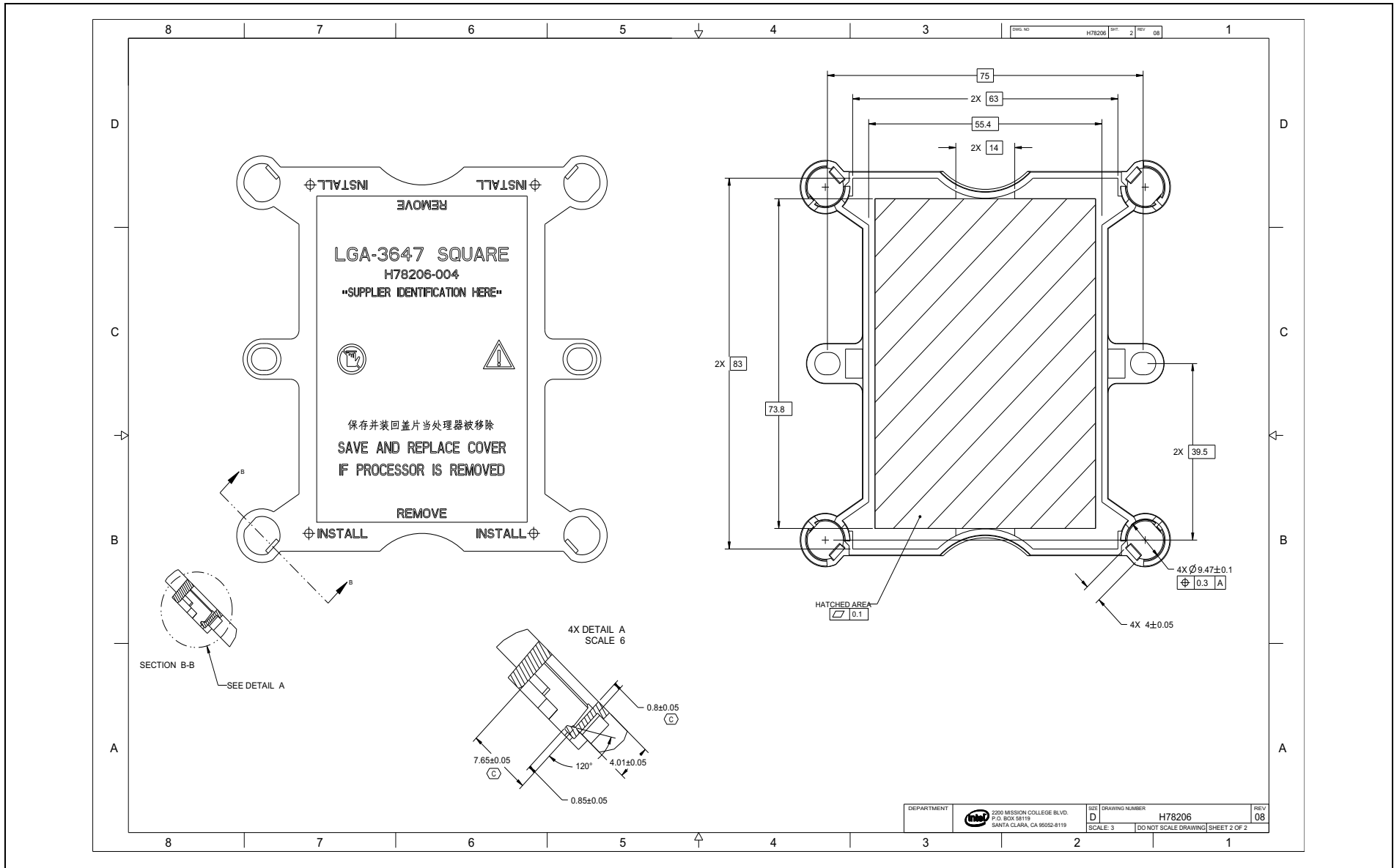
Figure D-22. Square Dust Cover (Sheet 2 of 2)
