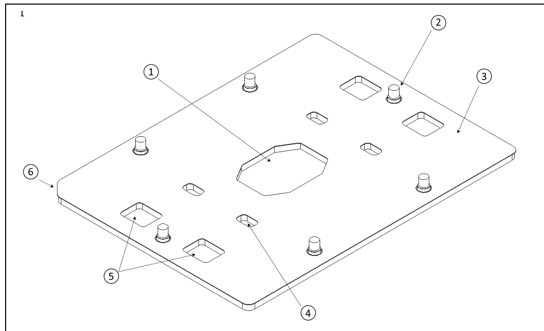
Figure 8-11. Square Back Plate Part Feature
