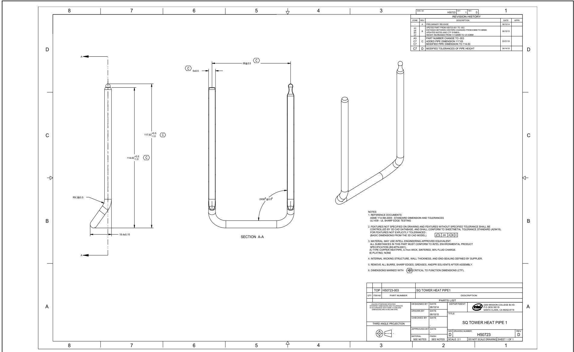
Figure E-16. Square Tower Heat Pipe 1
