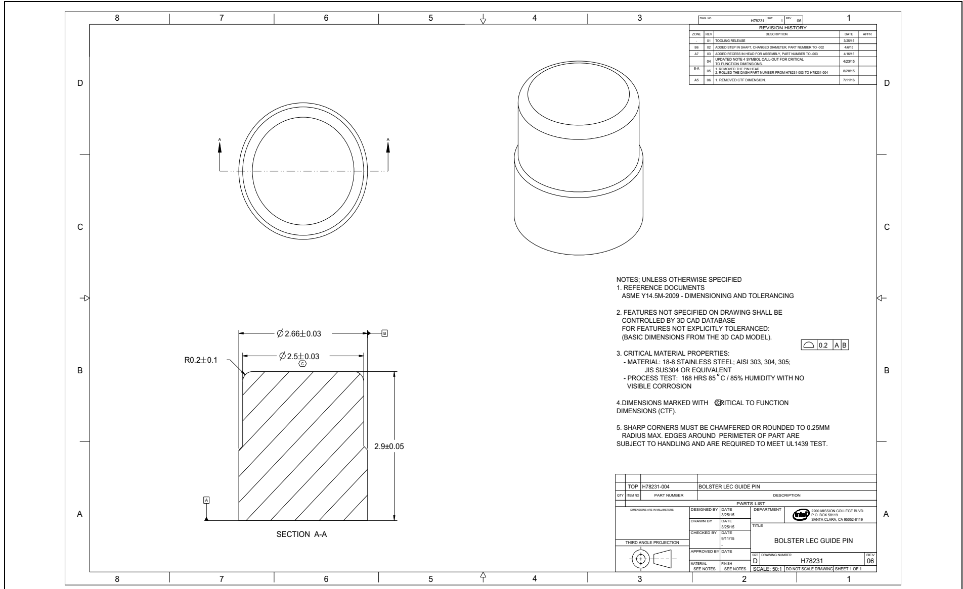
Figure D-23. Bolster LEC Guide Pin
