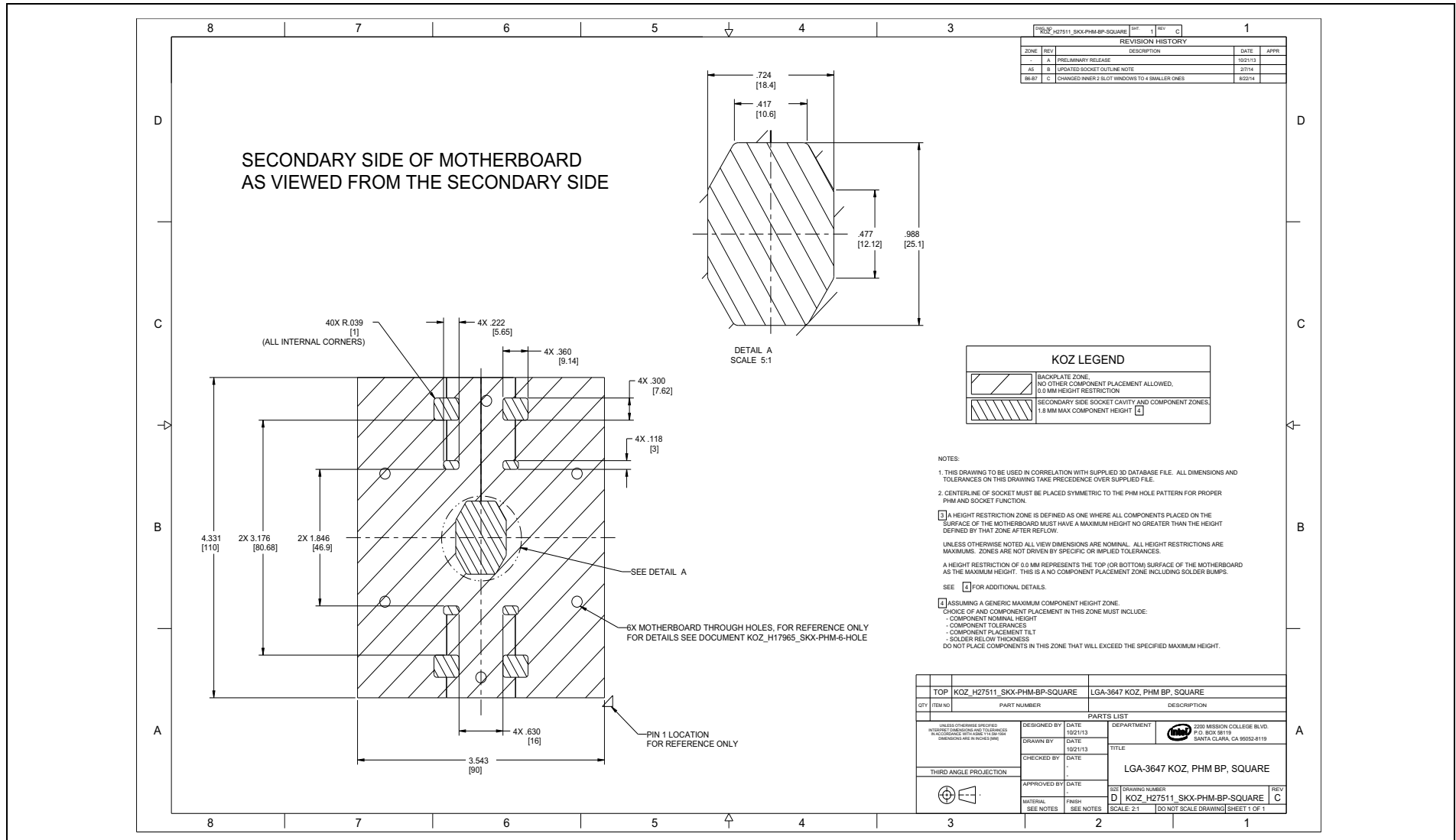
Figure F-6. KOZ:PHM Square Backplate
