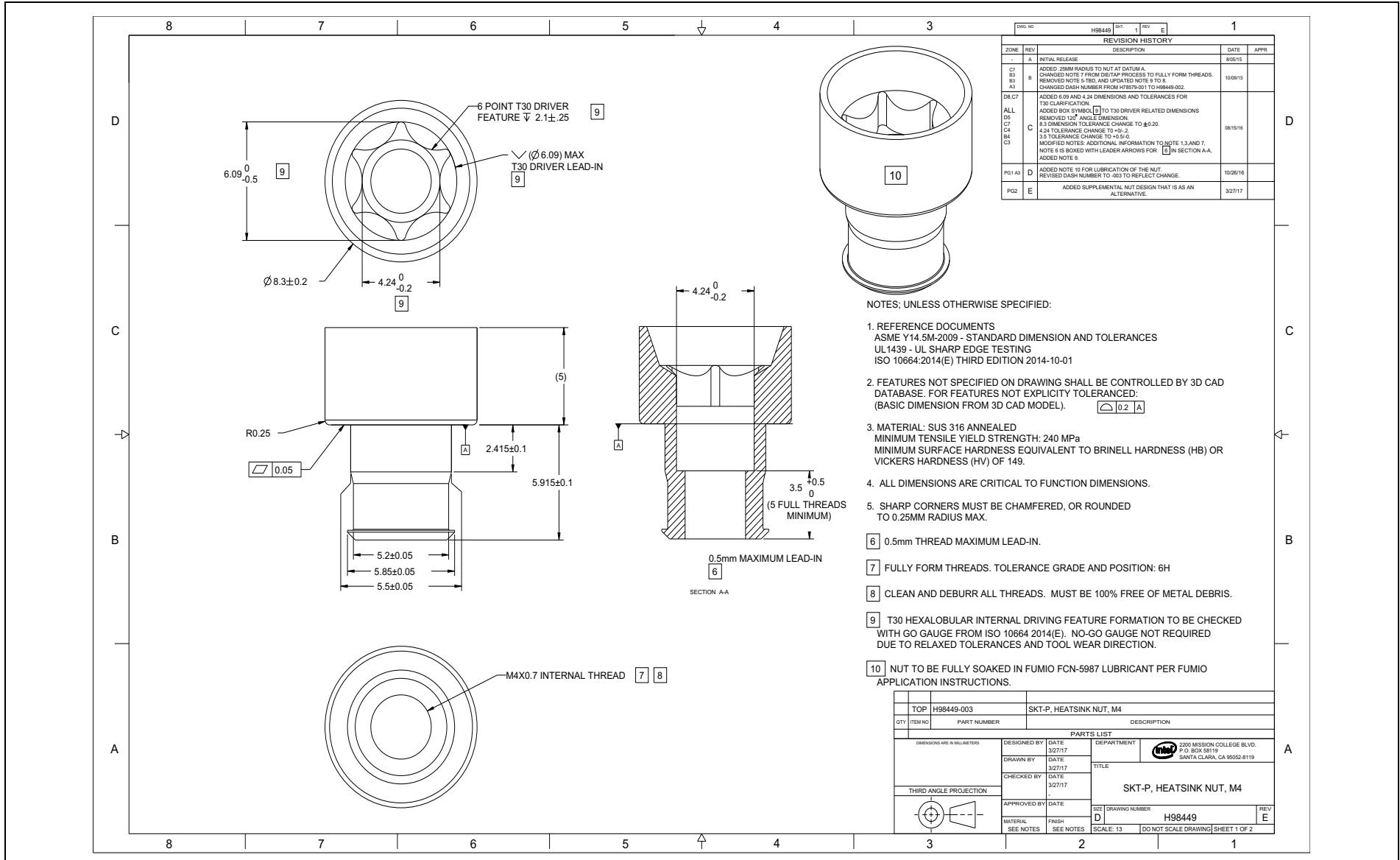
Figure E-24. Heatsink Nut (Sheet 1 of 2)
