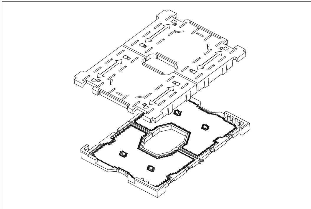
Figure 3-1. LGA3647-0 Socket with PNP Cap
