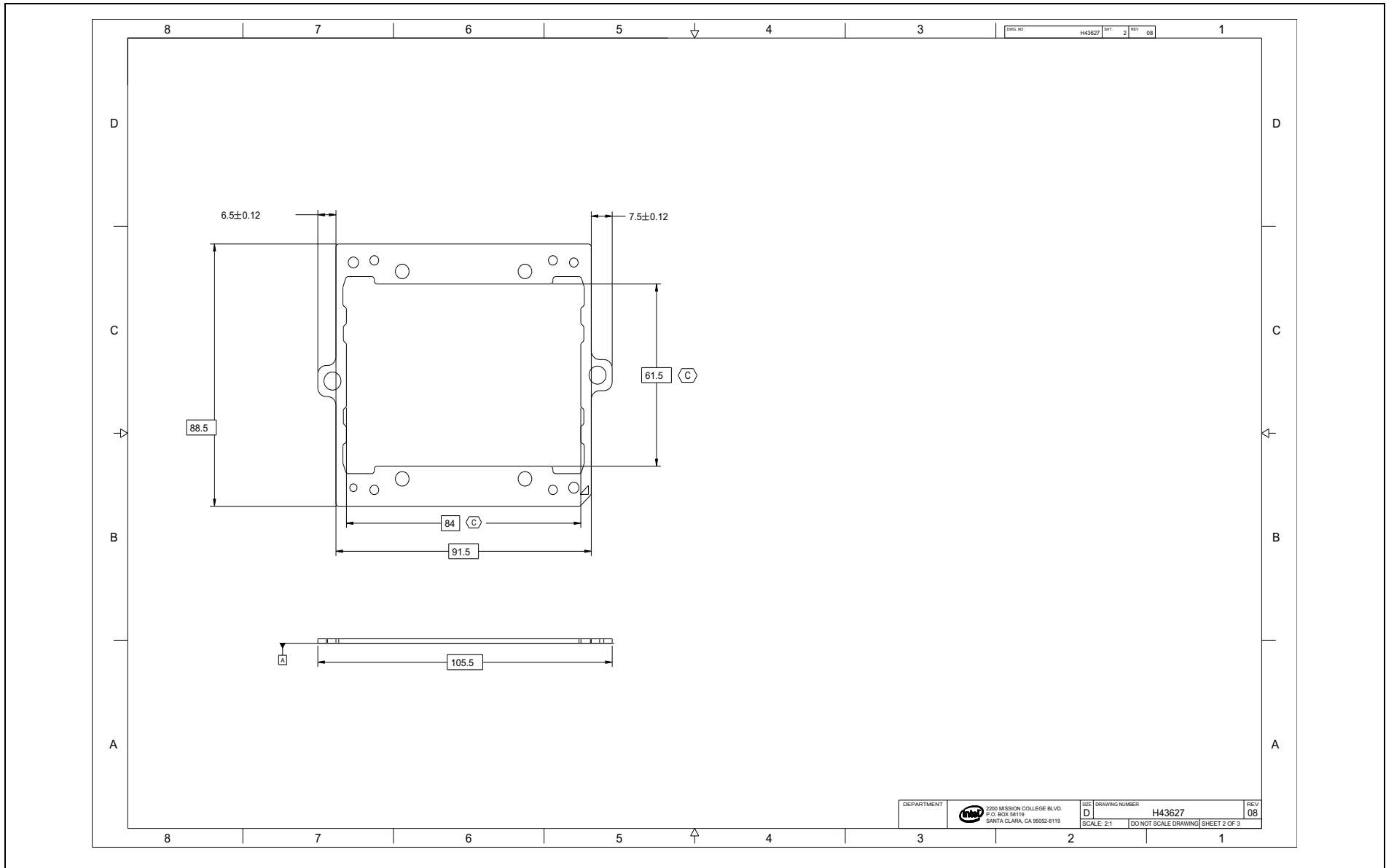
Figure D-12. Square Bolster Plate (Sheet 2 of 3)
