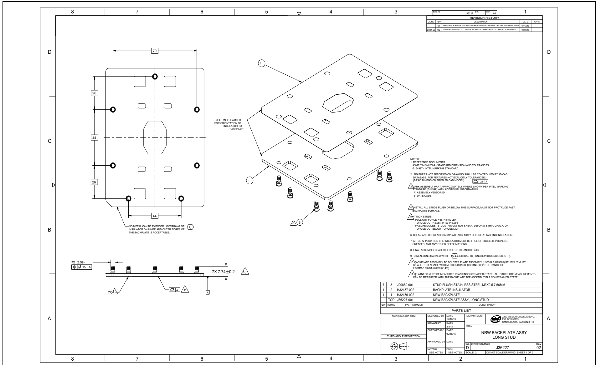
Figure D-35. Narrow Backplate Long Stud Assembly (Sheet 1 of 2)
