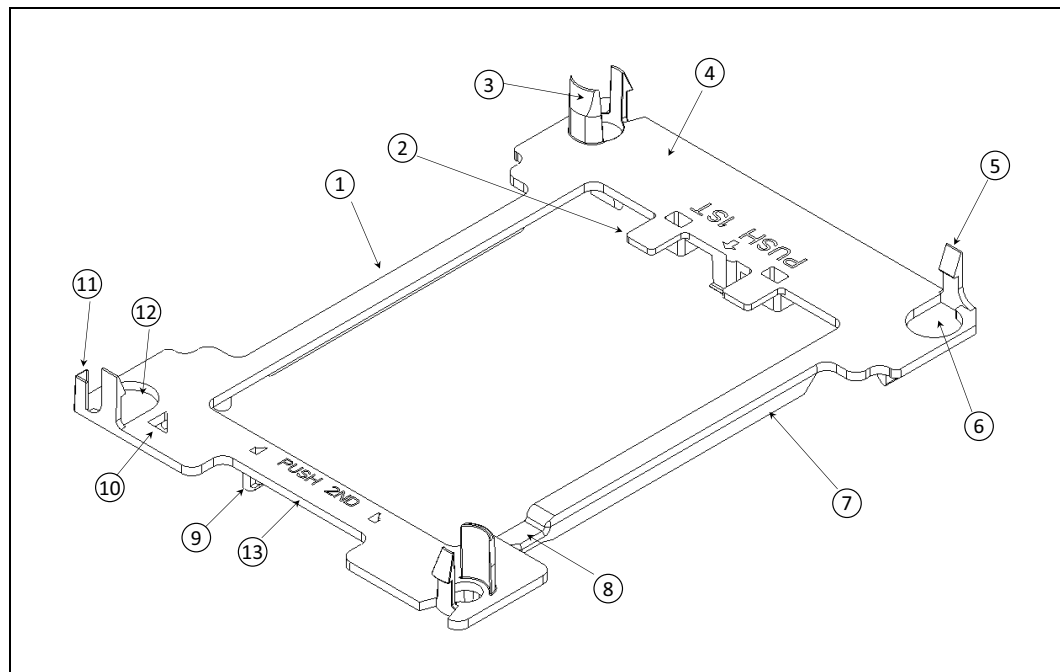
Figure 8-12. Narrow Fabric Package Carrier Mechanical Features (Top View)
