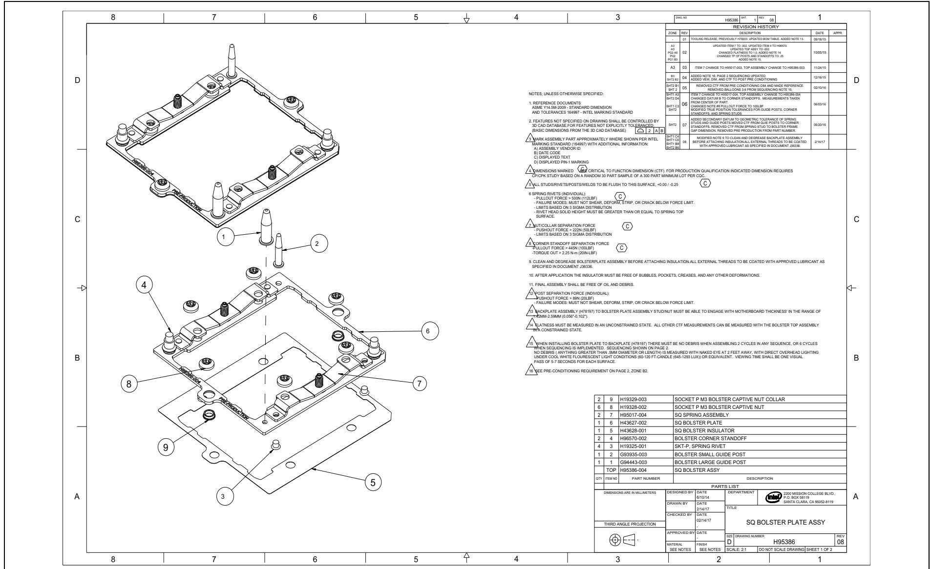
Figure D-30. Square Bolster Plate Assembly (Sheet 1 of 2)
