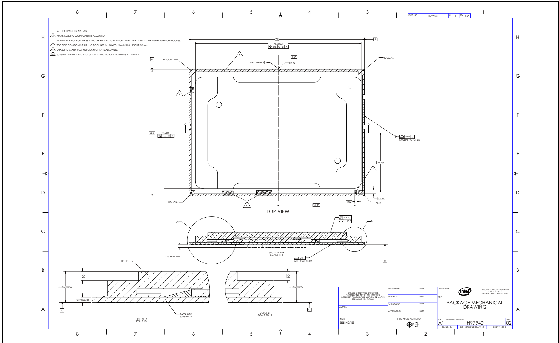
Figure B-3. PMD HCC Form Factor (Sheet 1 of 3)
