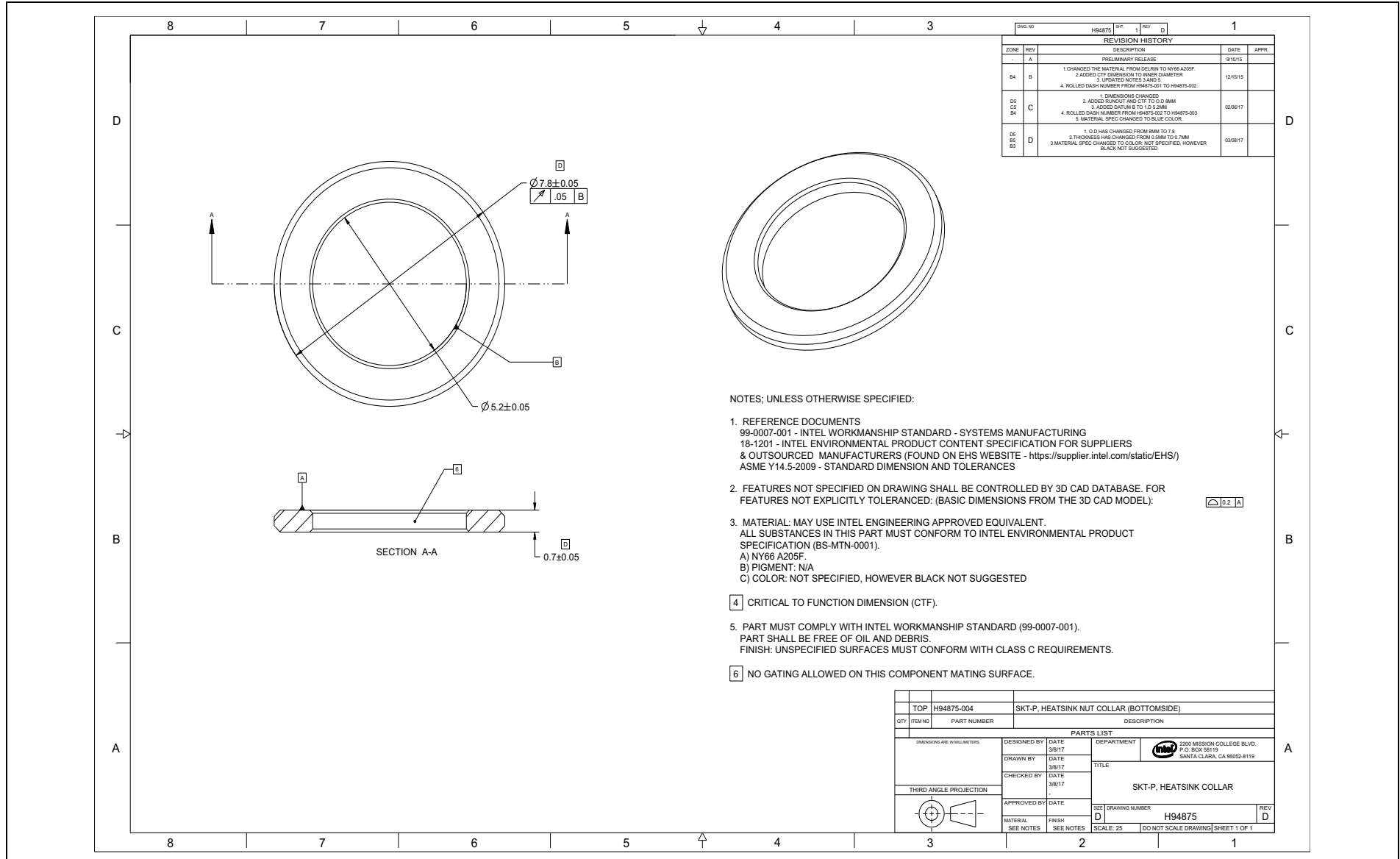
Figure E-23. Heatsink Collar
