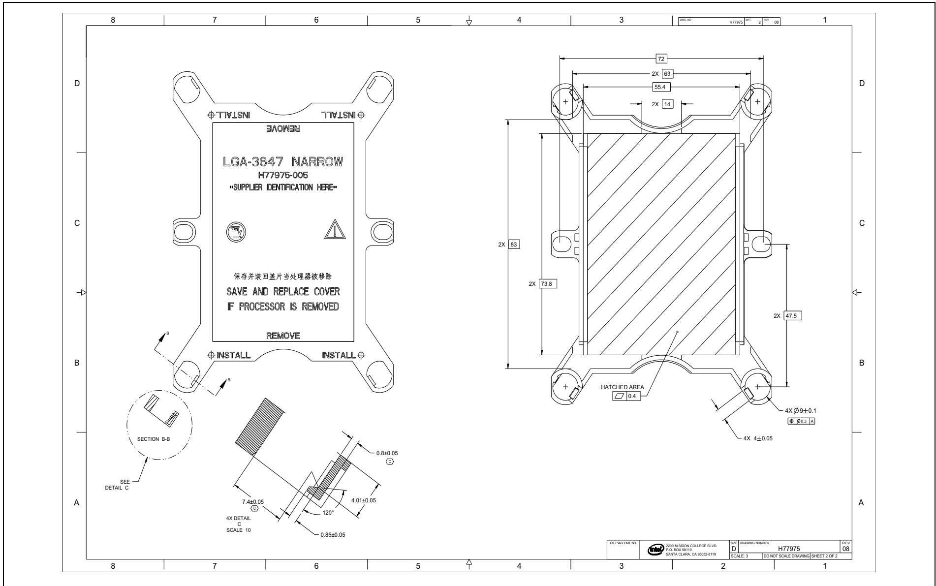
Figure D-20. Narrow Dust Cover (Sheet 2 of 2)
