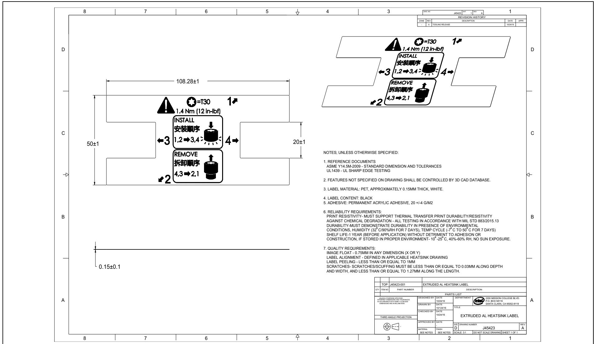
Figure E-25. Extruded Aluminum Heatsink Label
