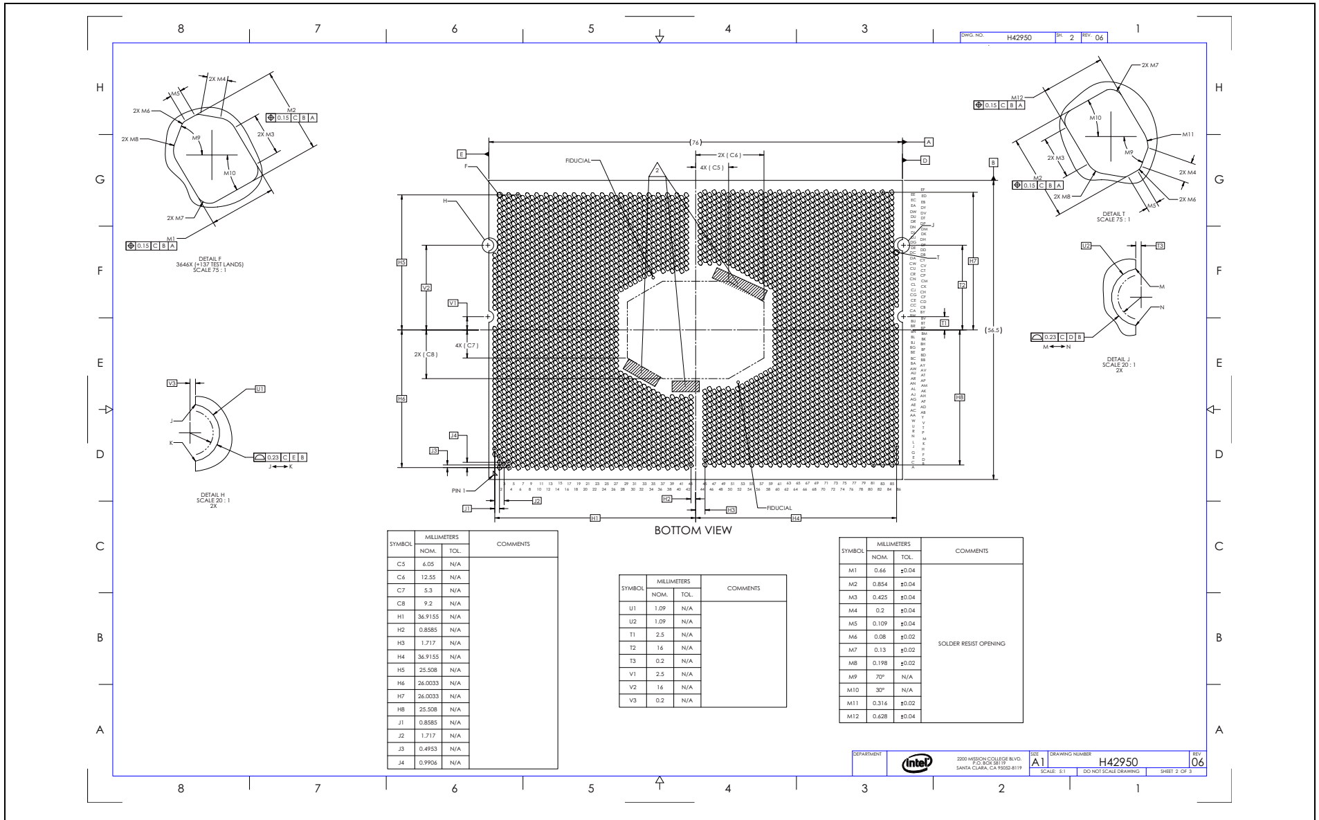
Figure B-1. PMD XCC: Non Fabric Form Factor (Sheet 2 of 3)
