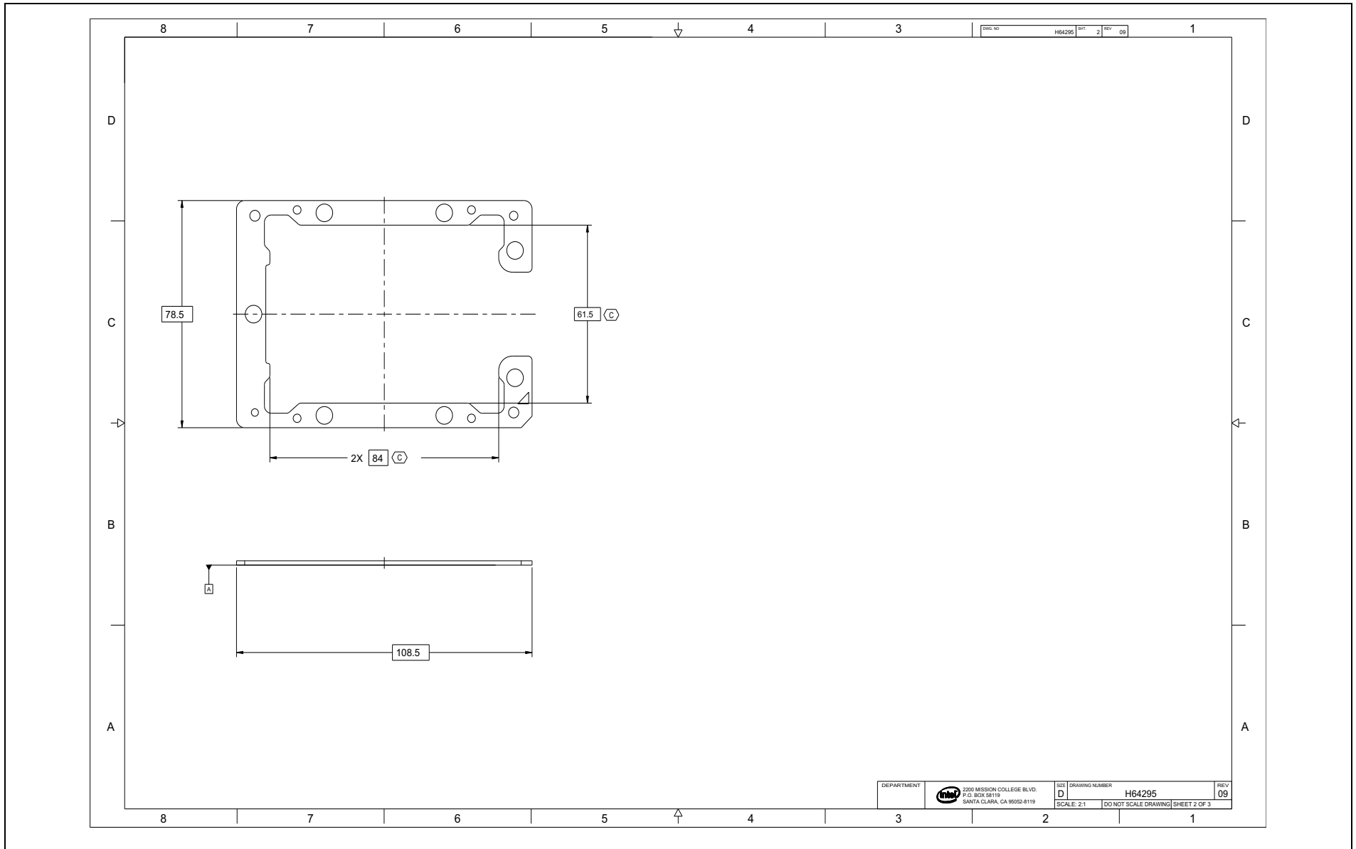
Figure D-14. Narrow Bolster Plate (Sheet 2 of 3)
