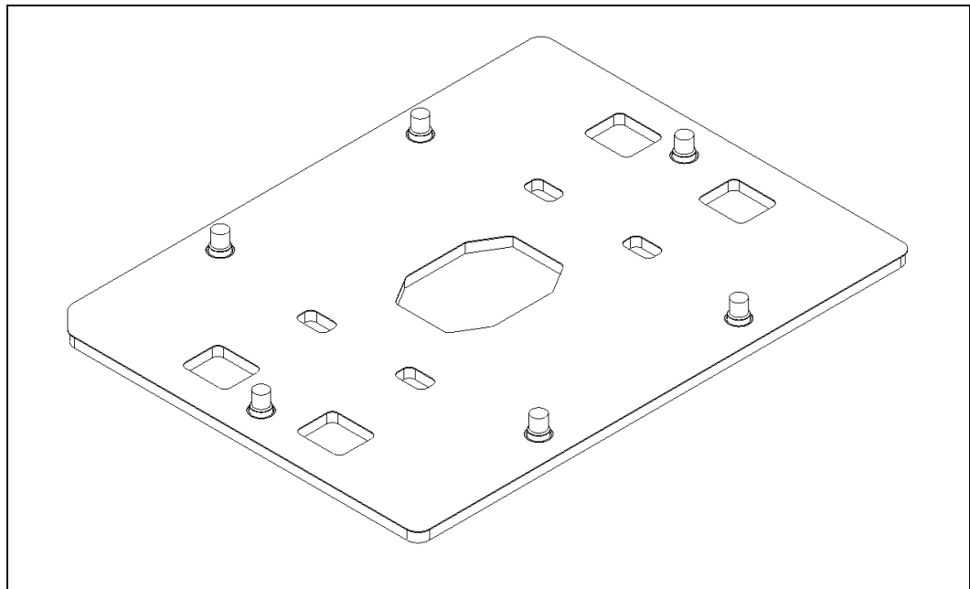
Figure 8-7. Square Back Plate (ISO View)
