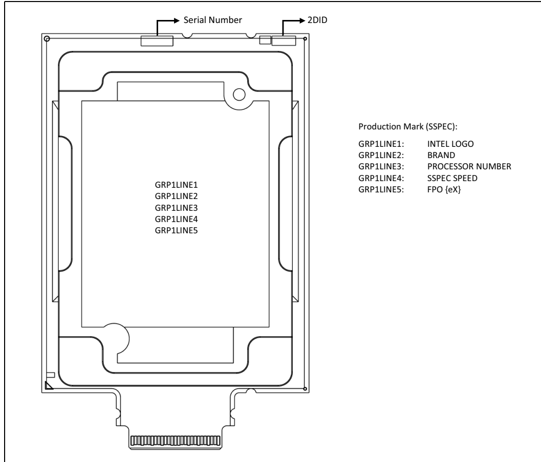
Figure 2-3. Intel® Xeon® Processor Scalable Family Package Top Side Markings
