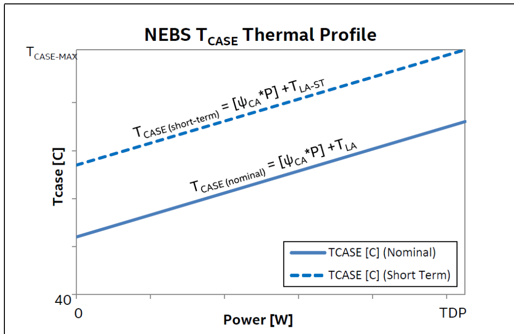
Figure 5-3. NEBS T CASE Thermal Profile
