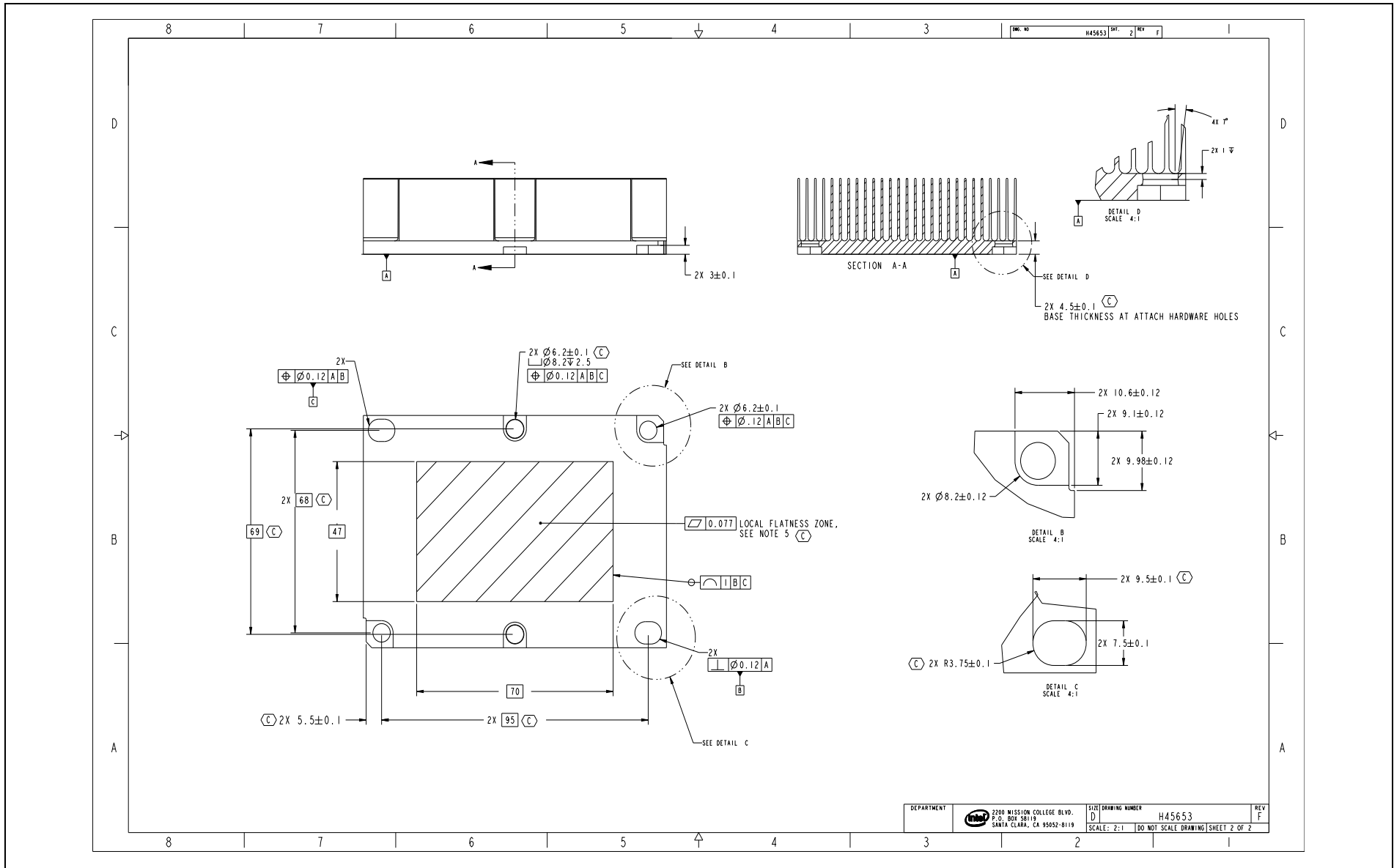
Figure E-12. 1U Extruded Heatsink (Sheet 2 of 2)
