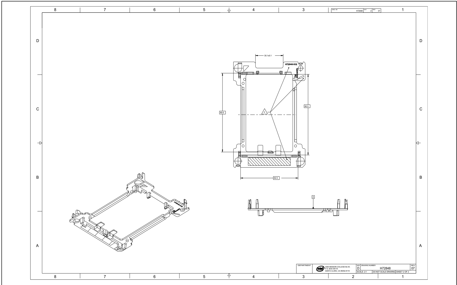
Figure D-16. Narrow-Fabric CPU Carrier (Sheet 2 of 2)
