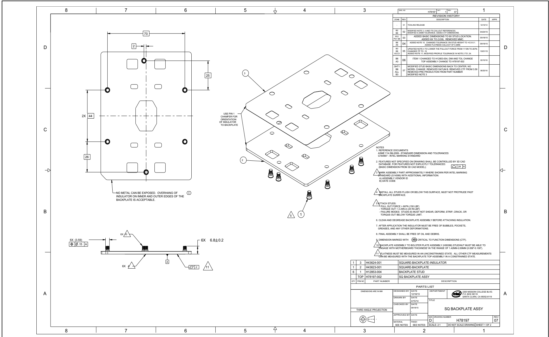
Figure D-21. Square Backplate Assembly (Sheet 1 of 2)
