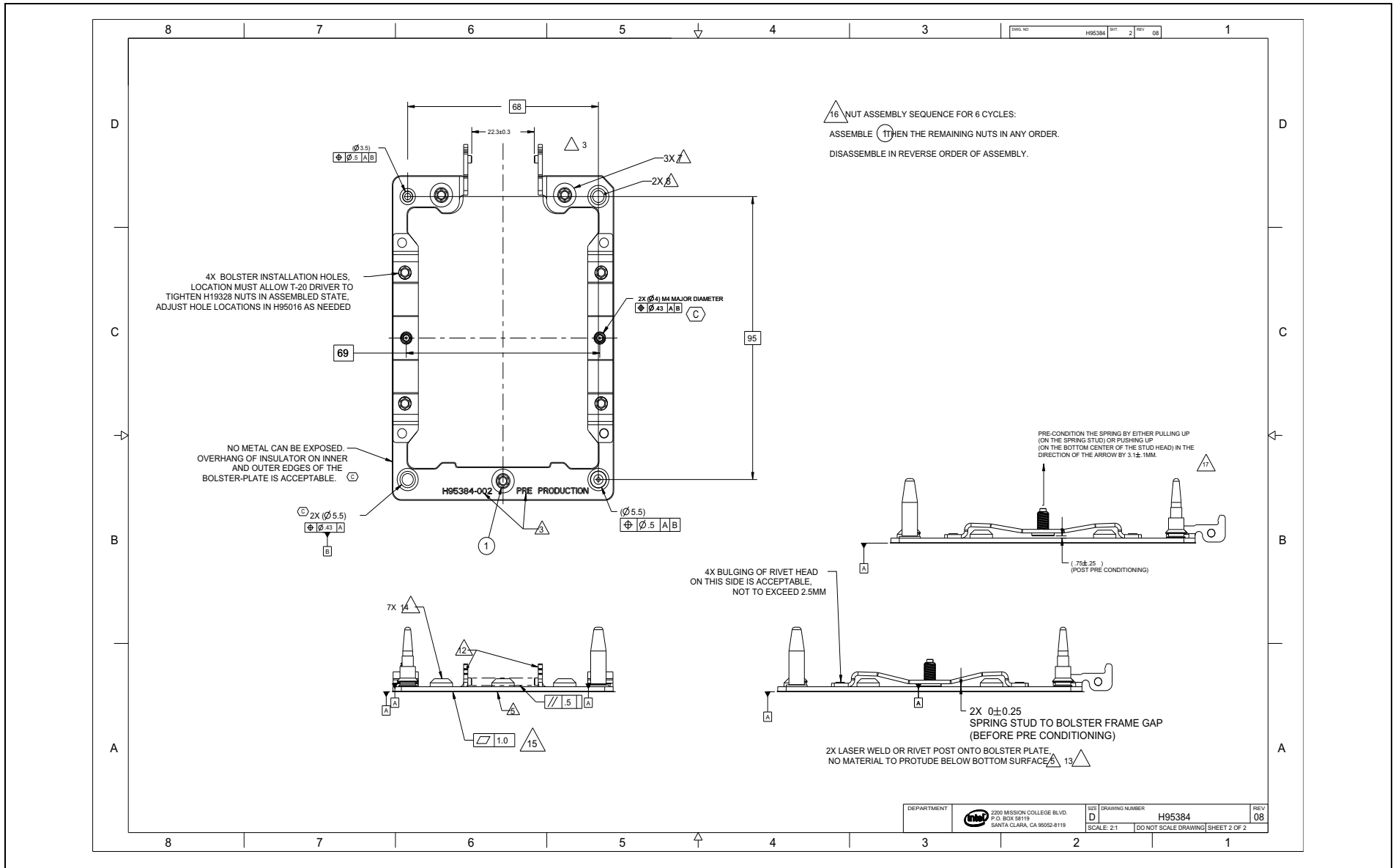
Figure D-28. Narrow - Fabric Bolster Plate Assembly (Sheet 2 of 2)
