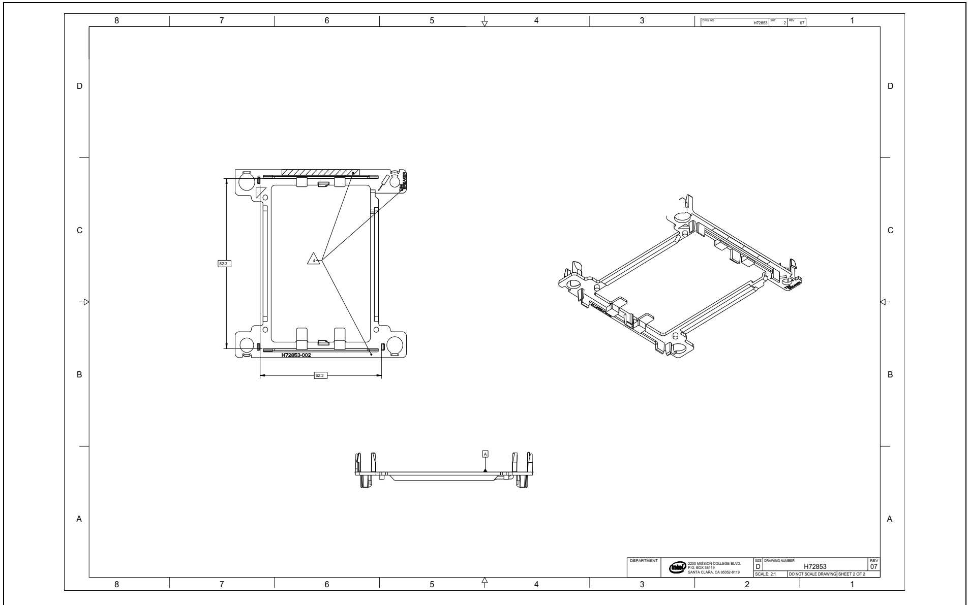
Figure D-18. Square CPU Carrier (Sheet 2 of 2)
