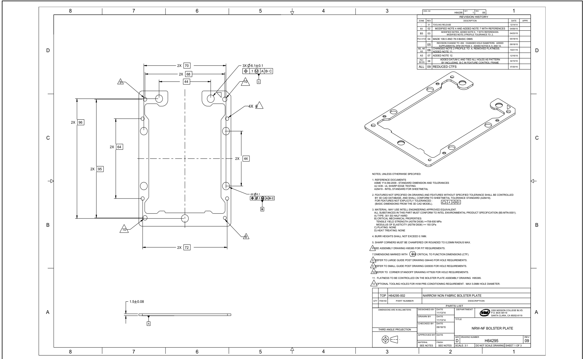
Figure D-14. Narrow Bolster Plate (Sheet 1 of 3)
