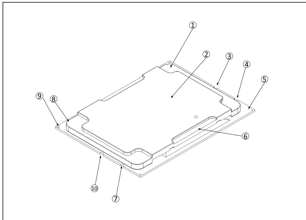
Figure 2-2. Processor without Fabric Package Assembly - ISO View
