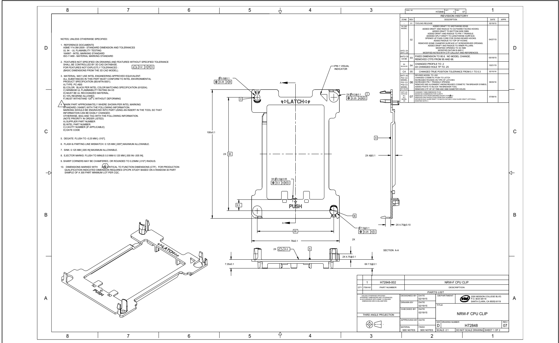
Figure D-16. Narrow-Fabric CPU Carrier (Sheet 1 of 2)
