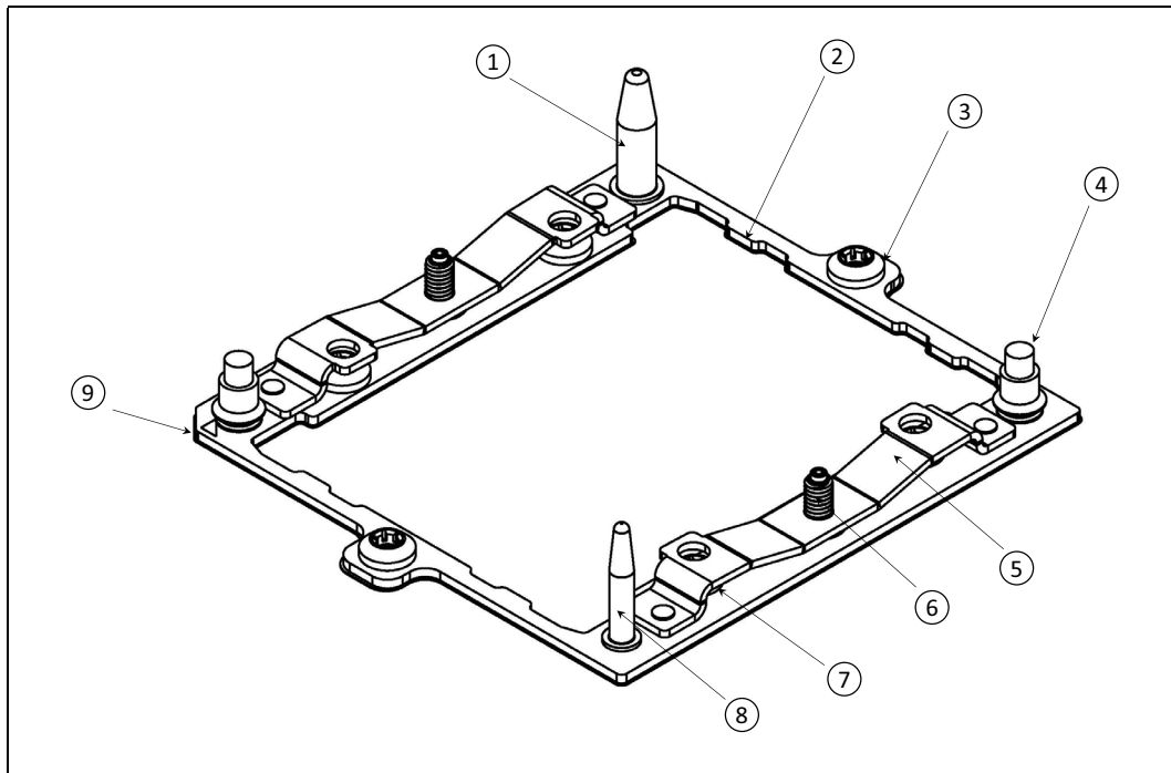
Figure 8-10. Square Bolster Plate Part Feature
