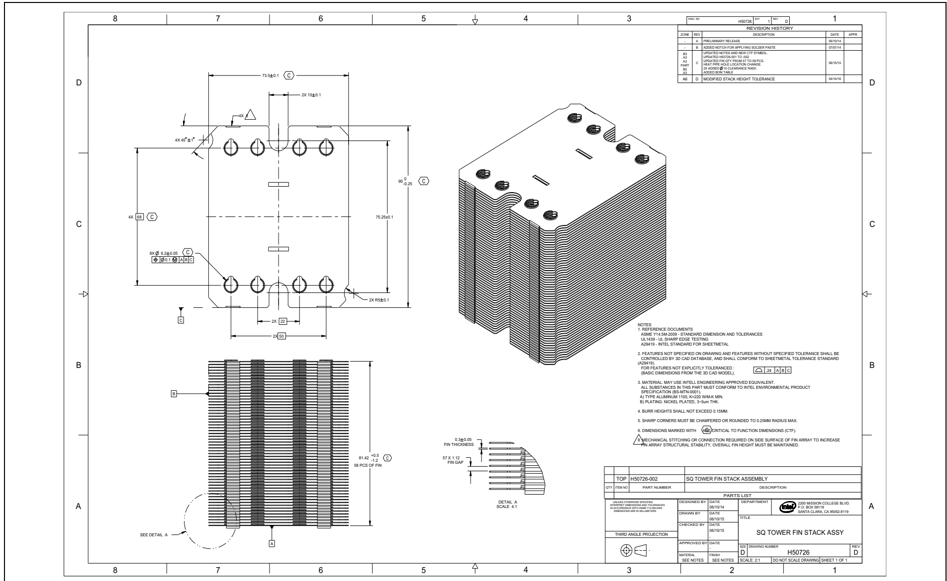
Figure E-18. Square Tower Fin Stack Assembly
