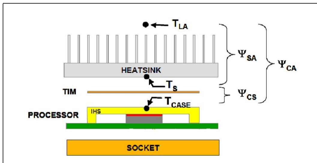
Figure 7-1. Thermal Characterization Parameters
