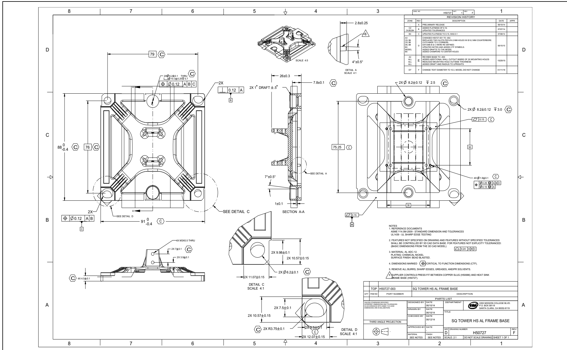
Figure E-19. Square Tower Heatsink Aluminum Frame Base
