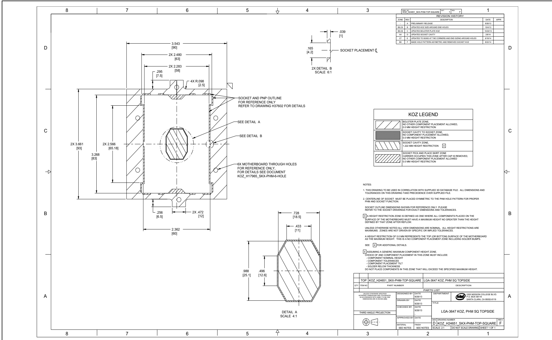
Figure F-5. KOZ: PHM Square Top
