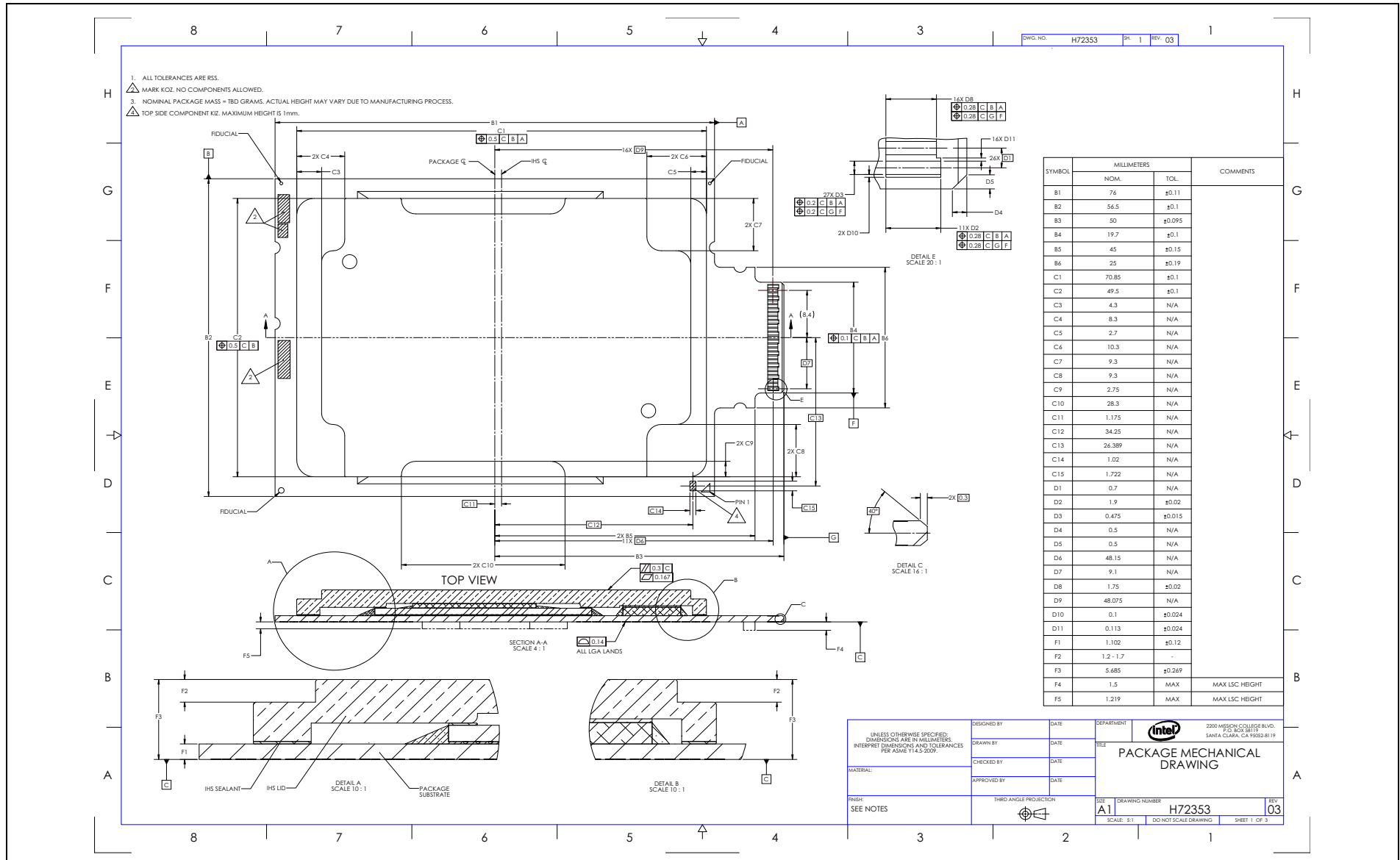
Figure B-2. PMD XCC: Fabric Form Factor (Sheet 1 of 3)
