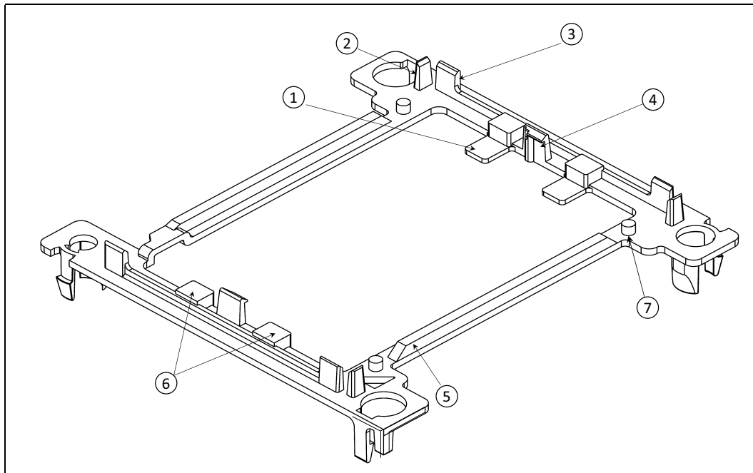
Figure 8-17. Square Package Carrier (Bottom View)
