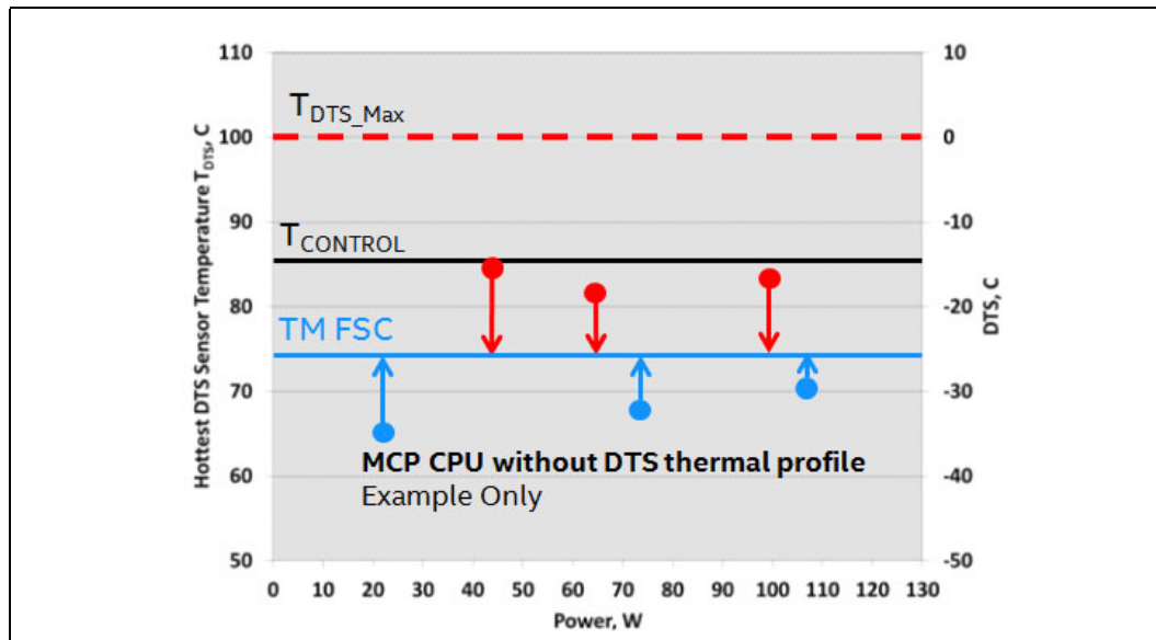
Figure 5-7. Thermal Margin to FSC Spec on Intel® Xeon® Processor Scalable Family (MCP)
