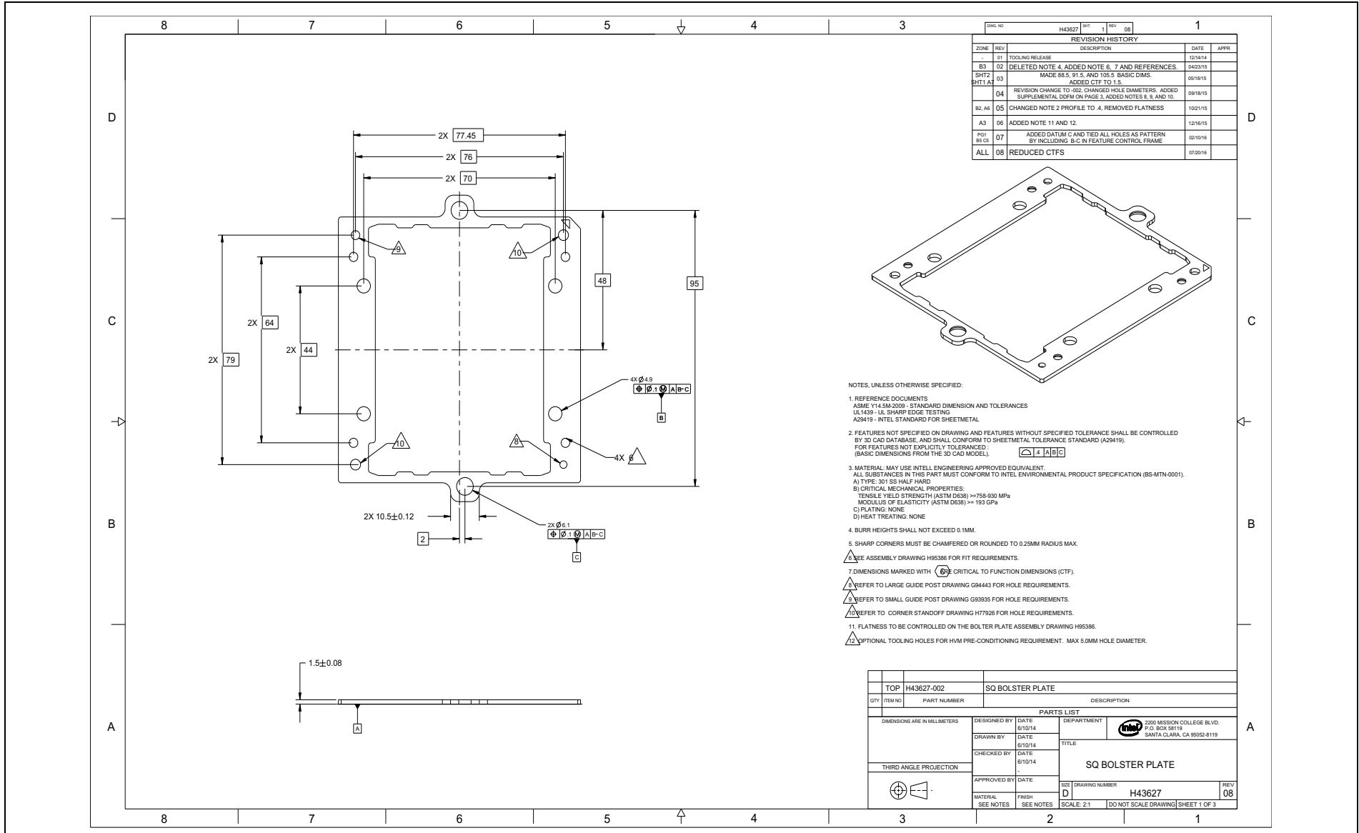
Figure D-12. Square Bolster Plate (Sheet 1 of 3)
