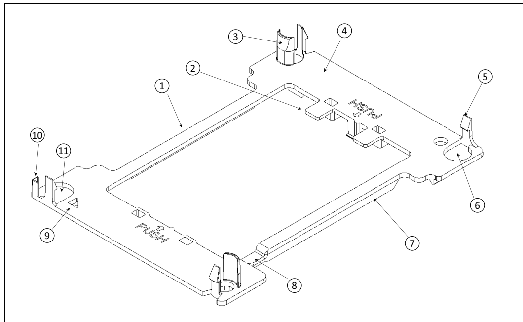
Figure 8-14. Narrow Non-Fabric Package Carrier Mechanical Features (Top View)
