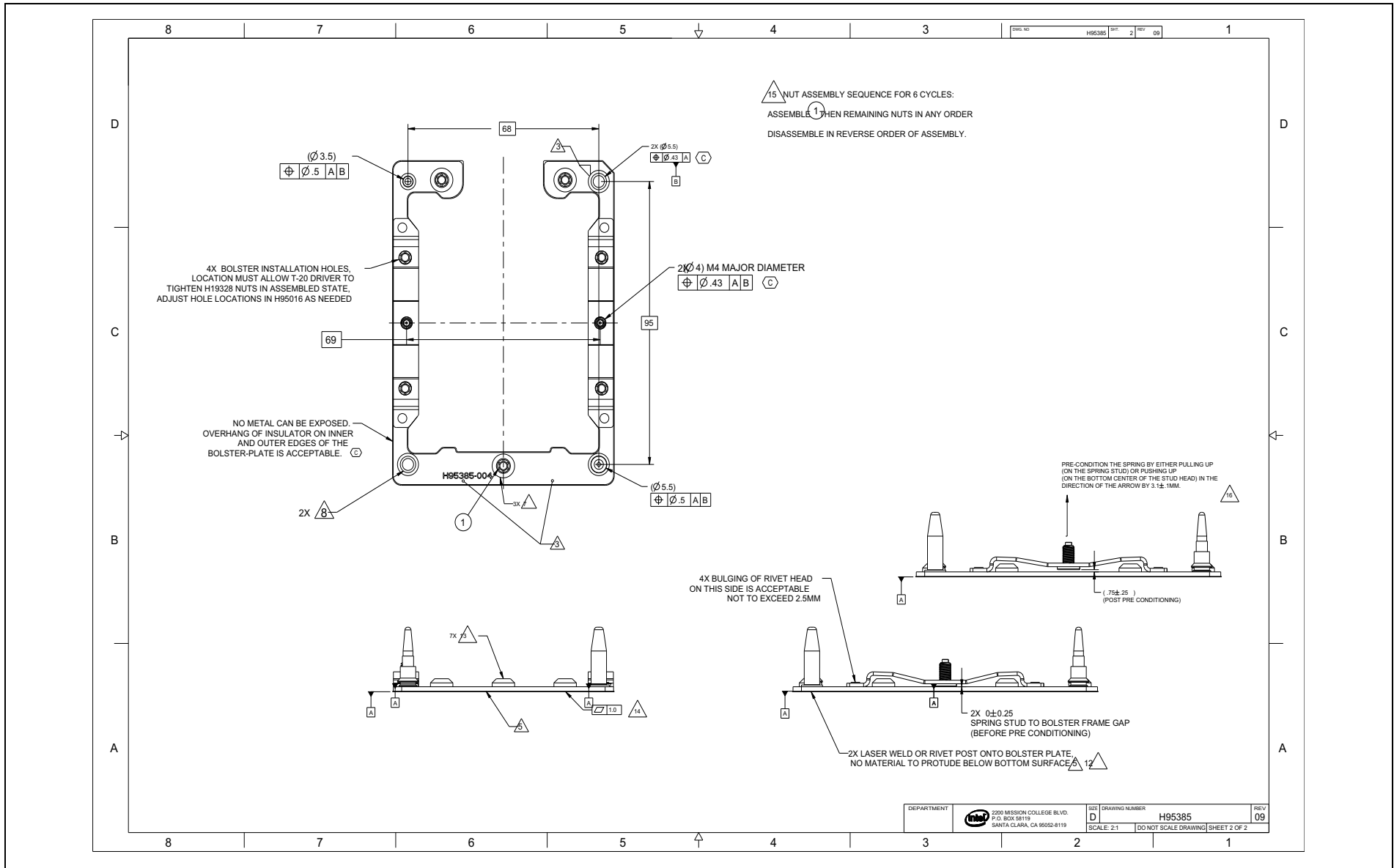
Figure D-29. Narrow Bolster Plate Assembly (Sheet 2 of 2)
