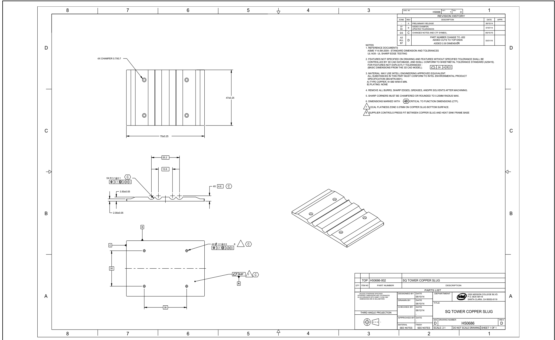
Figure E-15. Square Tower Copper Slug
