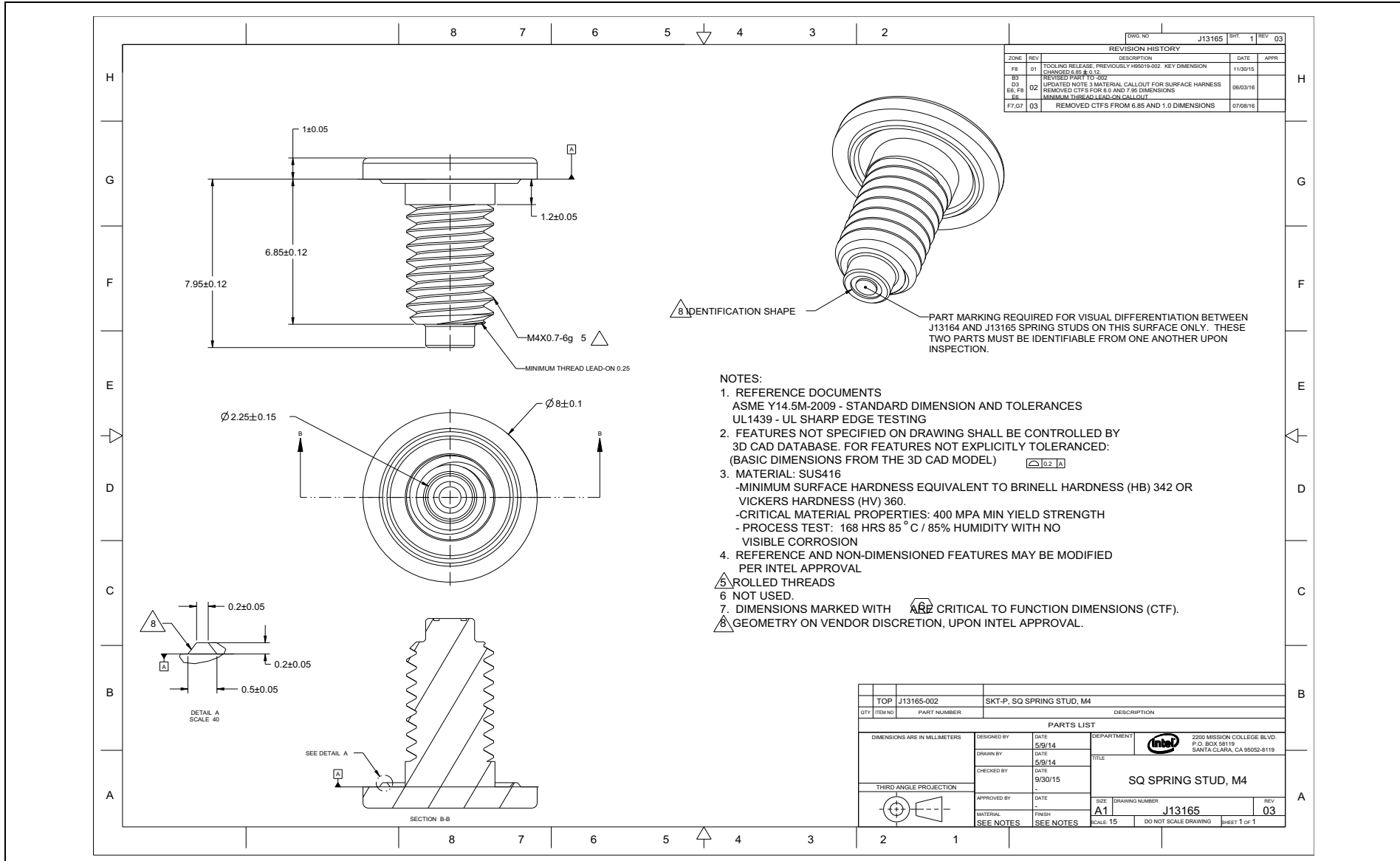
Figure D-33. Square Spring Stud
