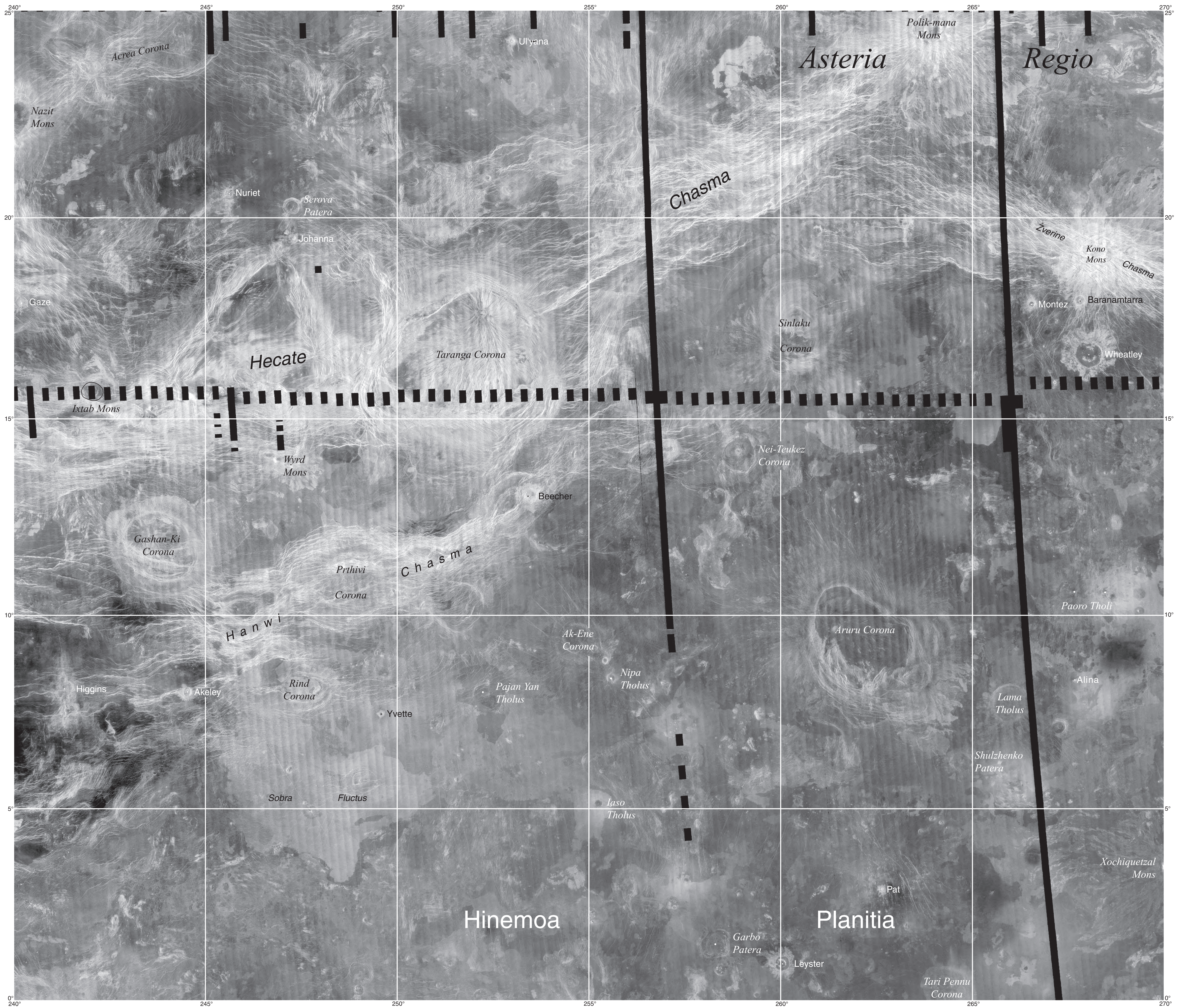
Hecate Chasma, V-28 Mercator projection
