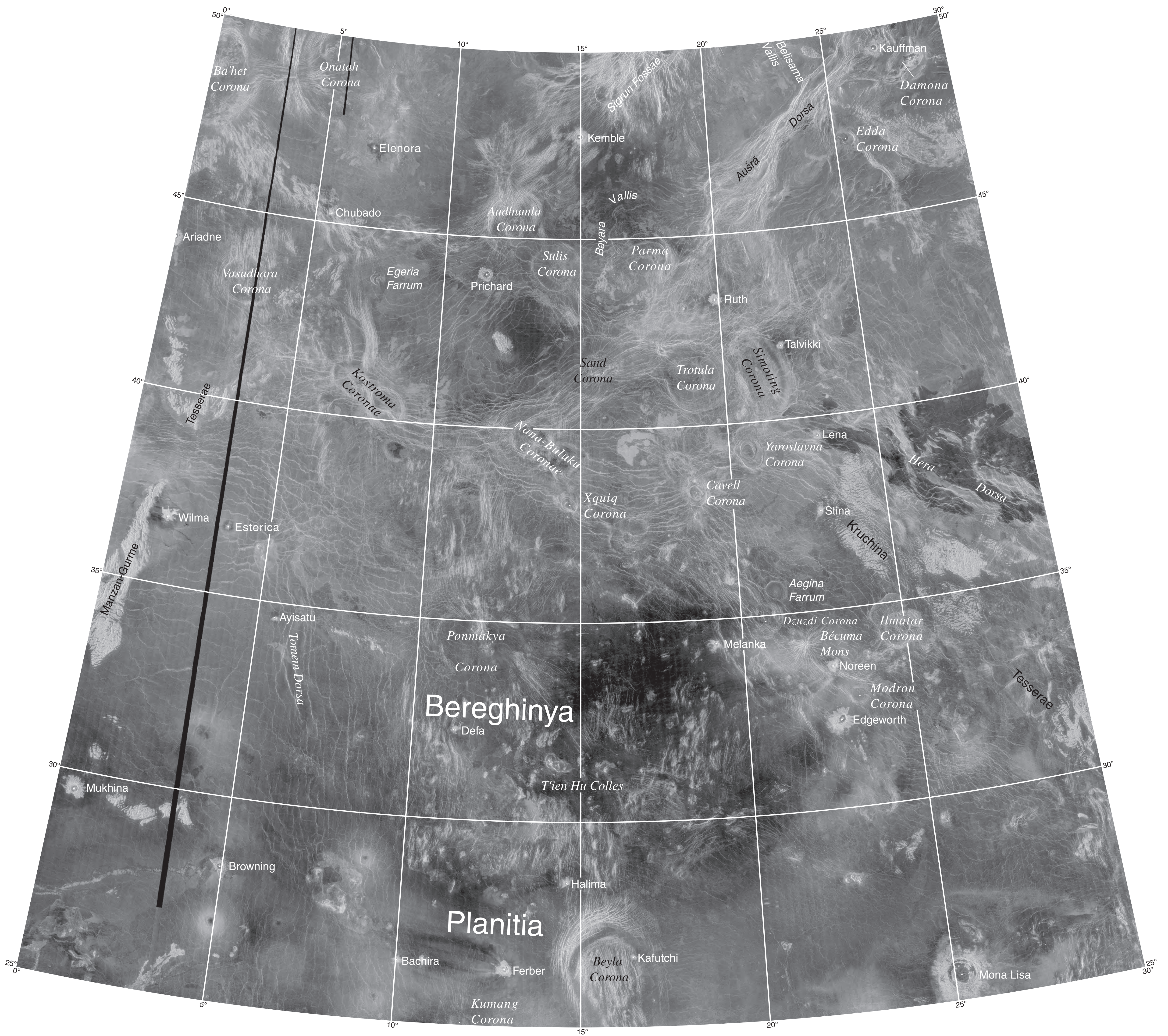
Bereghinya Planitia, V-8 Lambert projection
