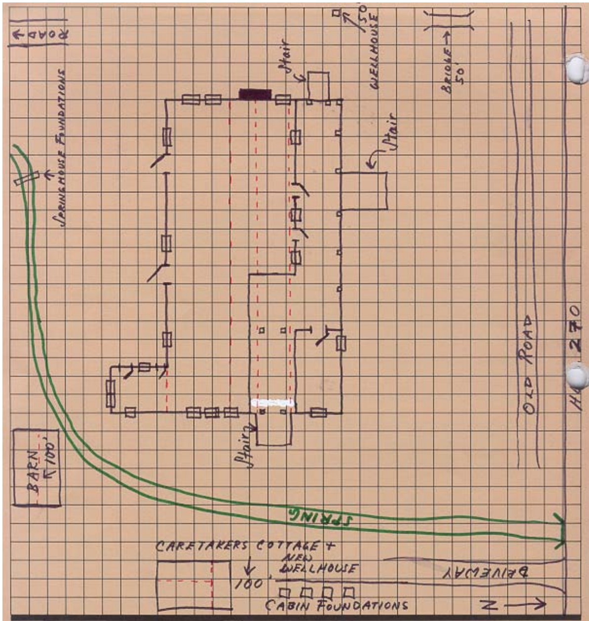
Figure 38: Mayberry Springs/Rector House Site Plan, Crystal Springs vic., Garland County. AHPP Survey Files.
