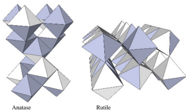
Fig. 3 Three-dimensional representation of the arrangement of TiO 6 octahedra in anatase and rutile showing 4 edge sharing connectivity in anatase and 2 edge sharing connectivity in rutile
