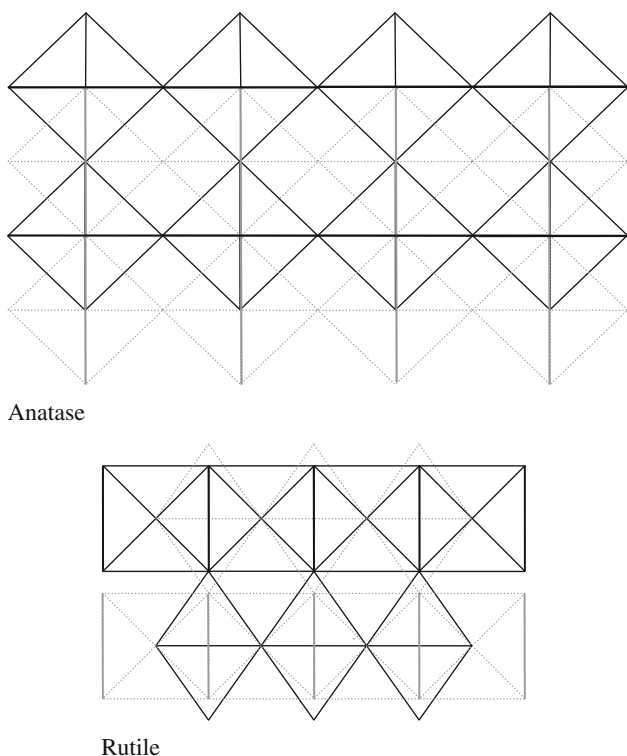
Fig. 4 Two-dimensional projection, down the c -axis, of the TiO 6 octahedra in anatase and rutile; shared edges in bold lines
