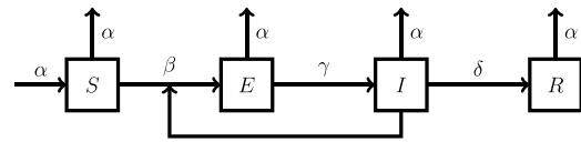
Fig. 5. Flowchart of the SEIR model with vital dynamics.
