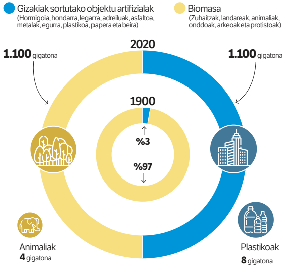
ITURRIA: GLOBAL HUMAN-MADE MASS EXCEEDS LIVING BIOMASS
