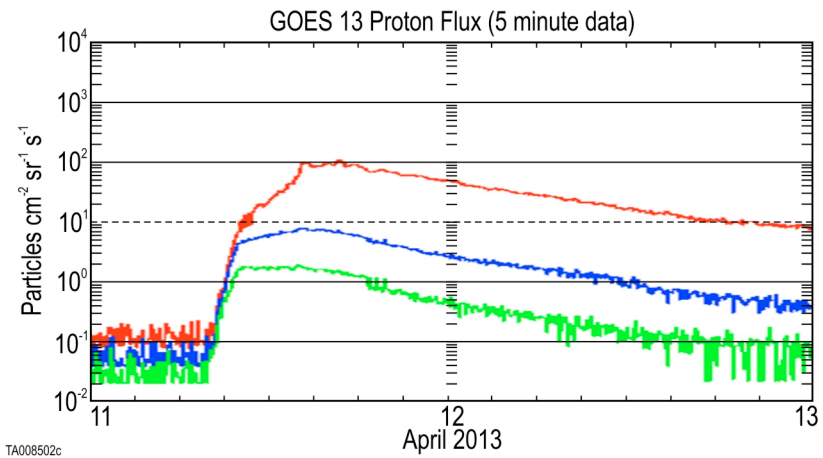
Figure 5. a) Dose rate enhancement from a solar energetic particle (SEP) event observed on the Martian surface by RAD on Sol 242 (11-12 April 2013), while Mars was in solar conjunction. b) the same SEP event seen from the STEREO-B spacecraft, almost magnetically aligned with Mars, and c) The same SEP event seen by the GOES-13 satellite in earth orbit, almost 180 degrees away in heliospheric longitude.
