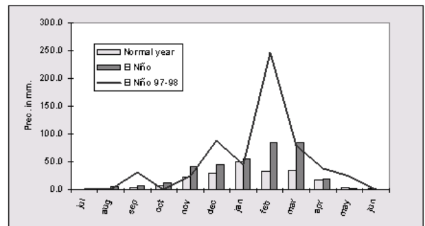
Fig. 2. Comparison of rainfalls at La Presa Rodríguez.
