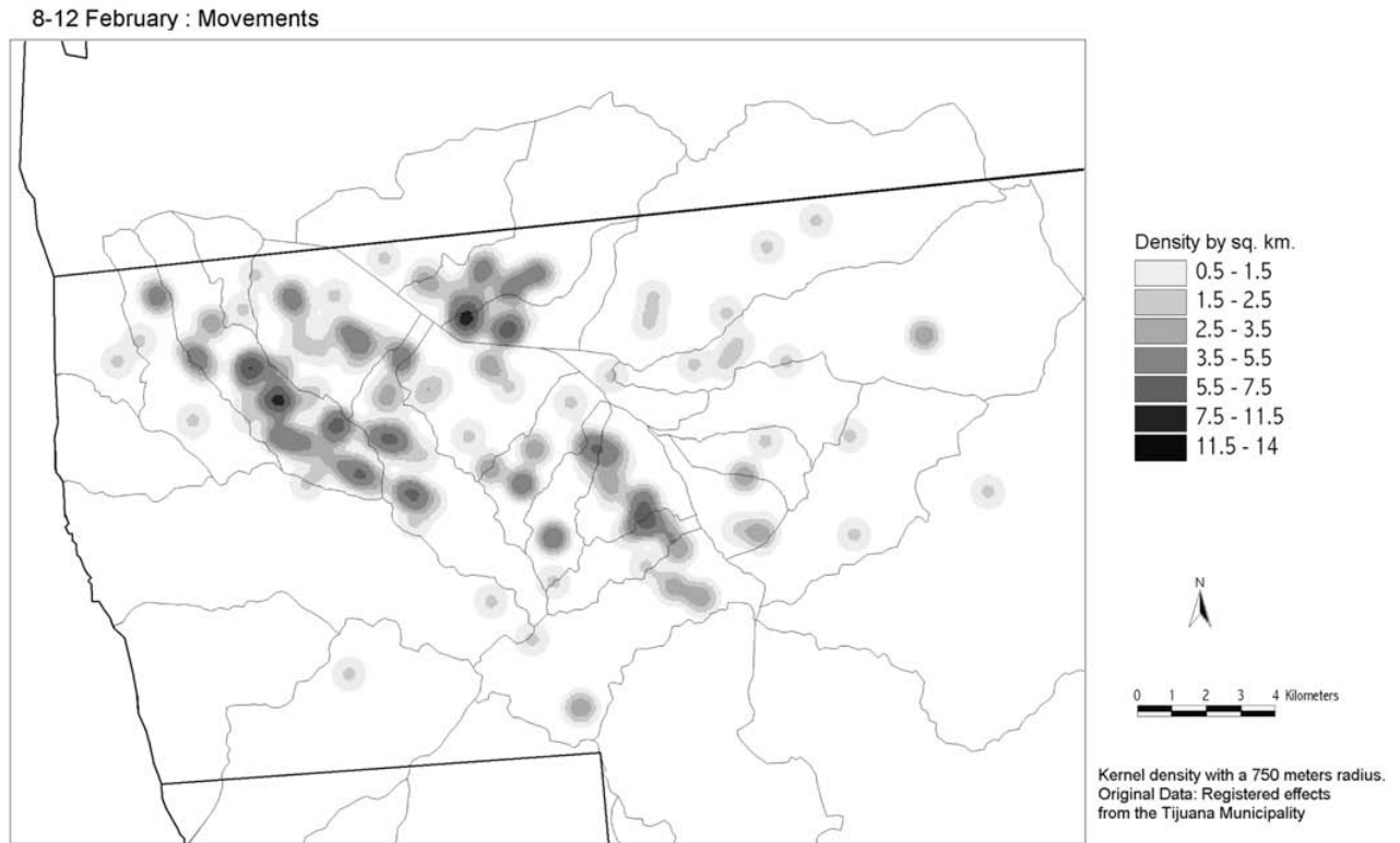
Fig. 7. Events of slope dynamics between 8 and 12 February, 1998.
