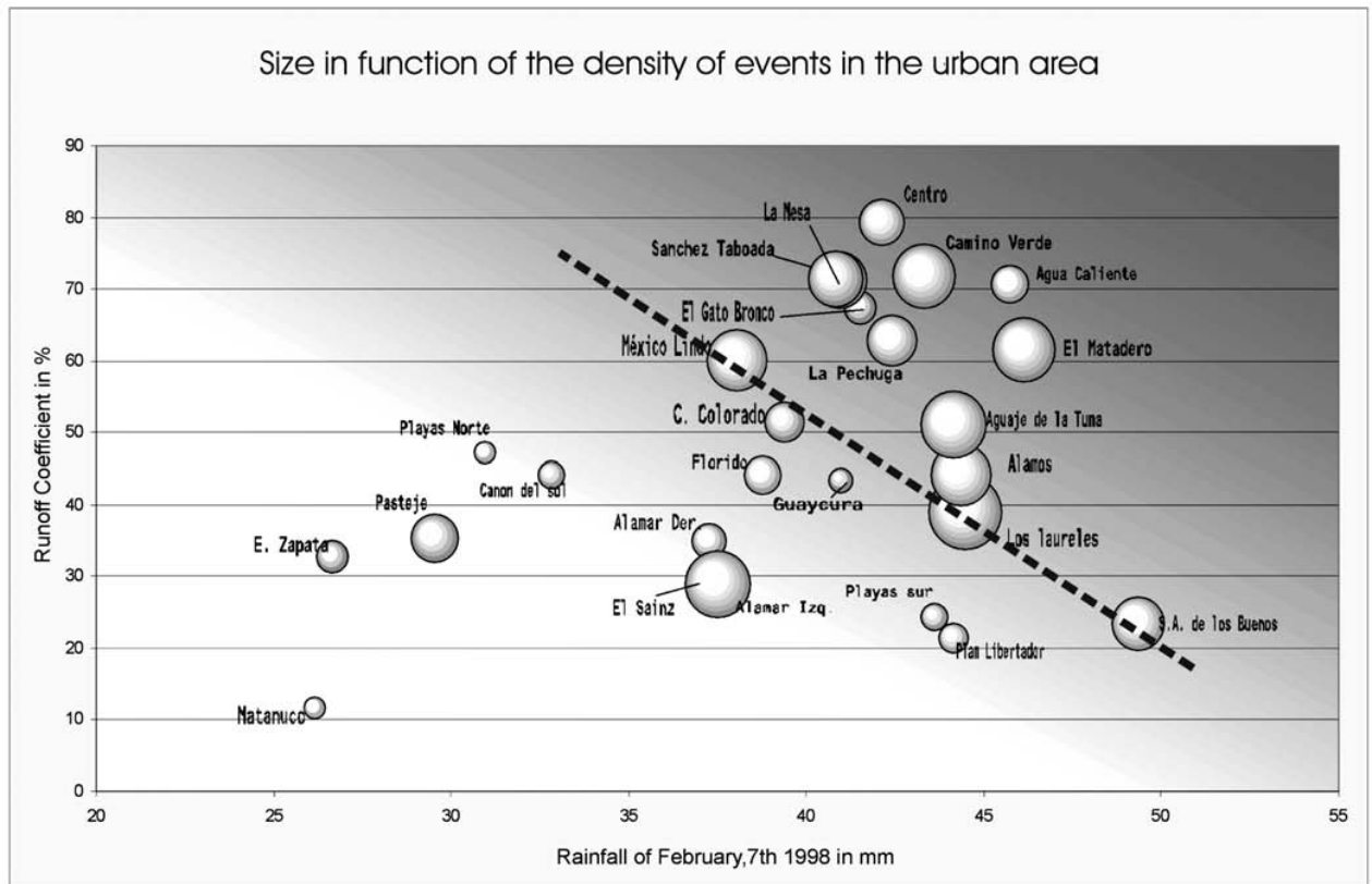
Fig. 11. Determination of thresholds of hazardous events.
