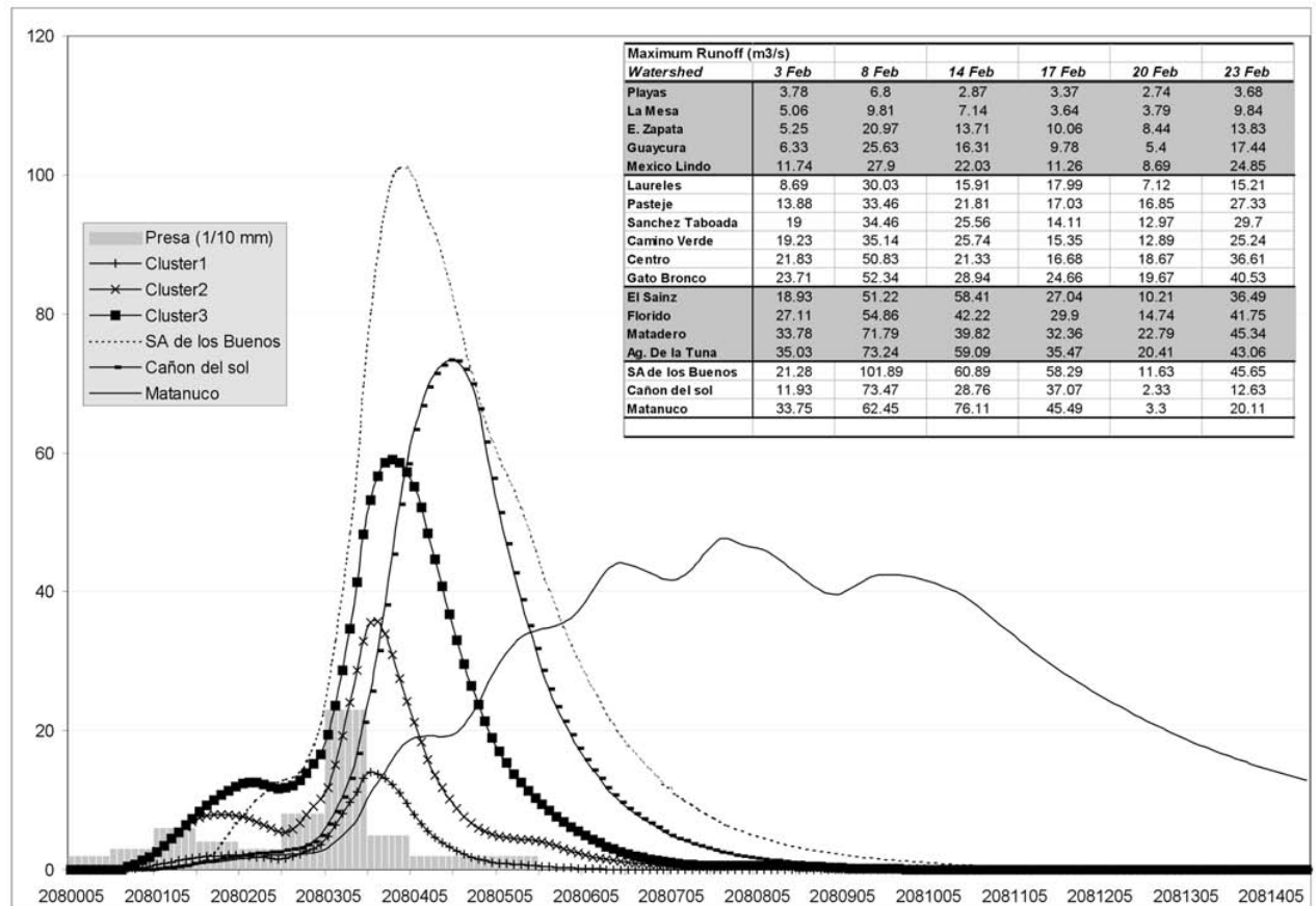
Fig. 10. Synthetic hydrograms from automatic cluster classification.
