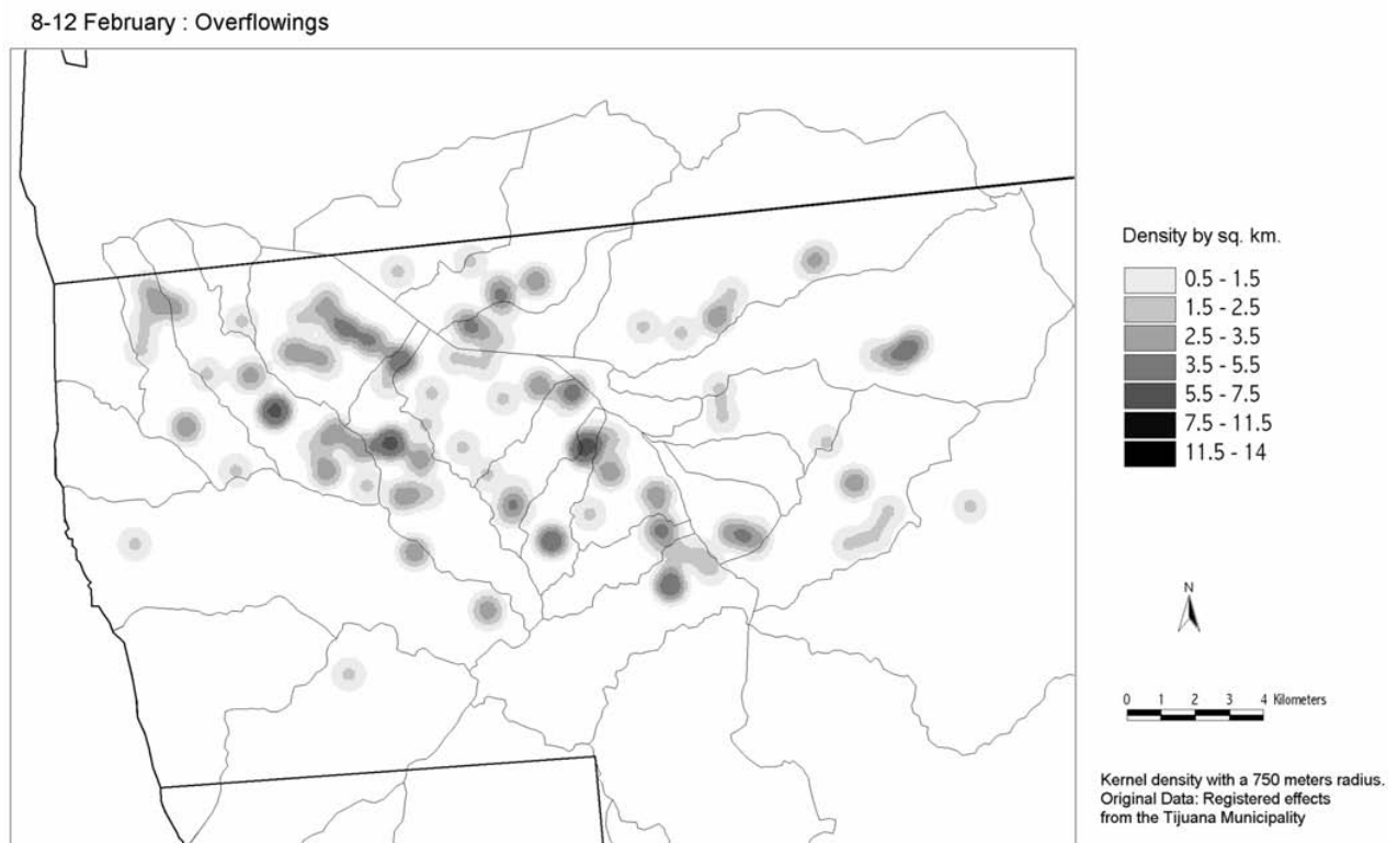
Fig. 5. Overflows between 8 and 12 February, 1998.
