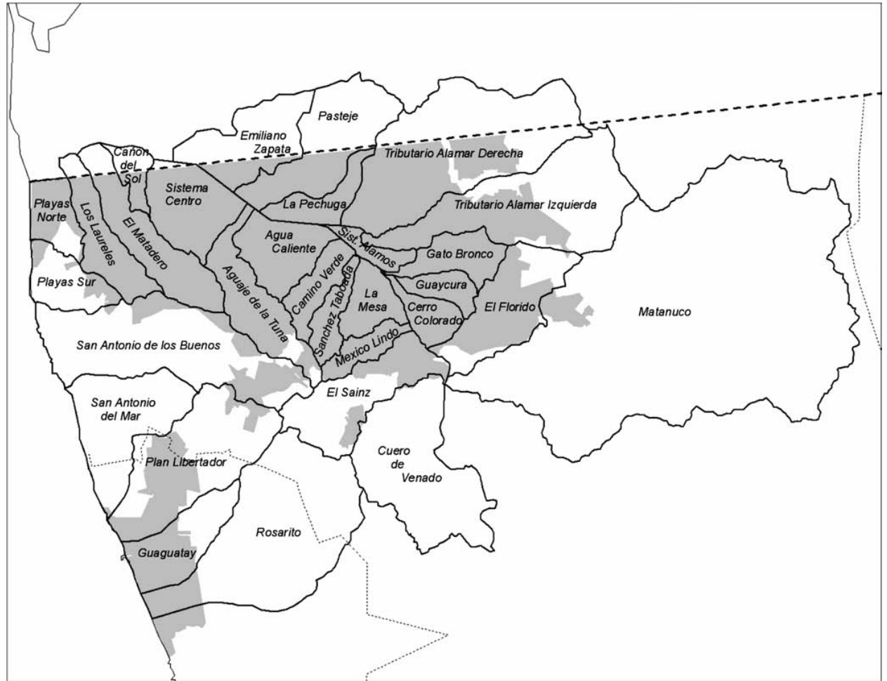
Fig. 1. Location of the Tijuana watersheds.
