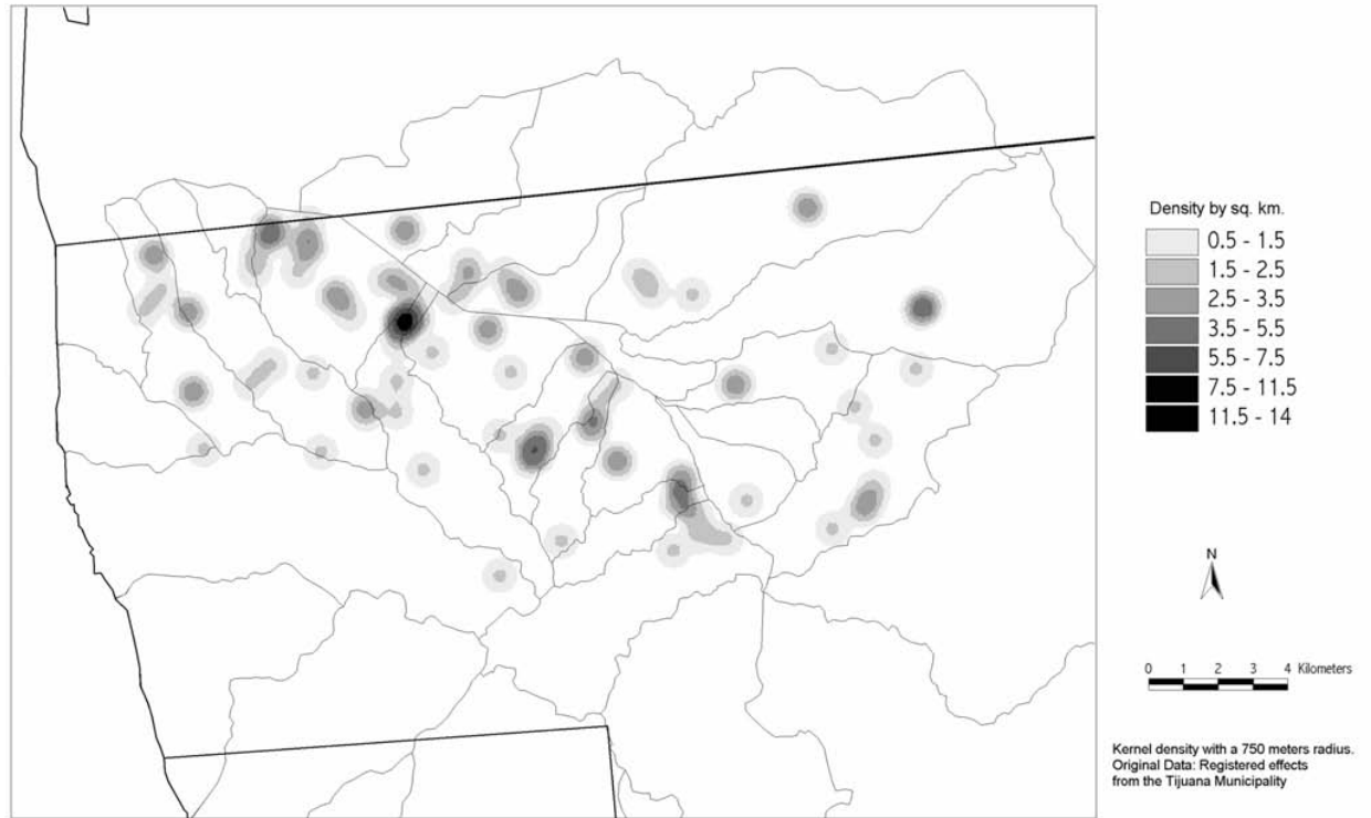
Fig. 6. Events of alluvial deposition between 8 and 12 February, 1998.
