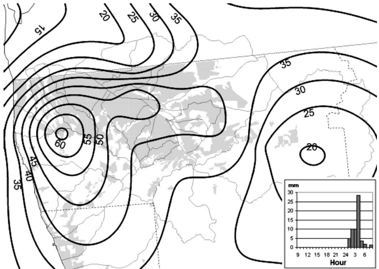
Fig. 4. Rainfall distribution on February 7, 1998.
