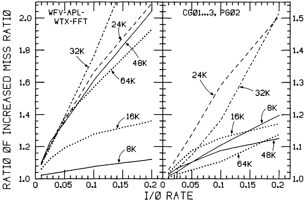
Figure 32. Miss ratio versus I/O rate for variety of memory capacities.
